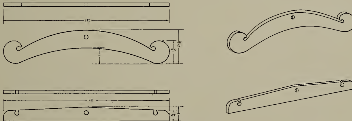
Fig. 41—Heddle Horses
