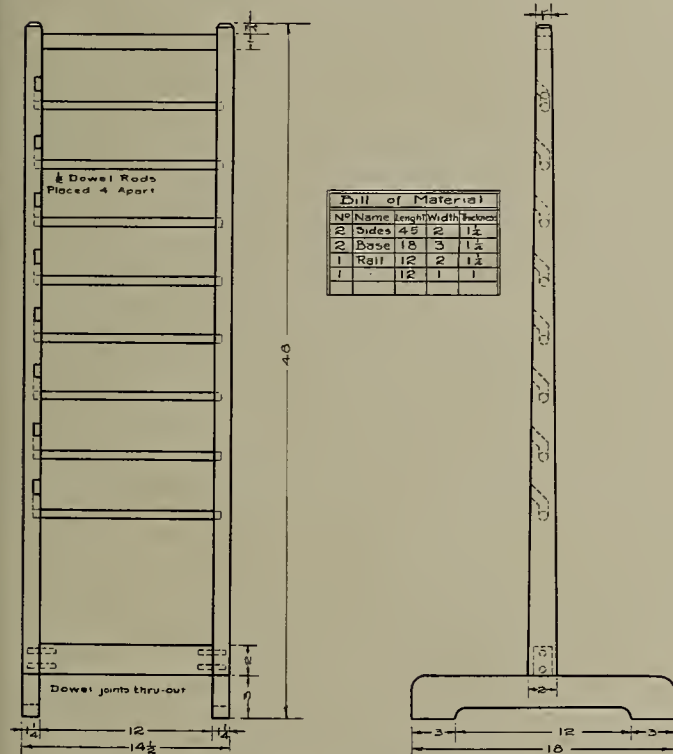
2 Fig. 9—Working Drawing of Spool Rack
