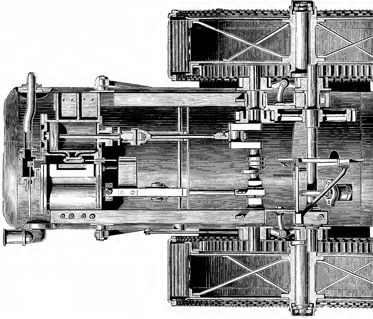
ROBEY'S ROAD STEAMER, 1870 (Sectional View).
