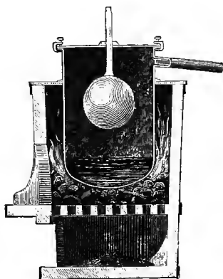
FIG. 53.—Deville and Troost's apparatus for determining the vapour densities, according to Dumas' method, of substances which boil at high temperatures. A porcelain globe containing the substance whose vapour density is to be determined is heated in the vapour of mercury ( 350^{\circ} ), sulphur ( 410^{\circ} ), cadmium ( 850^{\circ} ), or zinc ( 1,040^{\circ} ). The globe is sealed up in an oxyhydrogen flame.
