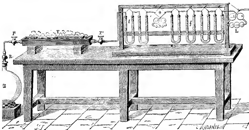
FIG. 38.—Dumas and Boussingault's apparatus for the analysis of air by weight. The globe B contains 10-15 litres. The air is first pumped out of it, and it is weighed empty. The tube T connected with it is filled with copper, and is weighed empty of air. It is heated in a charcoal furnace. When the copper has become red-hot, the stopcock r (near R) is slightly opened, and the air passes through the vessels L, containing a solution of potash, r , containing solutions and pieces of caustic potash, which remove the carbonic anhydride from the air, and then through o and t , containing sulphuric acid (which has been previously boiled to expel dissolved air) and pumice-stone, which removes the moisture from the air. The pure air then gives up its oxygen to the copper in T. When the air passes into T the stopcock R of the globe B is opened, and it becomes filled with nitrogen. When the air ceases to flow in, the stopcocks are closed, and the globe B and tube T weighed. The nitrogen is then pumped out of the tube and it is weighed again. The increase in weight of the tube shows the amount of oxygen, and the difference of the second and third weighings of the tube, with the increase in weight of the globe, gives the weight of the nitrogen.
