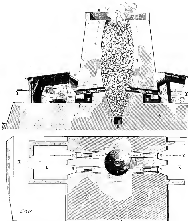
FIG. 78.—Continually-acting kiln for burning lime. The lime is charged from above and calcined by four lateral grates, R, M. D, fire-bars. B, space for withdrawing the burnt lime. K, stokehouse. M, fire grate. Q, R, under-grate.
