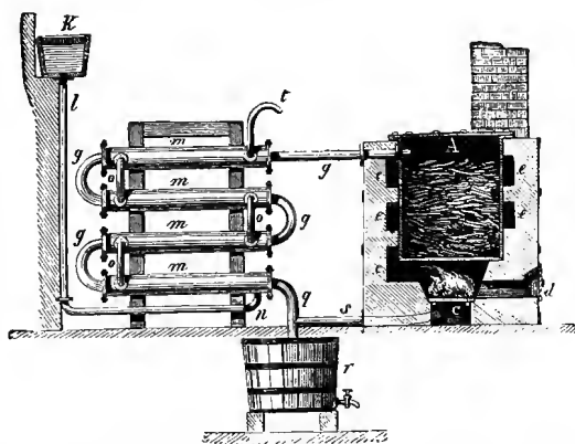
FIG. 57.—Apparatus for the dry distillation of wood. The retort a containing the wood is heated by the fires cc . The steam and volatile products of distillation pass along the tube g through the condenser m , where they are condensed. The form, distribution, and dimensions of the apparatus vary.
