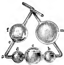
FIG. 39.—Apparatus for the absorption and washing of gases, known as Liebig's bulbs. The gas enters m , passes on the absorptive liquid, and passes from m into b , c , d , and e consecutively, and escapes through f .
