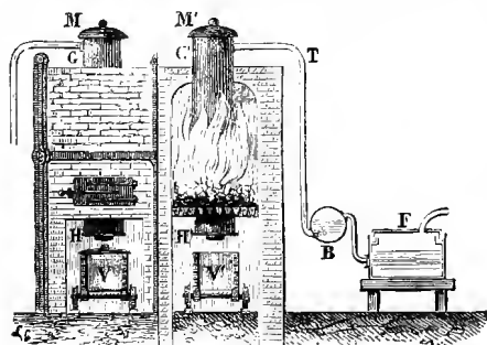
FIG. 42.—The dry distillation of bones on a large scale. The bones are heated in the vertical cylinders C (about 1\frac{1}{2} metre high and 30 centimetres in diameter). The products of distillation pass through the tubes T, into the condenser B, and receiver F. When the distillation is completed the trap H is opened, and the burnt bones are loaded into trucks V. The roof M is then opened, and the cylinders are charged with a fresh quantity of bones. The ammonia water is preserved, and goes to the preparation of ammoniacal salts, as described in the following drawing.
