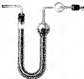
FIG. 41.—Tube for the absorption of carbonic acid. A plug of cotton wool is placed in the bulb to prevent the powder of soda-lime being carried off by the gas. The tube contains soda-lime and chloride of calcium.
