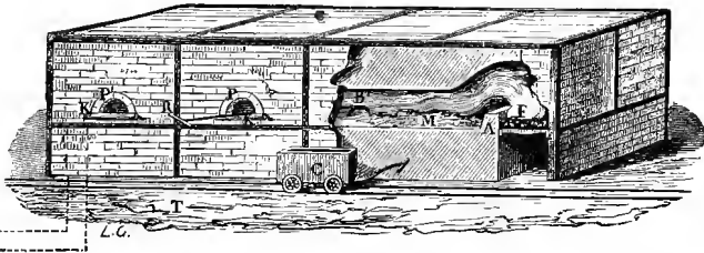
FIG. 68.—Reverberatory furnace for the manufacture of sodium carbonate. F, grate. A, bridge. M, hearth for the ultimate calcination of the mixture of sodium sulphate, coal, and calcium carbonate, which is charged from above into the part of the furnace furthest removed from the fire F. P, P, doors for stirring and bringing the mass towards the grate F by means of stirrers R. At the end of the operation the semifused mass is charged into trucks C.
