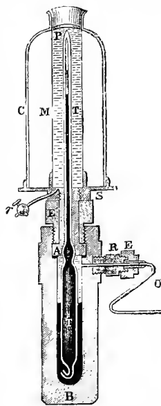
FIG. 25.—Cailletet's apparatus for liquefying gases.
