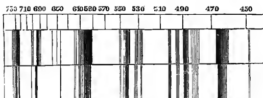
FIG. 73.—Absorption spectrum (Lecoq de Boisbandran) of salts of didymium in concentrated and dilute solutions.
