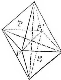
FIG. 11.—Triclinic pyramid.
