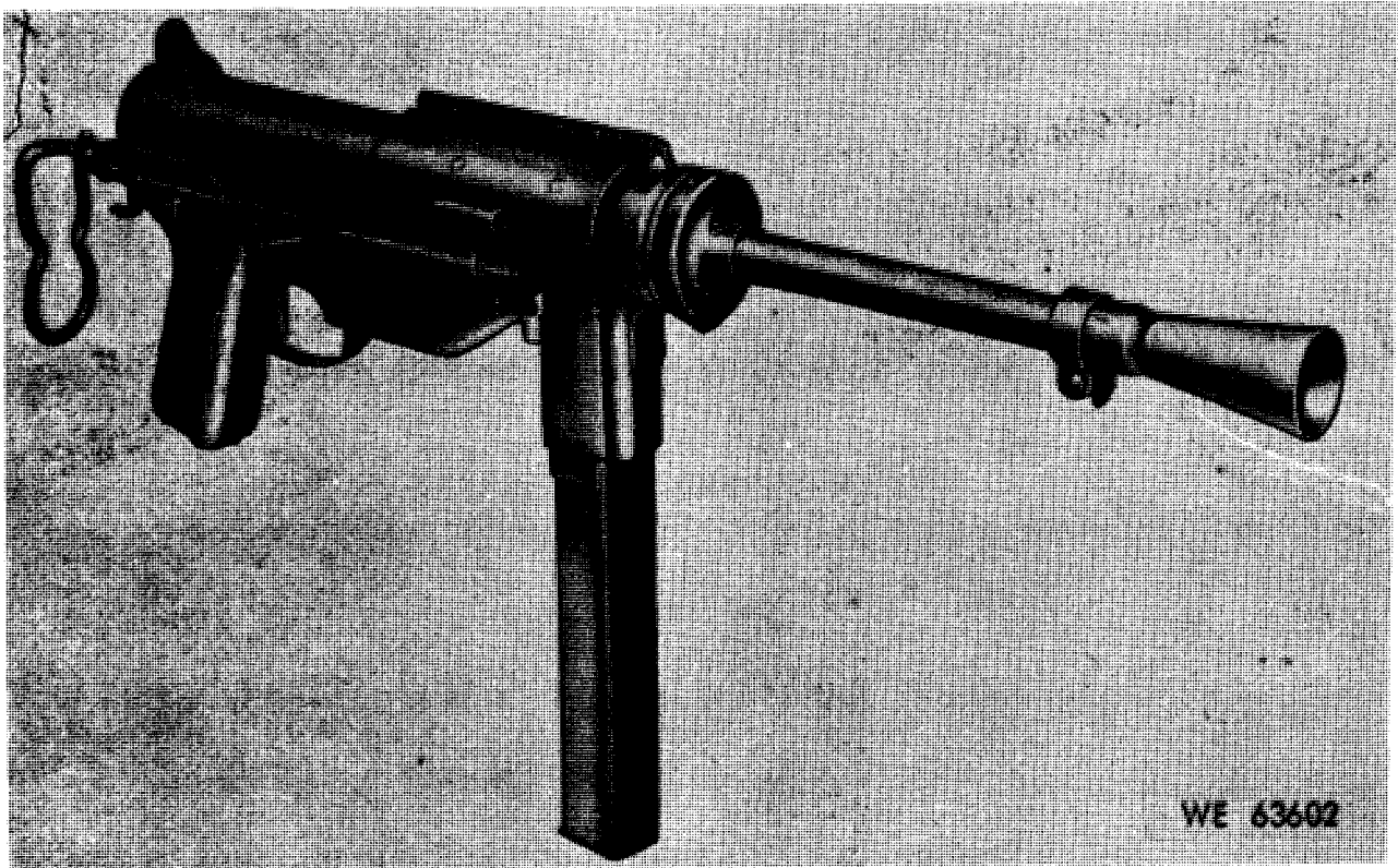
Figure 1-2 Caliber .45 Submachine Gun M3A1 w/Flash Hider Assembly, M9-right front view.
