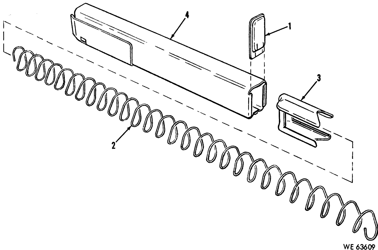
Figure 3-3. Magazine-exploded view.
