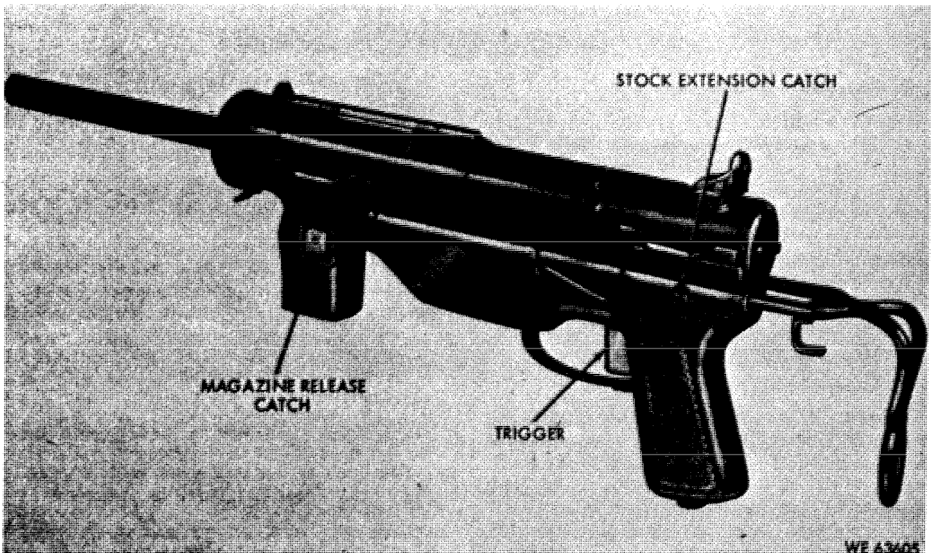
Figure 2-1. Controls.
