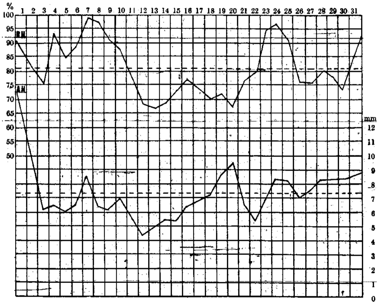
The March of Absolute and Relative Humidity in the Month of March, 1928
