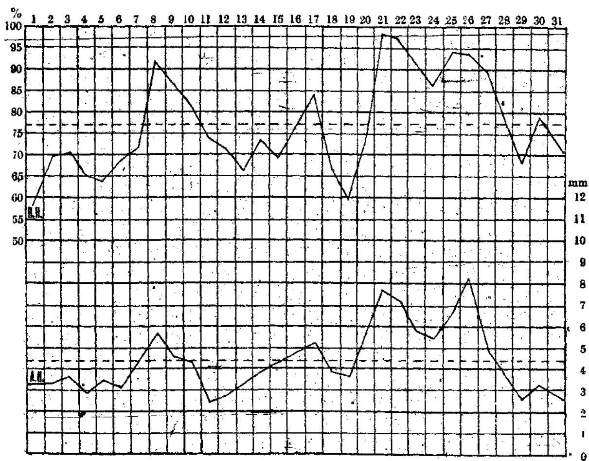
中華民國十七年一月份絕對濕度與相對濕度變遷圖 The March of Absolute and Relative Humidity in the Month of January, 1928
