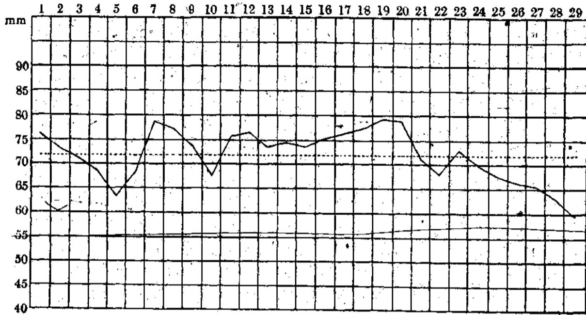
中華民國十七年二月份氣壓變遷圖 (700 mm+ ) The March of Barometric Pressure in the Month of February, 1928 (700 mm+ )
