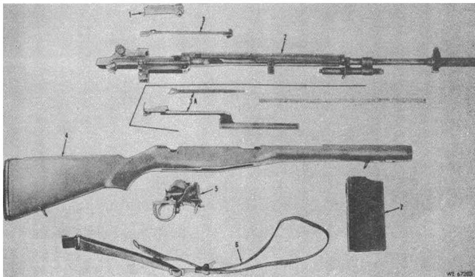
Figure 3-1. Weapon field stripped (M14).
