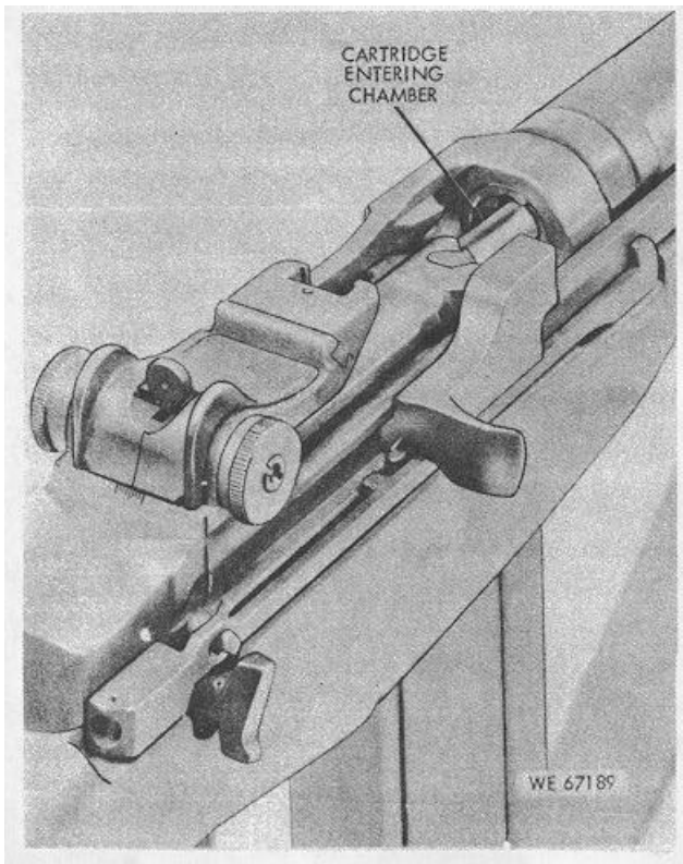
Figure 2-6. Chambering the cartridge.
