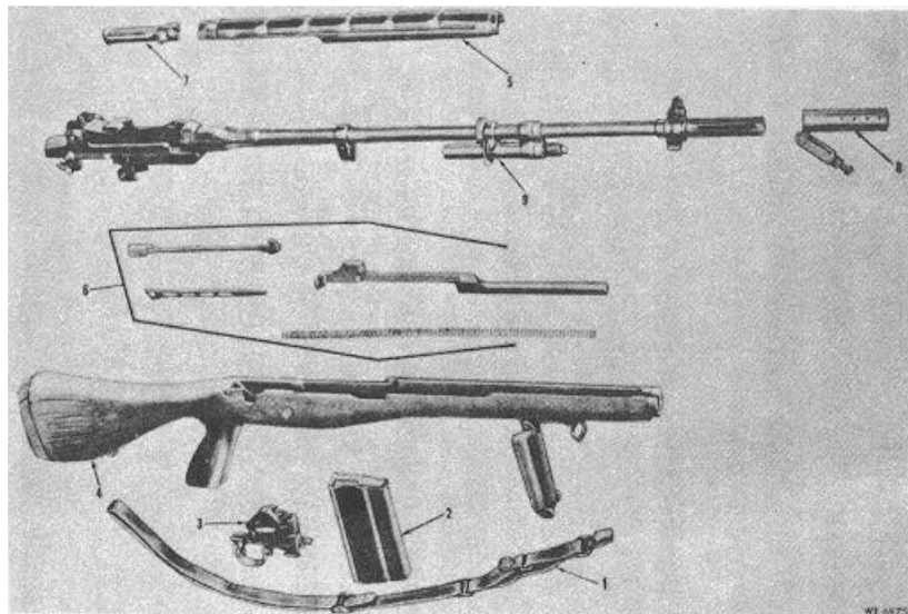
Figure 3-2. Weapon field stripped (M14A1).
