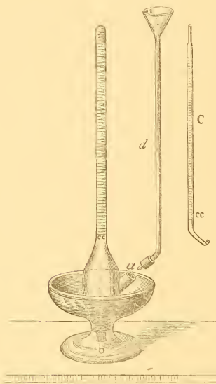
Marshall's Apparatus.
