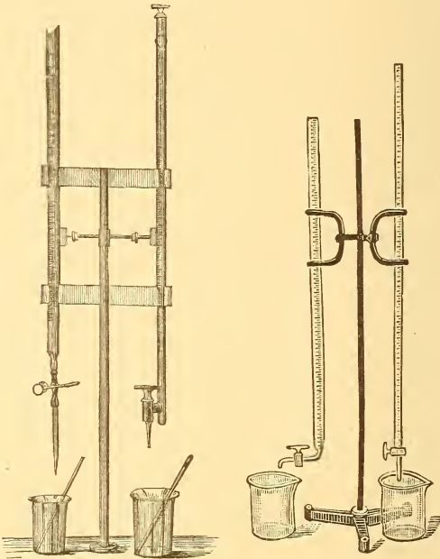
Varieties of Burette Stand.
