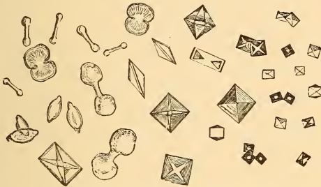
Oxalate of Lime Crystals. (After Harley.)
