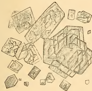
Crystals of Nitrate of Urea. (After Beale.)
