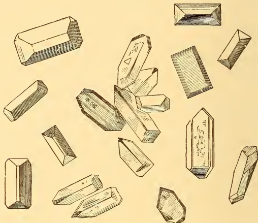
Forms of Crystals of the Ammonio-magnesian Phosphate. (After Harley.)
