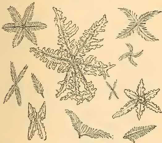
Stellate and Feathery Crystals of Triple Phosphate. (After Harley.)
