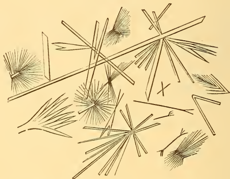
Crystals of Calcium Sulphate. (From Van Nüys.)
