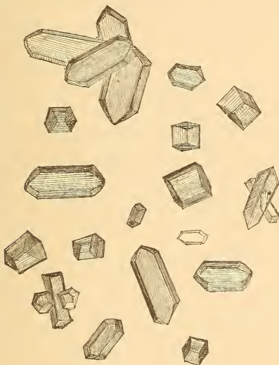
Other Unusual Forms of Uric Acid, not unlike Crystals of the Triple Phosphate of Ammonium and Magnesium. \times 150 .
