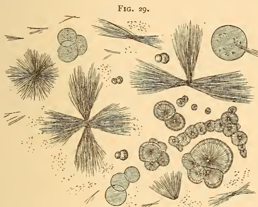
Leucin Spheres and Tyrosin Needles.
