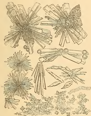
Prismatic Crystals of Sodium Urate, Spherules of Ammonium Urate, and Amorphous Urates, with Octohedral Crystals of Oxalate of Lime. (Ranke.)
