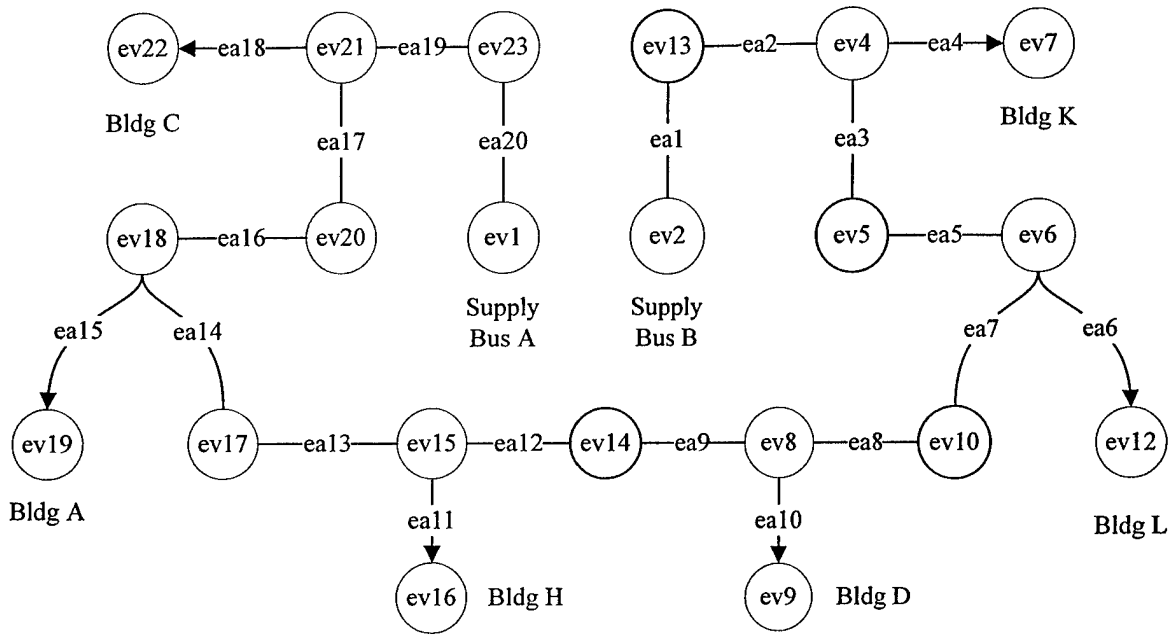
Figure III.9 Electrical distribution network digraph (loop one)
