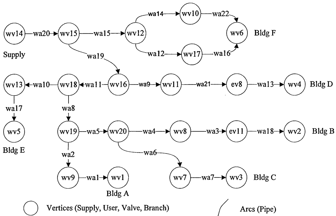
Figure III.7 – Water distribution network digraph
