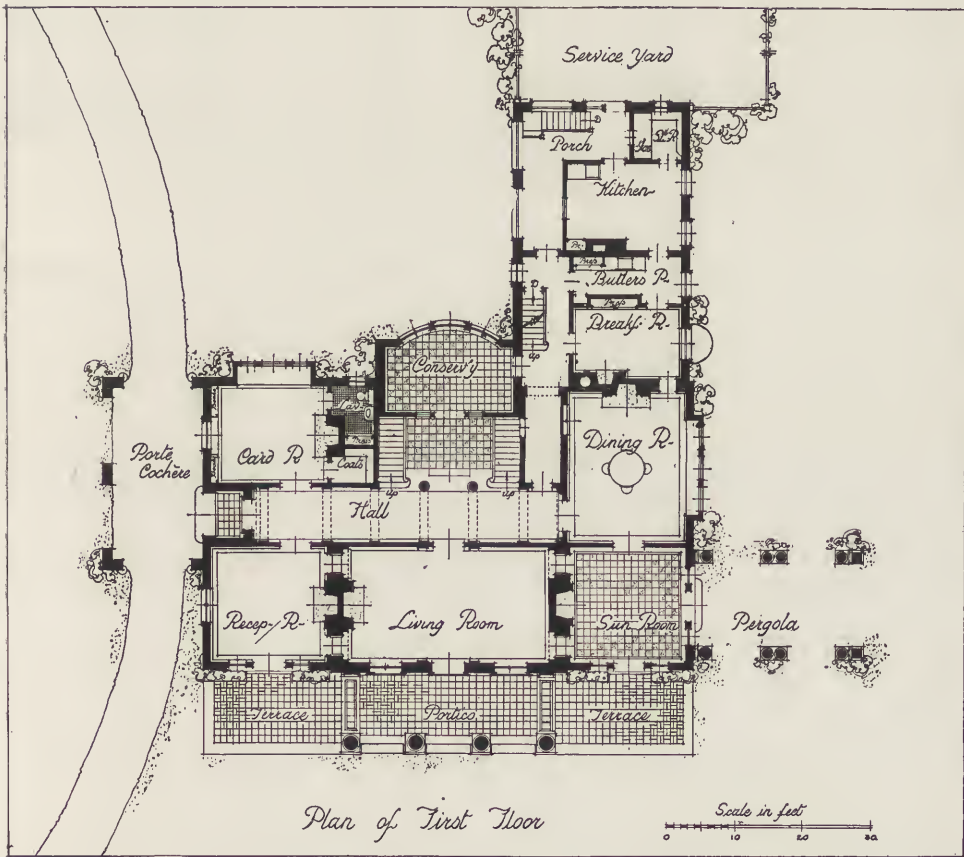
FIG. 73. FIRST FLOOR PLAN—RESIDENCE OF JOHN A. HITCHCOCK, ESQ., NASHVILLE, TENN. Dougherty & Gardner, Architects.
