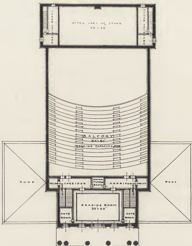
SECOND FLOOR PLAN SCALE \frac{1}{4}'' = 1'-0''
