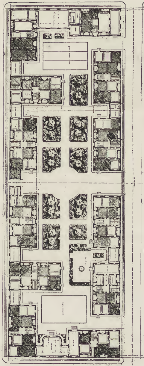
GROUND FLOOR AND SECOND FLOOR PLAN OF ROTTOLE HOUSING DEVELOPMENT, MILAN, BY THE UMANITARIA SOCIETY.
