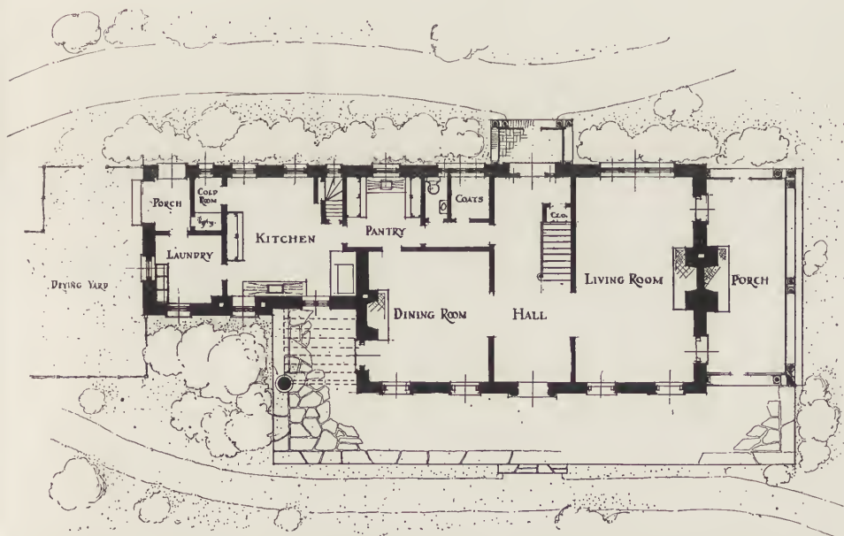
FIG. 68. FIRST FLOOR PLAN—RESIDENCE OF C. E. MCINNES, ESQ., RYDAL, PA. Duhring, Okie & Ziegler, Architects.
