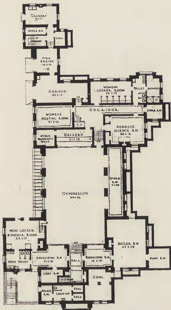
BASEMENT PLAN SCALE 3/8" = 1'-0"
