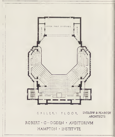
FLOOR PLANS—OGDEN HALL, HAMPTON NORMAL AND AGRICULTURAL INSTITUTE, HAMPTON, VA.
