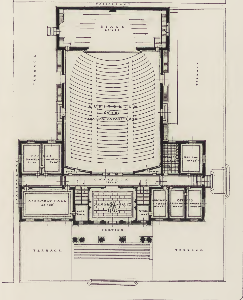
MAIN FLOOR PLAN SCALE 1" = 10'
