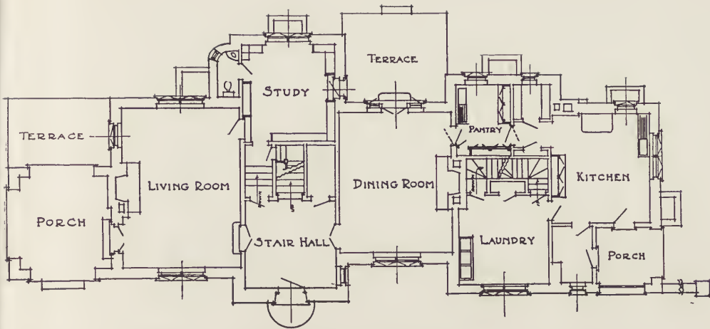
FIG. 71. FIRST FLOOR PLAN—RESIDENCE OF DR. EDWARD B. KRUMBHAAR, WHITEMARSH VALLEY, PA. Arthur H. Brockie, Architect.
