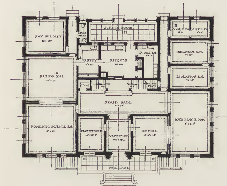
FIRST FLOOR PLAN SCALE \frac{1}{8}''=1' SANTA BARBARA COUNTY DETENTION HOME SANTA BARBARA CALIFORNIA
