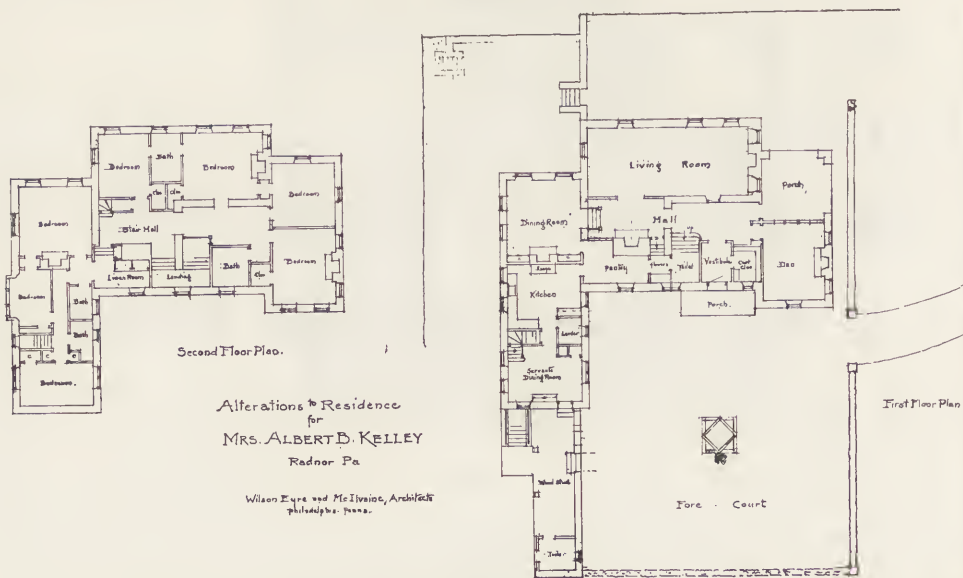
FIG. 72. FIRST AND SECOND FLOOR PLANS—RESIDENCE OF MRS. ALBERT B. KELLEY RADNOR, PA. Wilson Eyre & McIlvaine, Architects.
