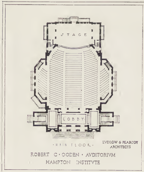
FLOOR PLANS—OGDEN HALL, HAMPTON NORMAL AND AGRICULTURAL INSTITUTE, HAMPTON, VA.
