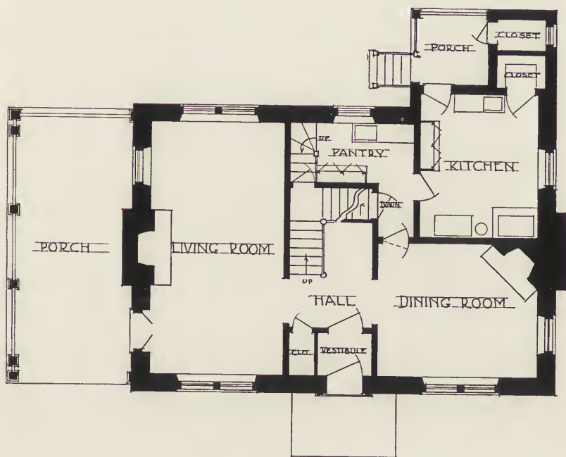
HOUSE AT CHESTNUT HILL —PHILA—
