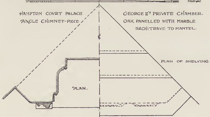
ANGLE CHIMNEYPICE IN GEORGE II'S PRIVATE CHAMBER, HAMPTON COURT PALACE.
