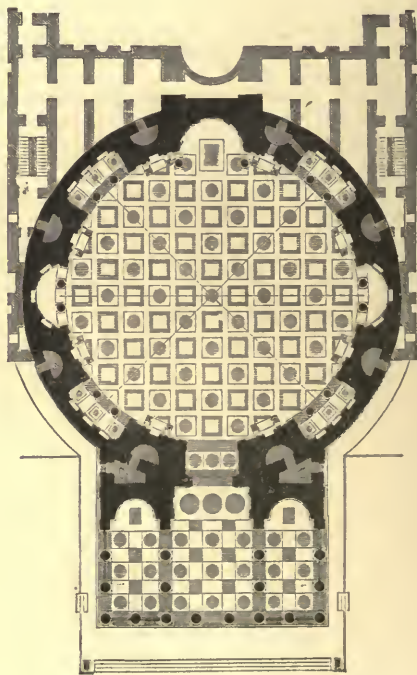
FIG. 135.—THE PANTHEON, ROME. GROUND-PLAN.
