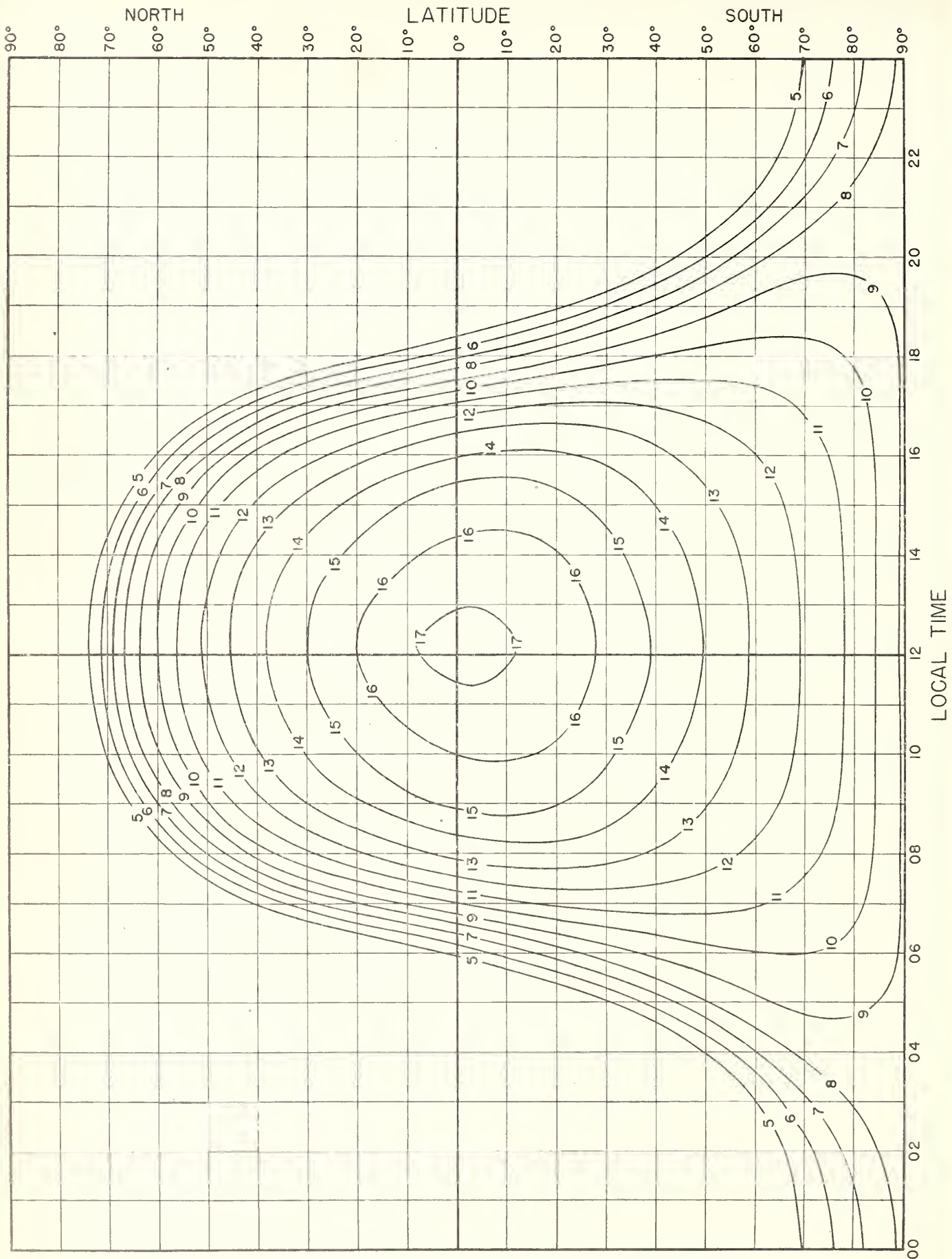
FIG. 7. E-2000-MUF, IN Mc, PREDICTED FOR JANUARY 1955
