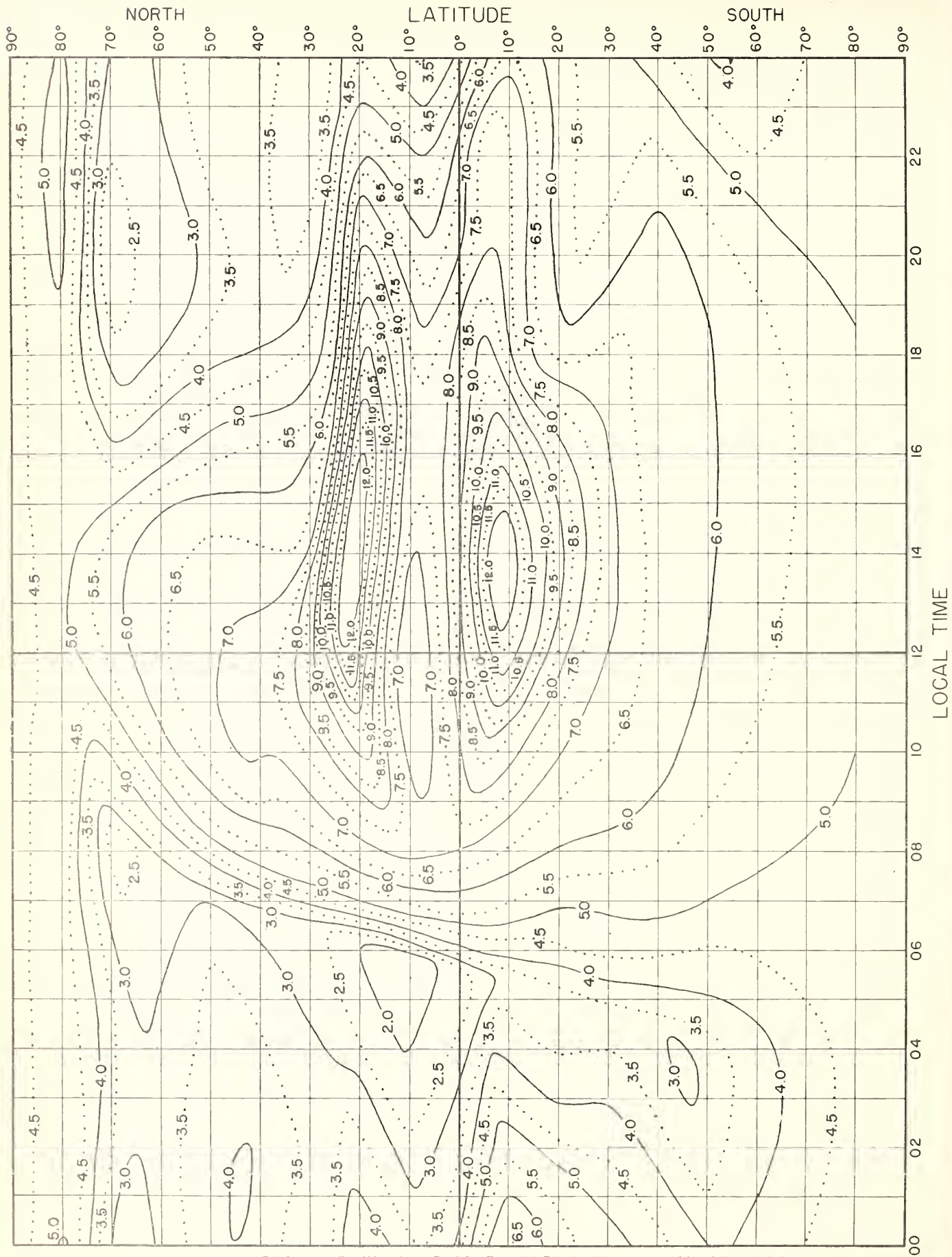
FIG. 5 F2-ZERO-MUF, IN Mc, E ZONE, PREDICTED FOR JANUARY 1955
