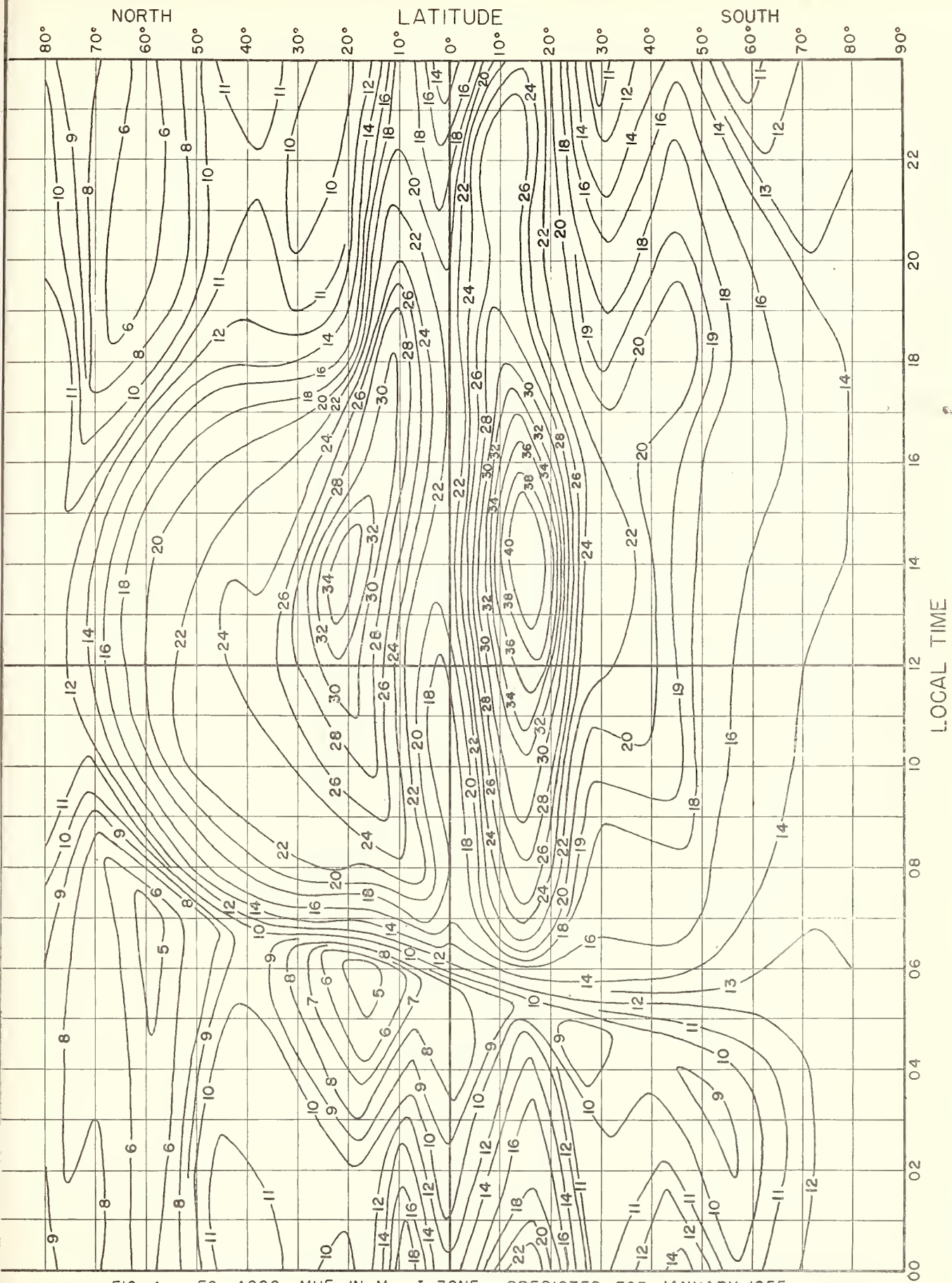
FIG. 4. F2-4000-MUF, IN Mc, I ZONE, PREDICTED FOR JANUARY 1955
