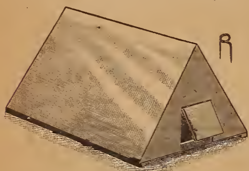
SWINGING DOOR FOR HOG HOUSE
