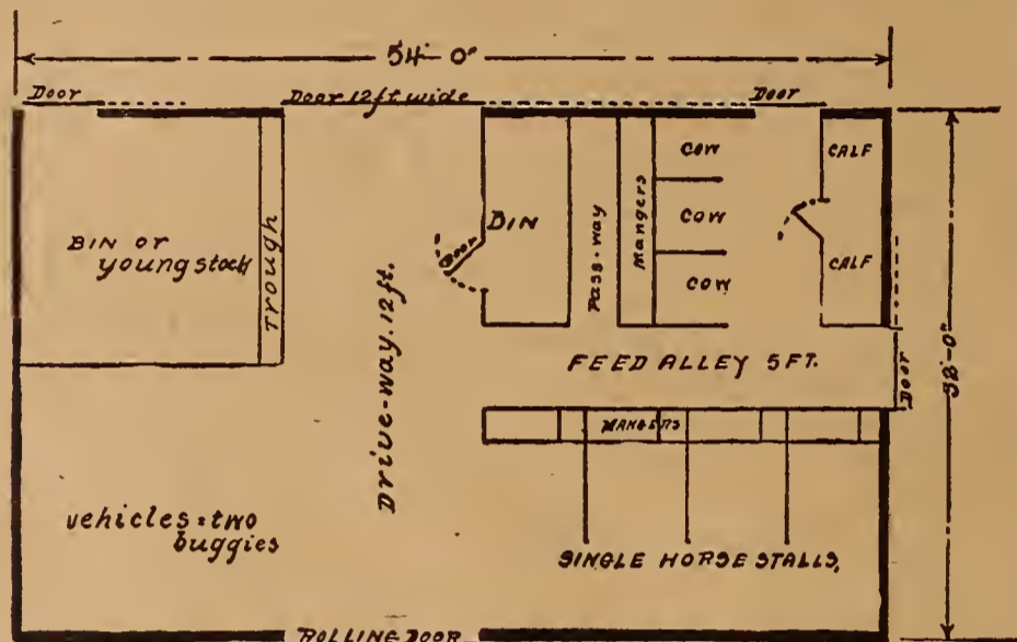
RECTANGULAR BARN 32x54 FT. COMPARED TO A ROUND BARN WITH SAME NO. OF FEET OF WALL TAKING 172 LINEAL FEET
