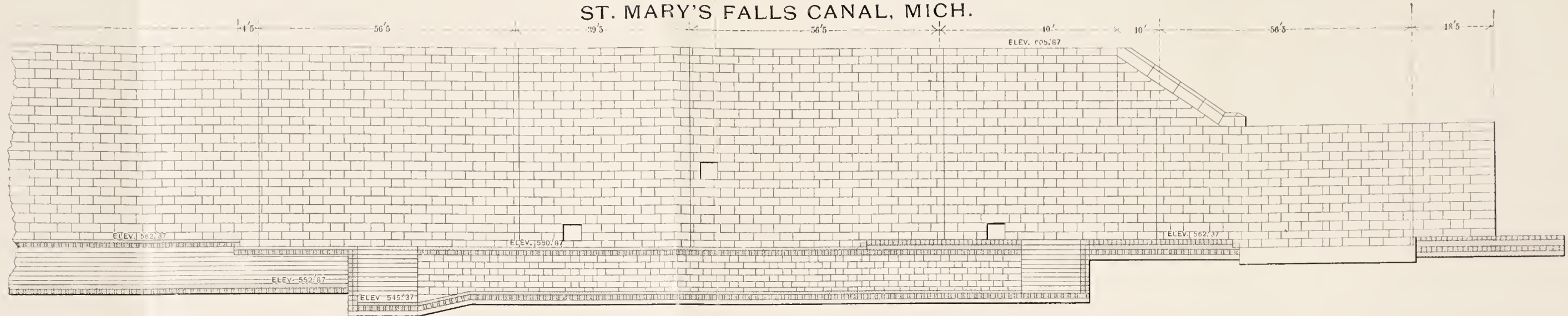
LONGITUDINAL SECTION OF FLOOR AND ELEVATION OF WALL AT EAST END
