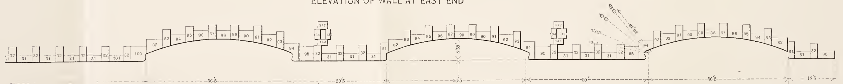
LONGITUDINAL SECTION OF FLOOR AND ELEVATION OF WALL AT EAST END
