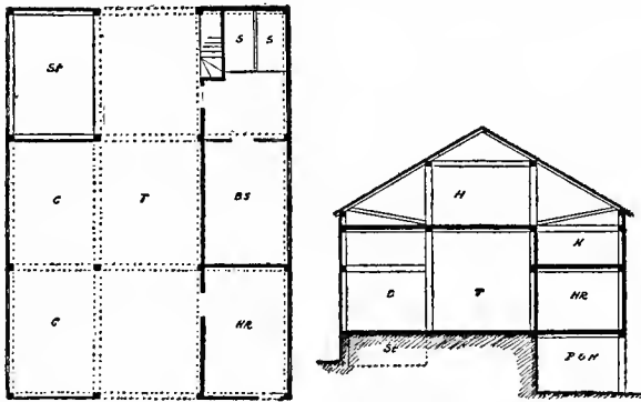
Fig. 17—Plan and section suggestive of the stableizing of the old barn. B S, Box stall; C, Carriage; H, Hay; HR, Harness room; S, Stall; St, Straw bay; T, Threshing-floor; P & H, Poultry & hogs
