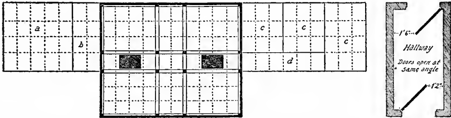
Fig. 5—Showing the narrow hallway with the advantage of the uncentered over the centered door
