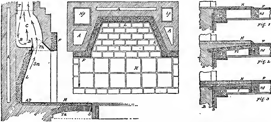
Fig. 11—Sections illustrating the incorporating of a hearth. Fig. 1 shows a hearth laid on the floor (very bad); Fig. 2, an incorporated and raised hearth by aid of flagging; Fig. 3 the incorporated flush hearth by aid of irons. Hd—header; H—hearth; F—flooring; B—brickwork; S—plank studding, Fl—flagstone; T—tire beam; I—tire irons
