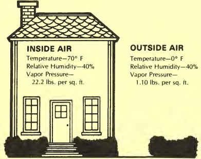
Figure 1. Vapor pressure difference between indoors and outdoors causes the movement of moisture into the walls.
