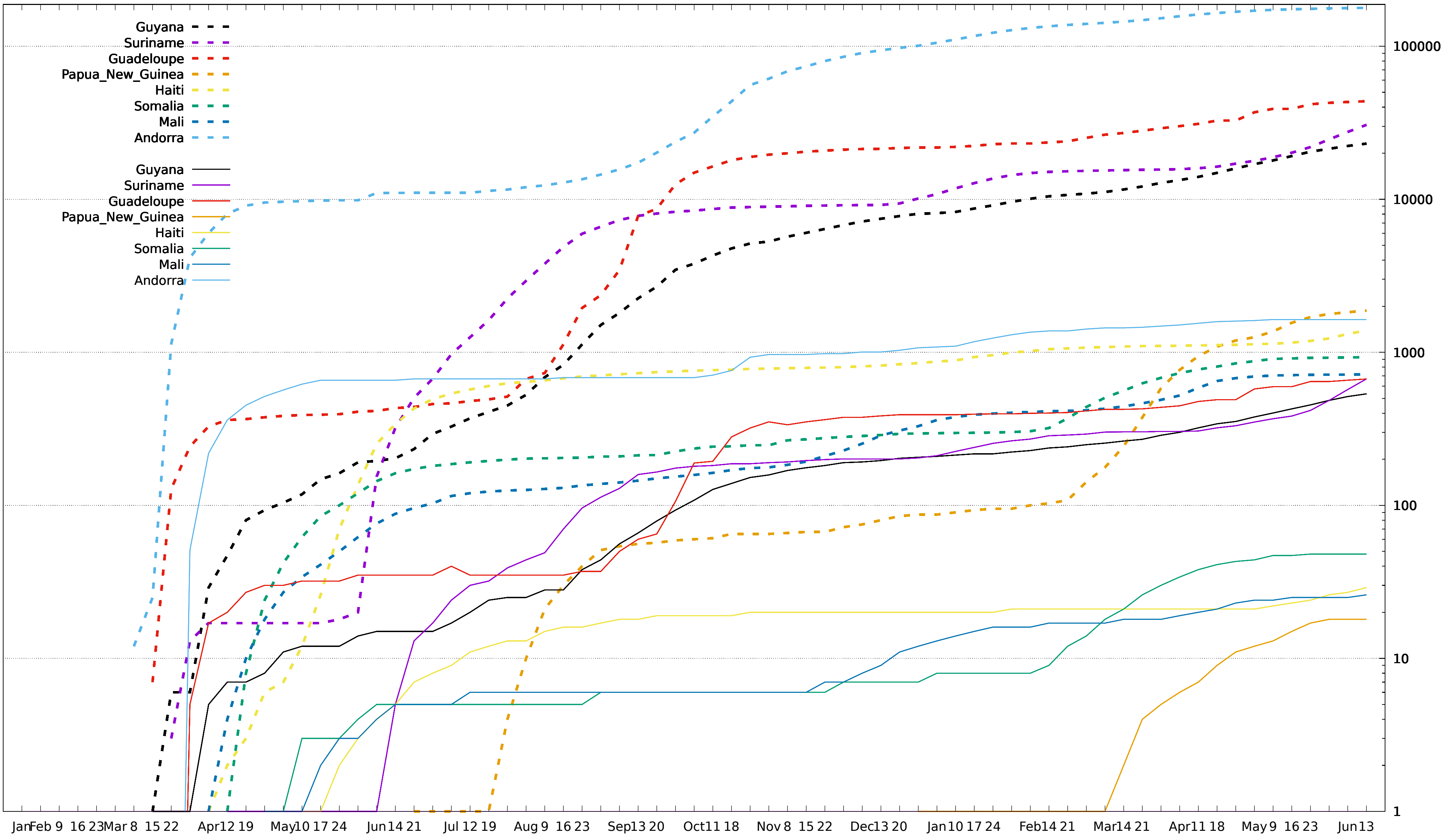
@confirmed,@deaths by count [18]
