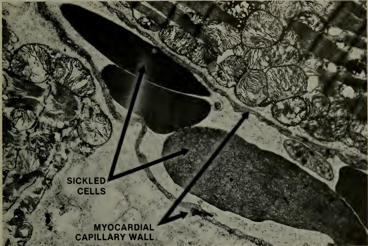
Figure 22. This transmission electron micrograph shows abnormal sickle-shaped red blood cells blocking a small blood vessel, or capillary, in the heart (magnification x 10,000). For comparison, the appearance of a normal circle-shaped red blood cell can be seen in figure 19.
