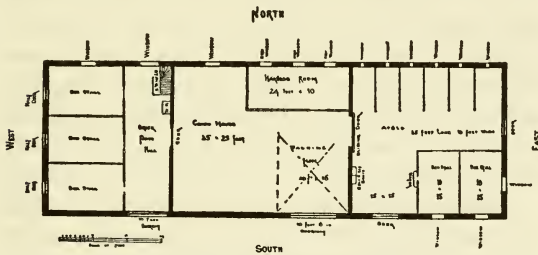
PLATE XV.—STABLE PLAN
