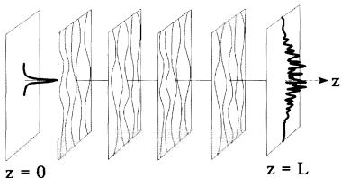
Figure 9 Computer simulation using the split-step method. The source (left) is propagated in steps out to z = L , with phase screens applied at each step.
