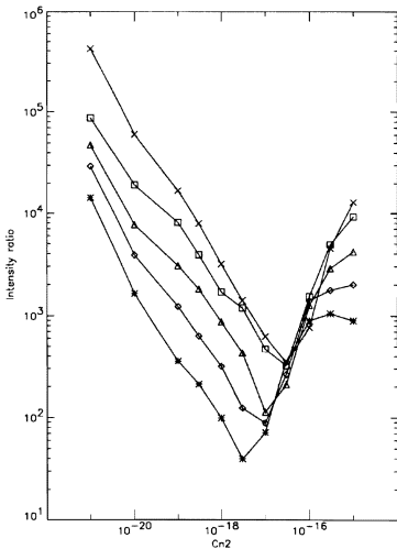
Figure 24 Irradiance ratio versus turbulence strength ( \beta_0^2 = [5 \times 10^{-4}, 5 \times 10^2] ) for grid sizes: 64x64 (asterisks), 128x128 (diamonds), 256x256 (triangles), 512x512 (squares), 1024x1024 (X's).
