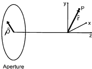
Figure 2 Propagation coordinate system showing relations between the aperture variables and the field variables.
