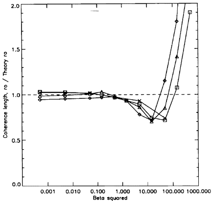
Figure 29 Spherical wave coherence length from simulations versus turbulence strength for grid sizes 128x128 (diamonds), 256x256 (triangles), 512x512 (squares), and 1024x1024 (X's).
