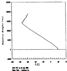
Figure 6 Vertical profile of temperature in the atmosphere.
