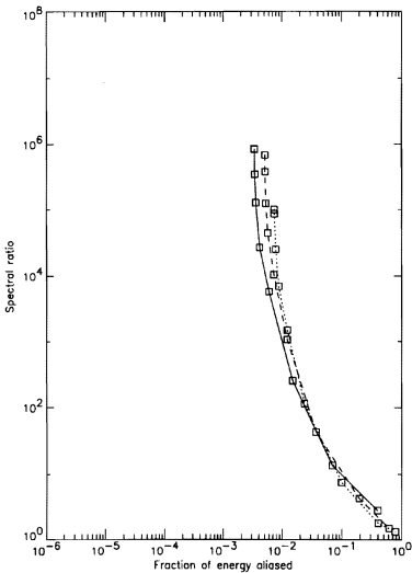
Figure 35 Power spectral density ratio versus fraction of energy aliased for Airy-type source; grid sizes: 64x64 (dotted line), 128x128 (dashed line), 256x256 (solid line).
