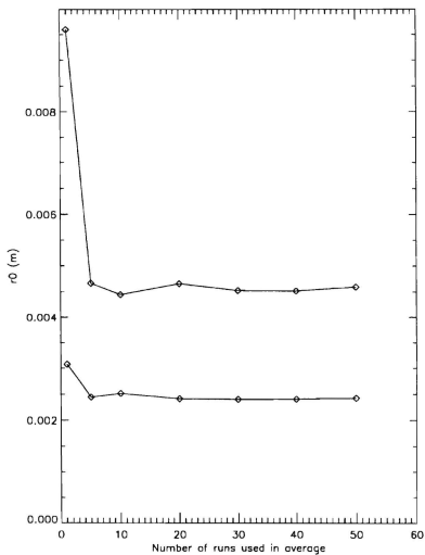
Figure 45 Coherence length as a function of the number of realizations used in the average atmospheric MTF (top: \beta_0^2 = 3 ; bottom: \beta_0^2 = 20 ).
