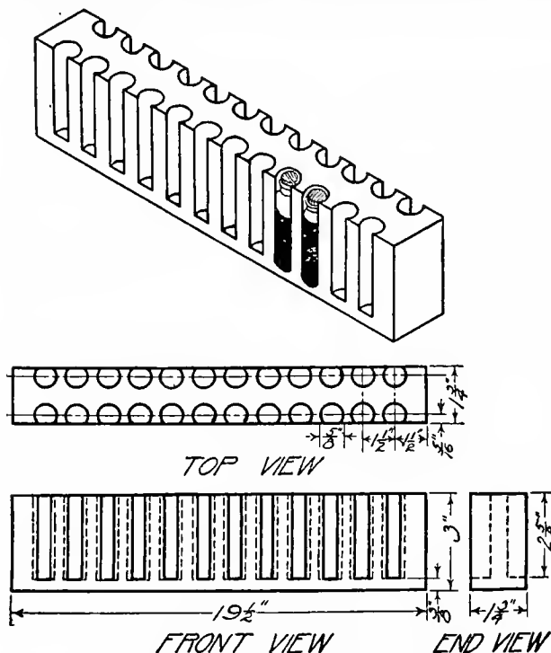
FIG. 76. — Case for storing bottles of seeds.
