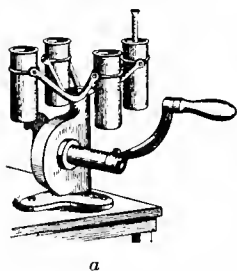
FIG. 149. — A four-bottle hand power tester.
