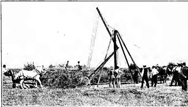
FIG. 60. — A sweep-rake bringing the hay to the stacker.
