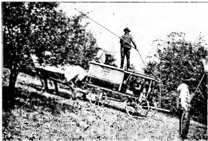
FIG. 103. — Gas-engine sprayer.
