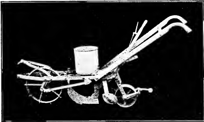
FIG. 208. — One-horse corn-planter.
