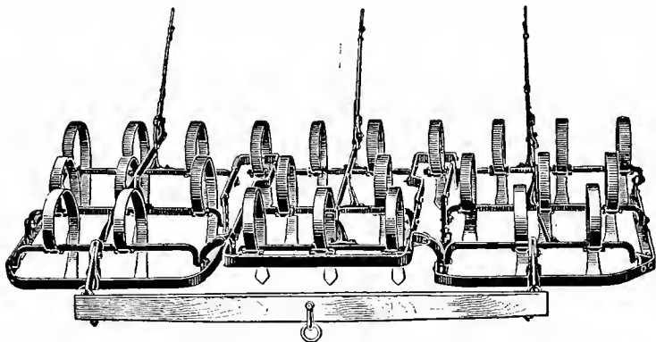
FIG. 201. — Spring-tooth harrow.
