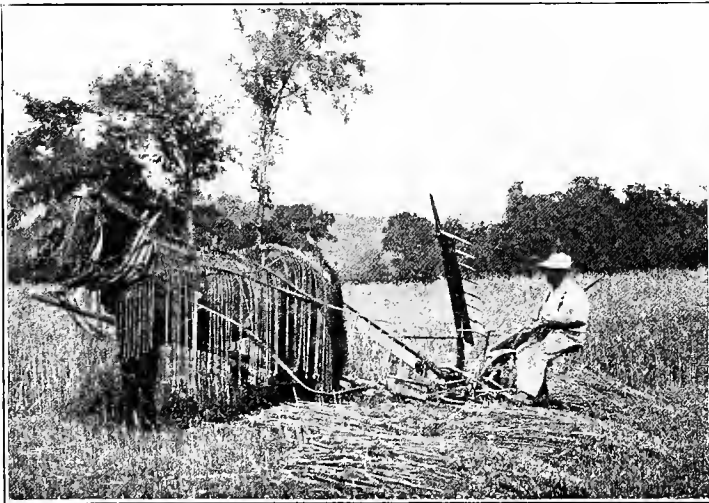
FIG. 51. — Self-rake reaper.
