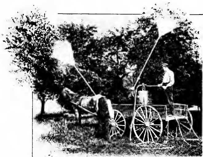
FIG. 104. — Hand-power sprayer.
