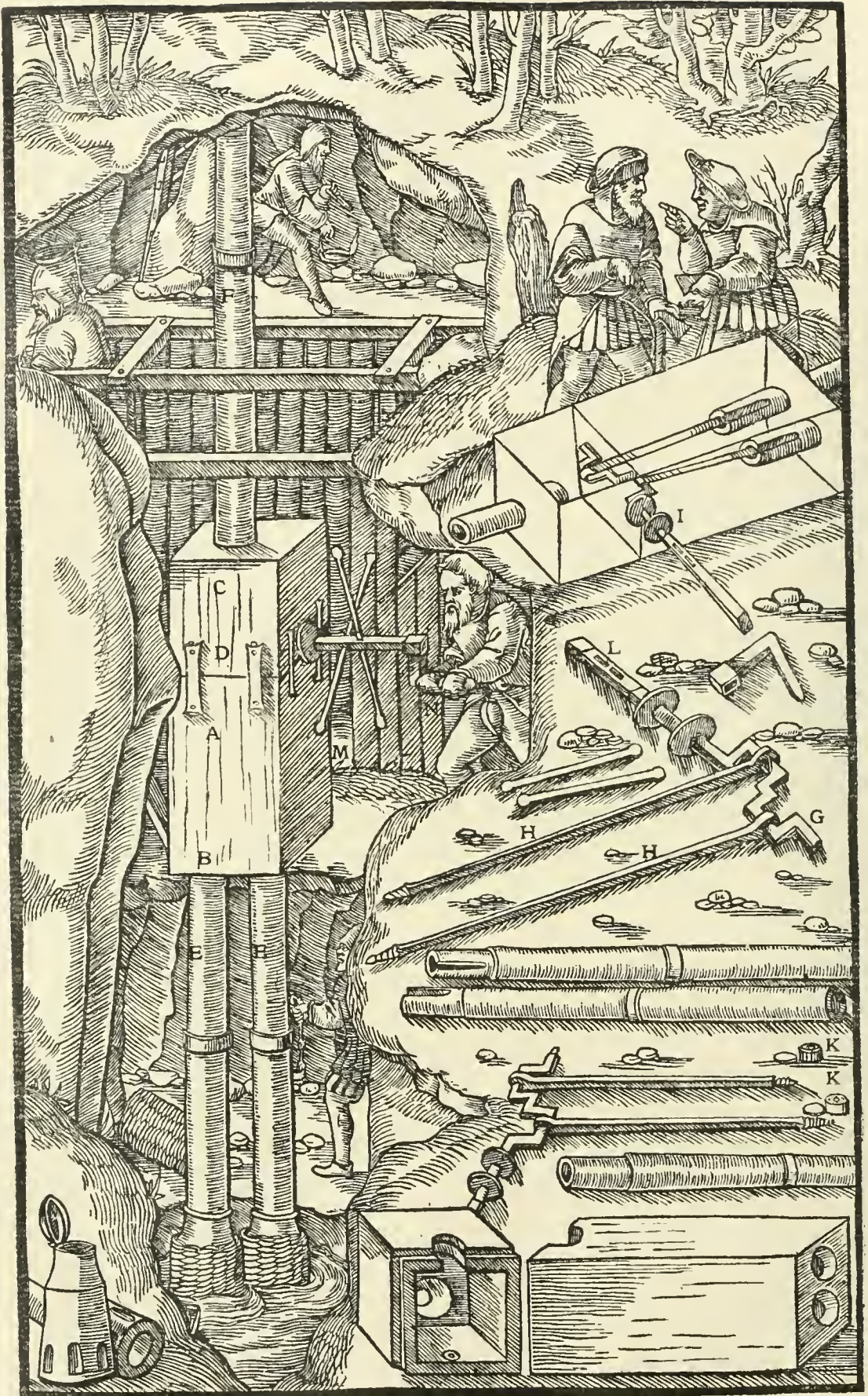
A—BOX B—LOWER PART OF BOX. C—UPPER PART OF SAME. D—CLAMPS. E—PIPES BELOW THE BOX. F—COLUMN PIPE FIXED ABOVE THE BOX. G—IRON AXLE. H—PISTON-RODS. I—WASHERS TO PROTECT THE BEARINGS. K—LEATHERS. L—EYES IN THE AXLE. M—RODS WHOSE ENDS ARE WEIGHTED WITH LUMPS OF LEAD. N—CRANK.
