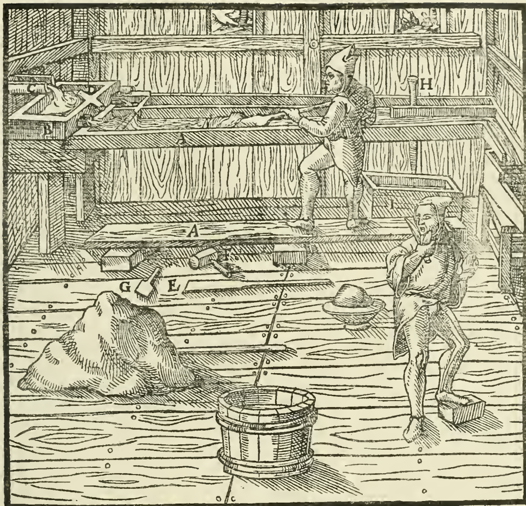
A—STRAKES. B—TANK. C—LAUNDER. D—PLUG. E—WOODEN SHOVEL. F—WOODEN MALLET. G—WOODEN SHOVEL WITH SHORT HANDLE. H—THE PLUG IN THE STRAKE. I—TANK PLACED UNDER THE PLUG.
