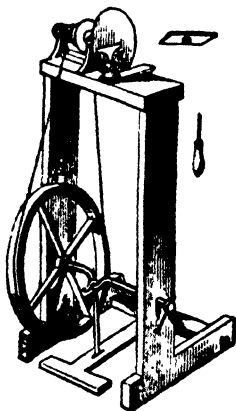
Fig 143b — Small Lathe for polishing.
