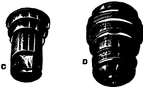
FIG. 35.—Wenham's Binocular Objective.
