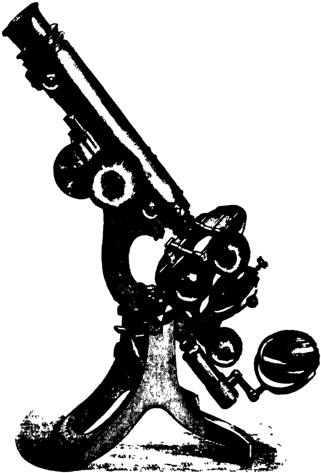
FIG. 62. -- Swift's New Challenge Microscope
