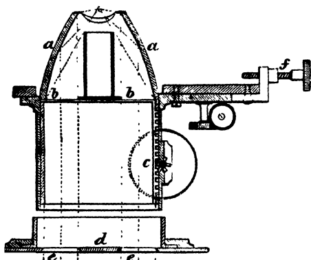
FIG. 106.—A sectional view of Wenham's Parabolic Illuminator.
