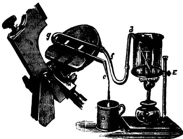
FIG. 28.—Bartley's Warm Stage.
