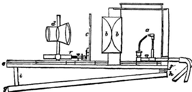
FIG. 95a.— Draper's Microphotographic Apparatus.
