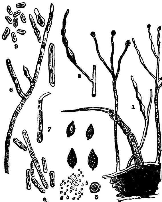
Fig. 160.—Fungoid growths.
