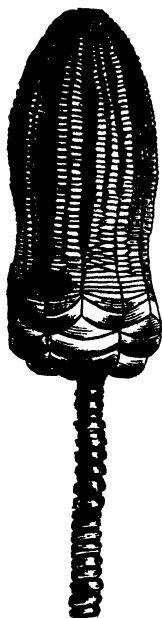
Fig. 241.— Encrinurus , Sea-holy.
