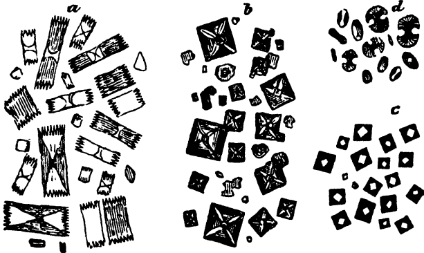
Fig. 89. — Urinary Salts.
