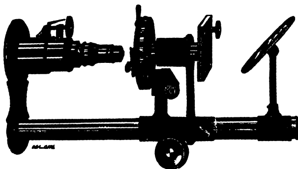
Fig. 95.—Highley's Photo-micrographic A-arrangement.
