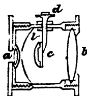
Fig. 2. Lieberkuhn's Microscope.
