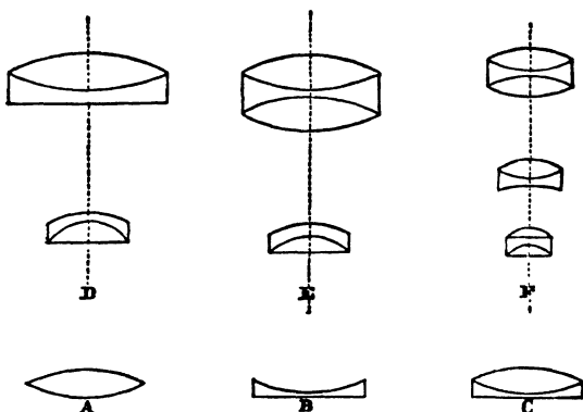
FIG. 37.—Forms of Object-glasses.
