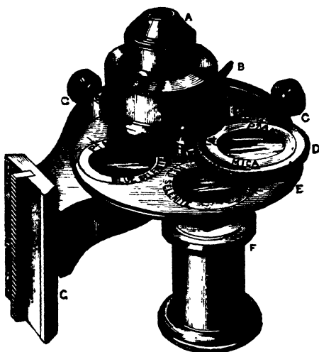
FIG. 113 — Swift's Achromatic Condenser.
