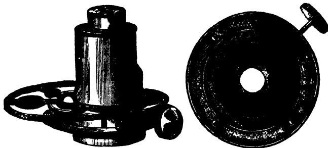
FIG. 115.—Collins's Webster's Universal Condenser.
