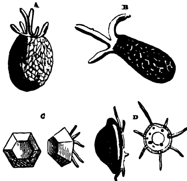
Fig. 205.—Simple Rhizopods.
