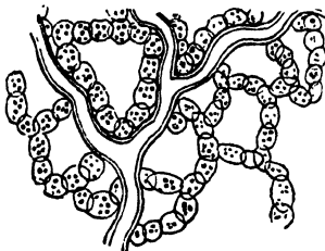
Fig. 178. — Lactiferous tissue.
