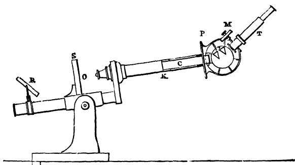
Fig. 74.—The Browning Huggins' Micro-spectroscop.
