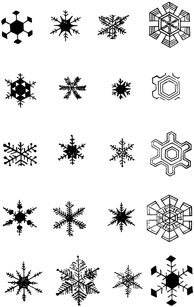
Fig. 92 — Snow Crystals.
