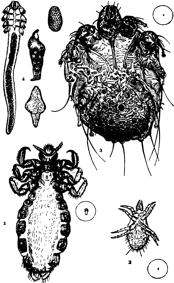
Fig. 290.—Parasites. Acarina .
