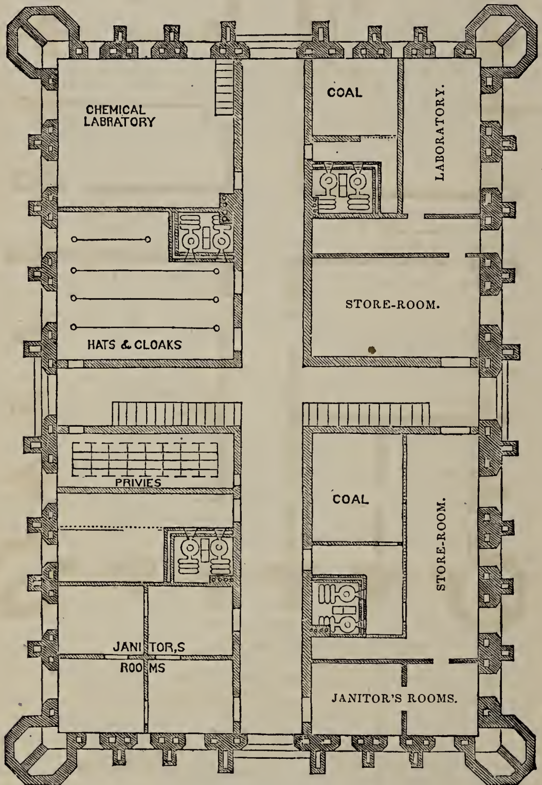
Fig. 3.—BASEMENT FLOOR.
