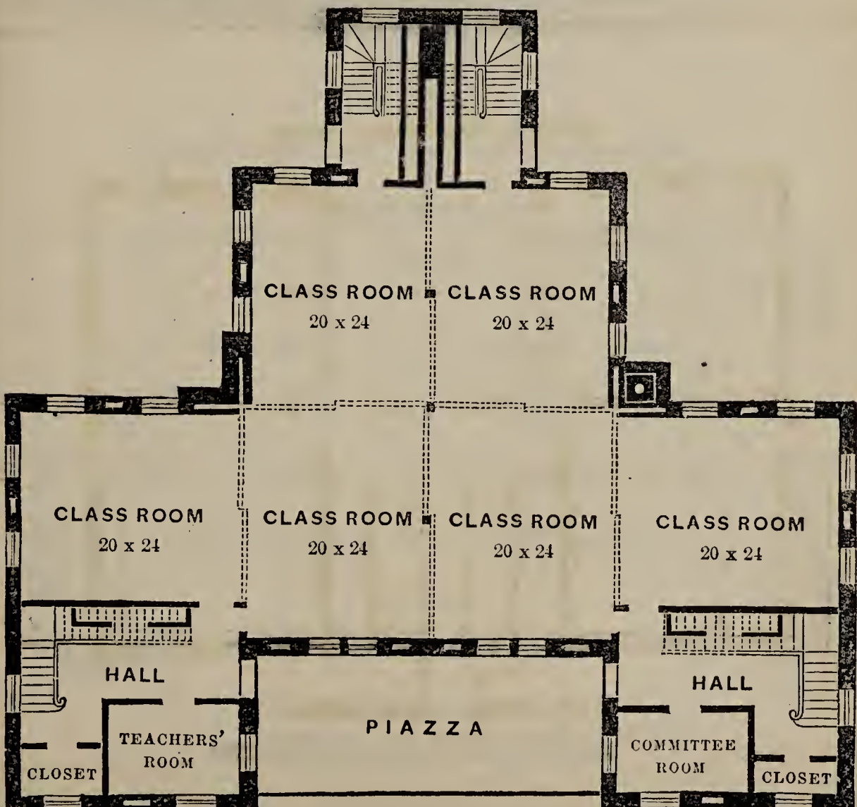
PLAN OF FIRST FLOOR.
