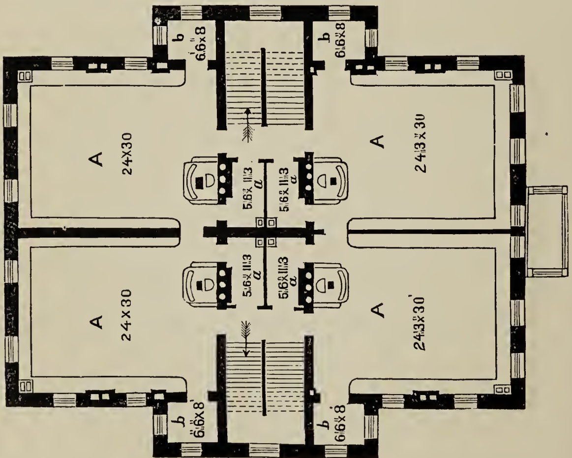
SECOND FLOOR.
