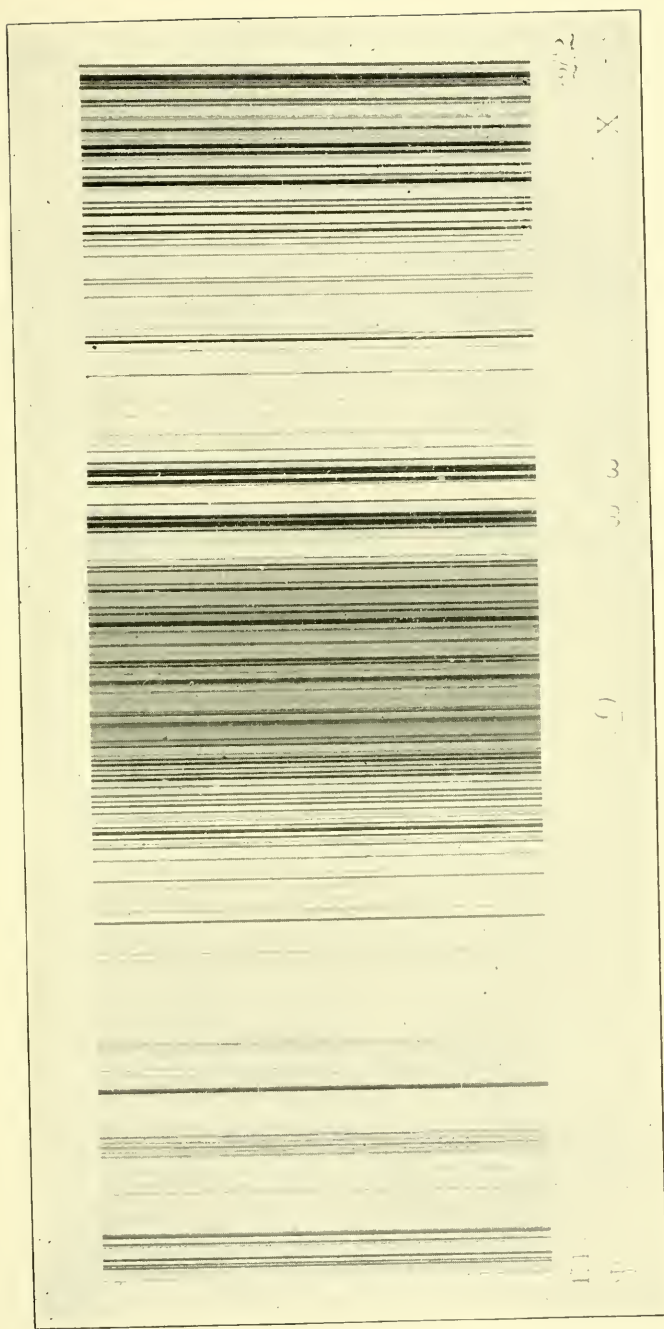
PART OF THE INFRA-RED SPECTRUM.
