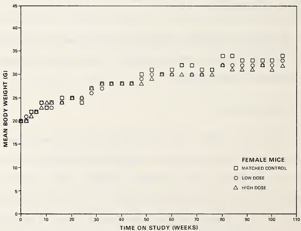
Figure 3. Growth Curves for Mice Administered dl-Menthol in the Diet
