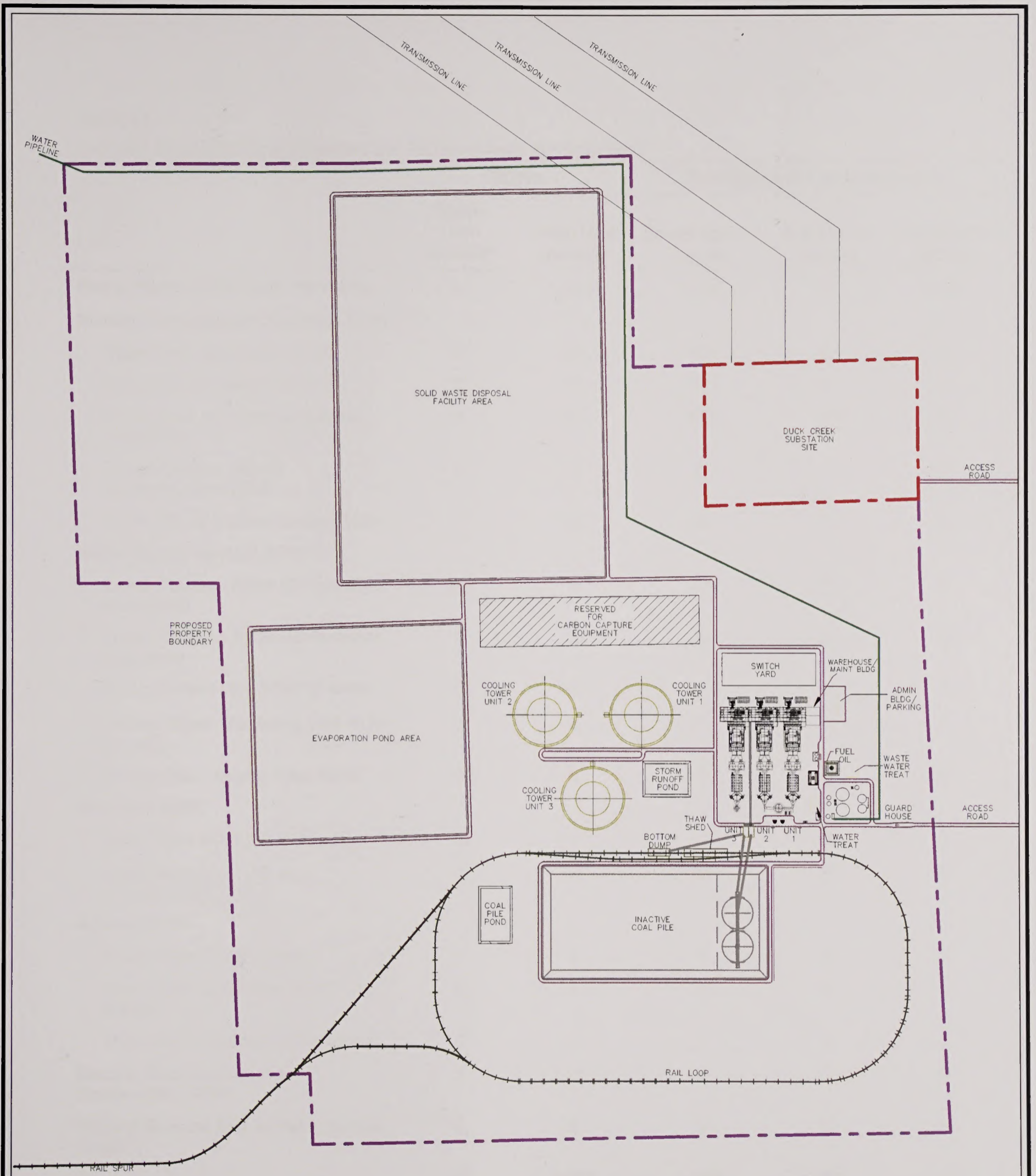
Preliminary Site Layout Alternative 1 White Pine Energy Station Project
