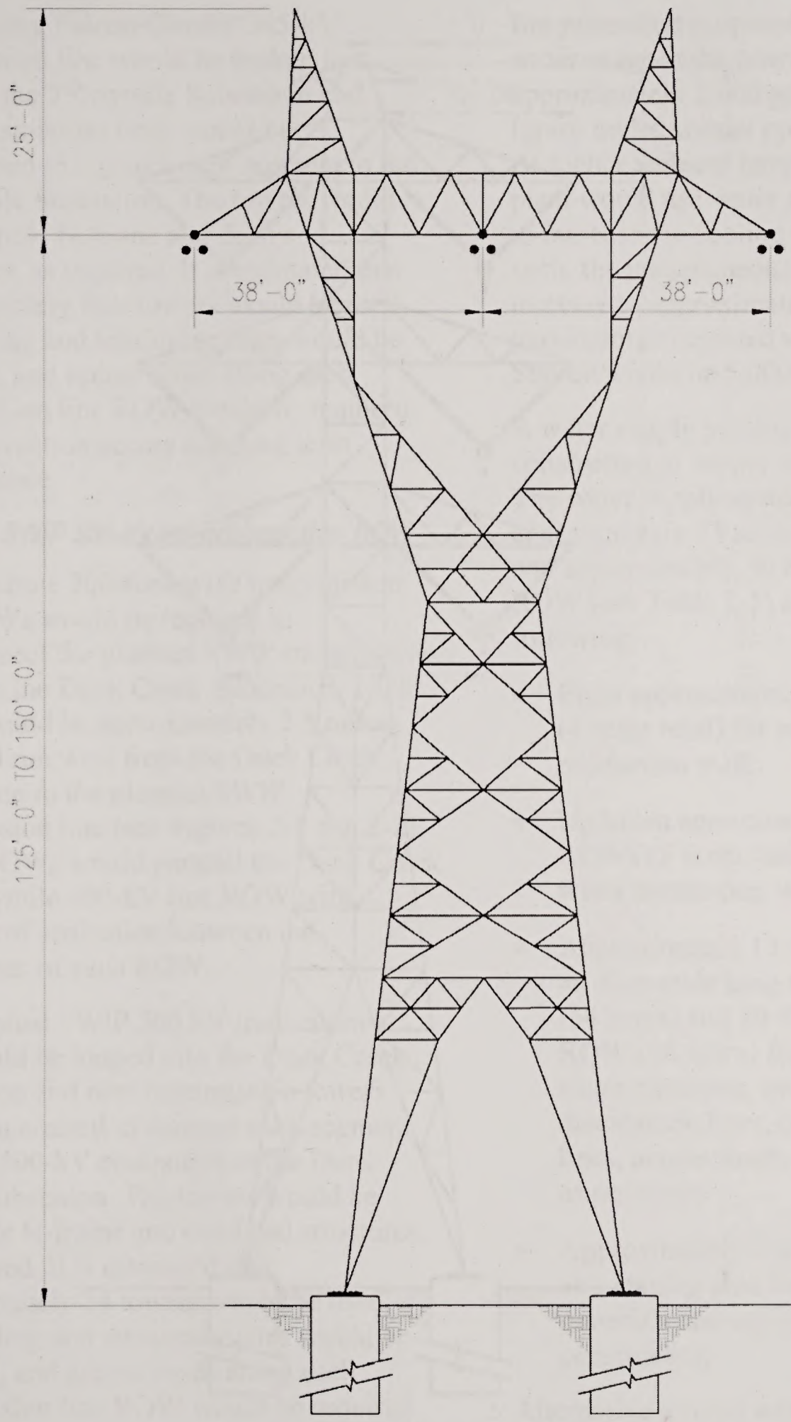
500-kV Transmission Line Typical Single Circuit Dead End White Pine Energy Station Project
