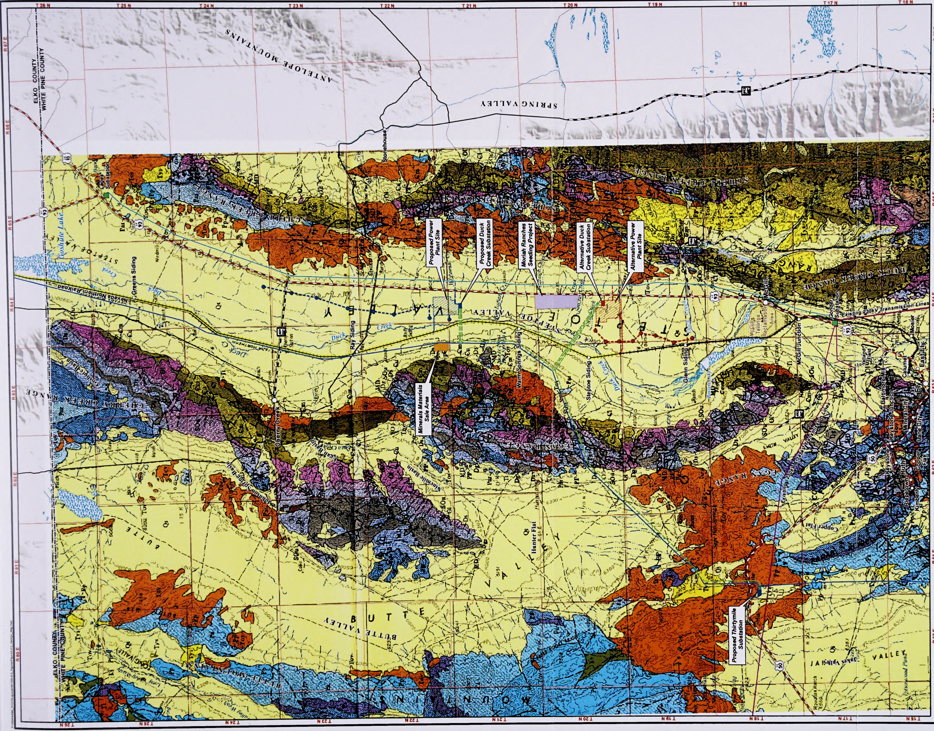
Geologic Map of White Pine County White Pine Energy Station Project Figure 3.2-2
