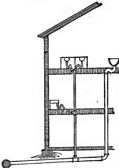
FIG. 24.—Soil pipes and waste pipes without ventilation.
