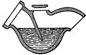
FIG. 57.—Redhill Trap.
