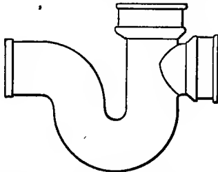
FIG. 44—Mott's Running Trap, with opening for fresh air.
