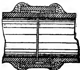
FIG. 266b.—Cement Joint in Vitrified Plain Pipe.
