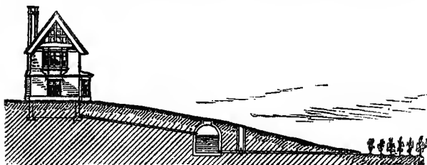
FIG. 268.—Disposal of Household Wastes by Surface Irrigation Mr. Edward S. Philbrick, C.E., at his country seat at Newport, R. I.* For cottages having little ground about them, this method of disposal
