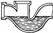
FIG. 70—Croydon Siphon Trap.
