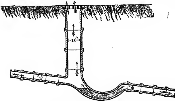
FIG. 54—Disconnecting Trap.
