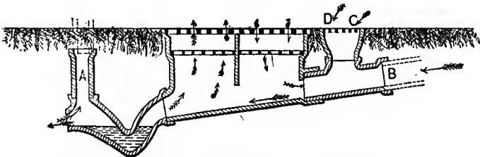
FIG. 68—Potts' Air-chambered Disconnecting Trap.
