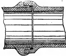
FIG. 266a.—Cement Joint in Vitrified Socket Pipe.
