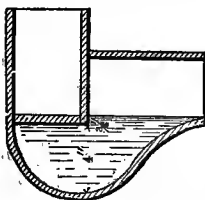
FIG. 91.—Smeaton's Eclipse Trap.
