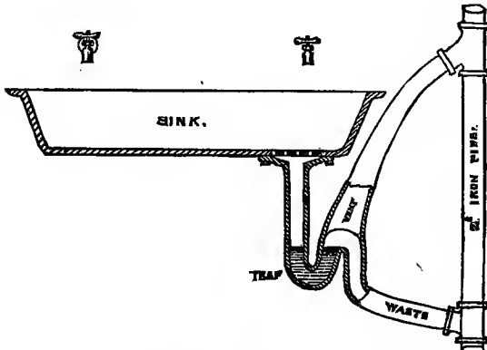
FIG. 207.—Kitchen Sink trapped by a vented S-trap.
