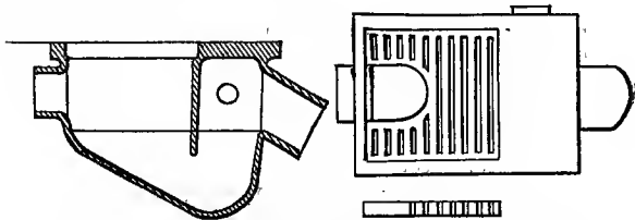
FIG. 74.—J. Tyler & Sone's glazed stoneware disconnecting chamber Sewer Trap.
