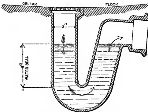
FIG. 167.—S-trap for cellar floor drains.
