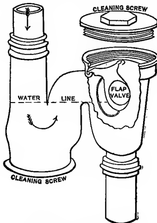
FIG. 150.—Barrett's Trap.
