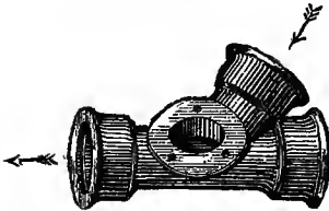
FIG. 200.—45° Y branch for cast-iron drain pipes, shown in perspective.
