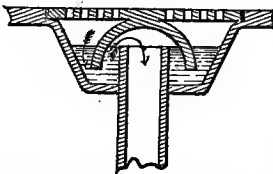
FIG. 99.—Common Bell-Trap.
