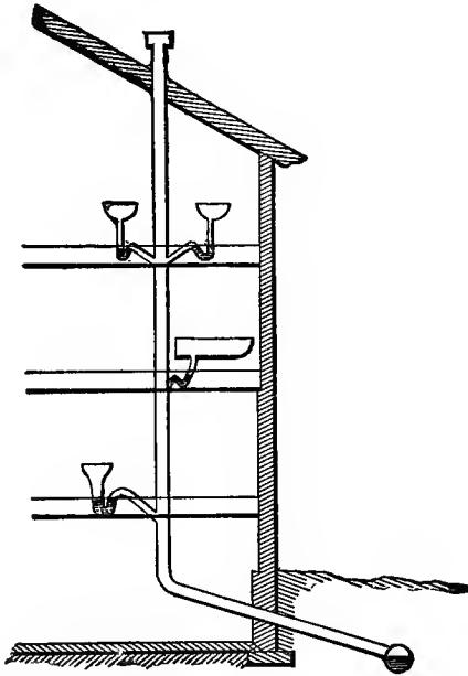
FIG. 36.—Fixtures trapped and soil pipe extended full size above the roof, but house drain left in direct connection with sewer or cesspool.
