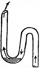
FIG. 18.—Water seal of S-trap lost by siphonage or evaporation.
