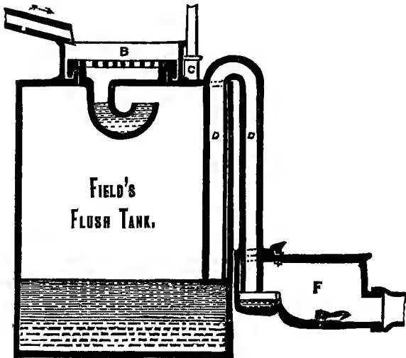
FIG. 278.—Field's Flush-tank.
