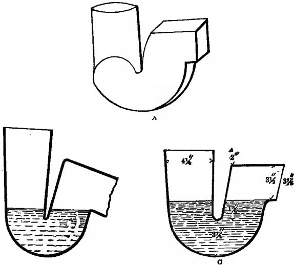
FIG. 93 a, b, c.—Hellyer's Anti-D-Trap.
