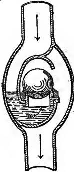
FIG. 146.—Jennings' Trap.
