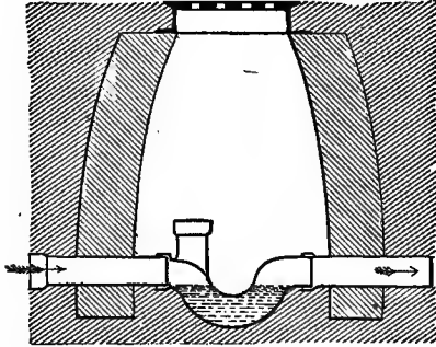
FIG. 49.—Trap and opening for fresh air located in a manhole.
