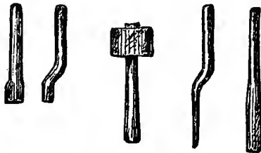
FIG. 185.—Caulking Tools.
