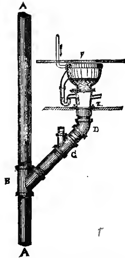
FIG. 190.—Soil Pipe with branch supporting a trap-less water-closet.
