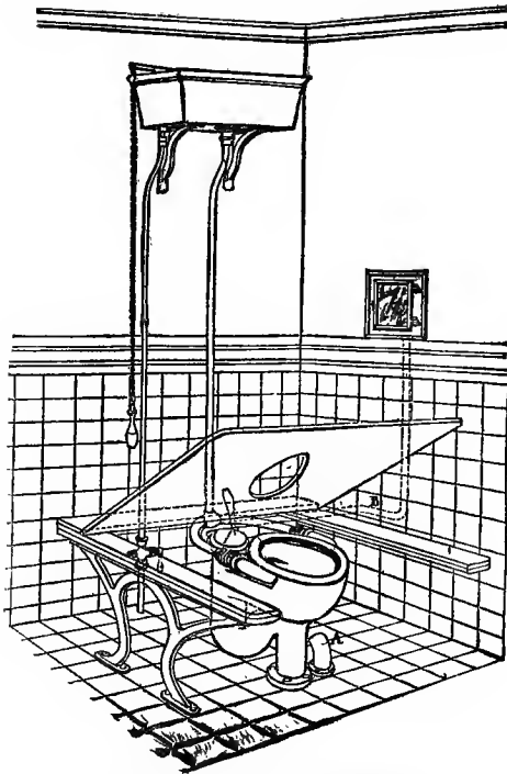
FIG. 25L.—Brighton water closet seat.
