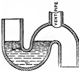
FIG. 160.—S-trap with vent pipe at crown of trap.
