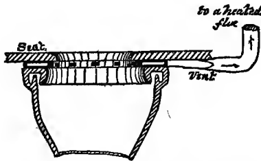
FIG. 256.—Vent of Water-closet under the seat.
