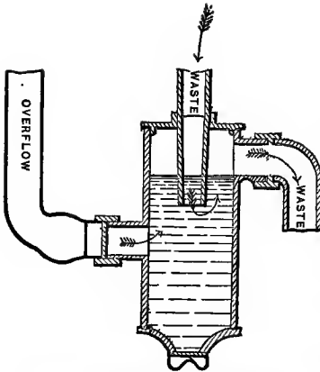
FIG. 120.—Stidder's Patent Soap Trap.
