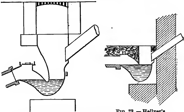
FIG. 72.—Hellyer's Soil-pipe Disconnector. FIG. 73.—Hellyer's Drain Interceptor.
