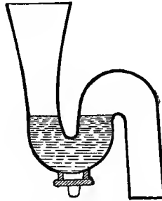
FIG. 107.—Hellyer's Slink S-Trap.
