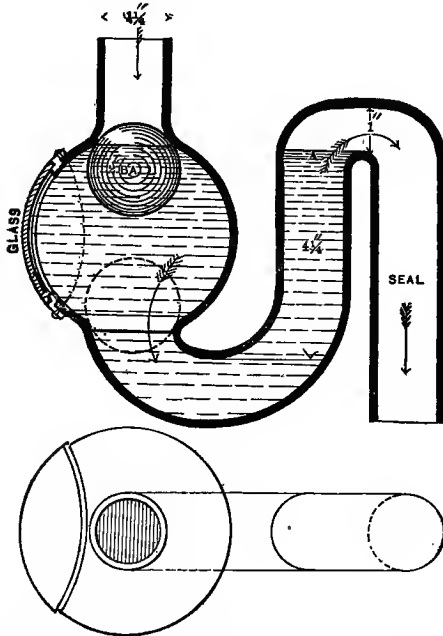
FIG. 157.—The author's suggestion for a Non-Siphoning, Self-Cleaning Trap.
