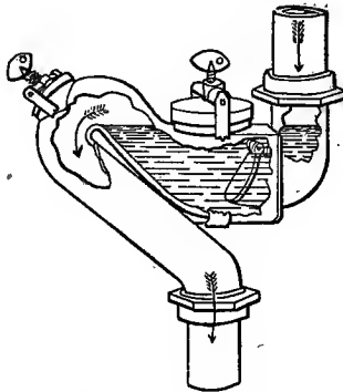
FIG. 148.—Clement's Trap.
