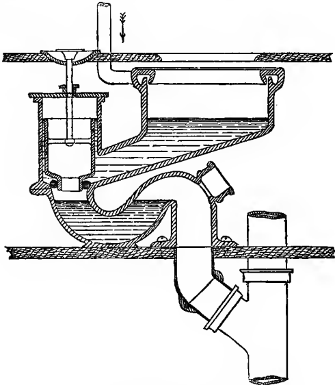
FIG. 13.—Plunger Closet.
