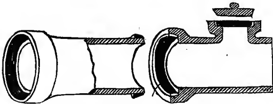
FIG. 267.—Stanford Patent Joint Pipe.
