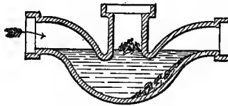
FIG. 50.—Bad form of running trap.
