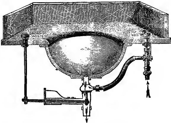
FIG. 221.—Stidder's Waste for Bowls.
