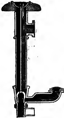
FIG. 226. — McFarland's Waste.
