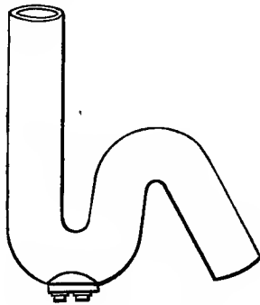
FIG. 109.—Du Bois' \frac{3}{4} S-Trap.
