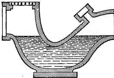
FIG. 65—Weaver's Trap.
