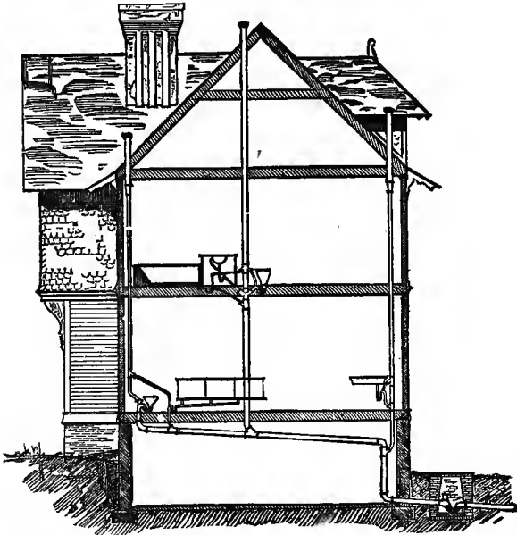
FIG. 183.—Soffit, Waste and Air Pipe System in a Country Dwelling.
