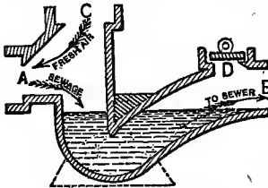
FIG. 58.—Buchan's Trap.
