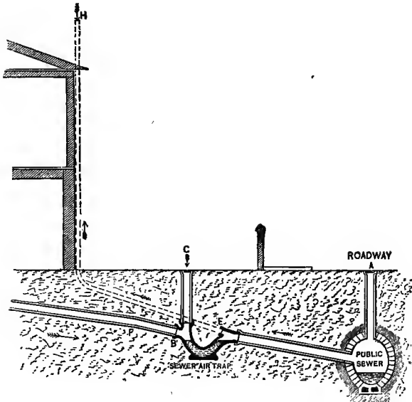
FIG. 65a.—Ventilation of the house drain and the sewer, as effected by Weaver's Trap.
