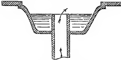
FIG. 8. —Bell Trap with Strainer removed.
