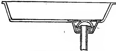
FIG. 7.—Sectional view of Kitchen Sink, with Bell Trap and Strainer.
