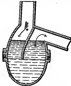
FIG. 119.—Brandeis' "Climax" Trap.
