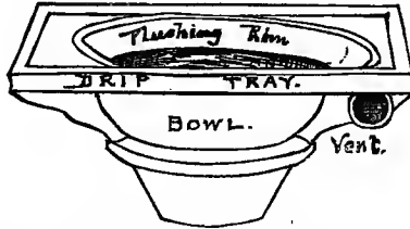
FIG. 260.—Vent of Water-closet from side of bowl.
