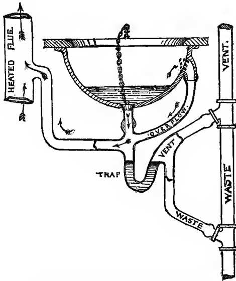
FIG. 258.—Ventilation of House-side of Trap.
