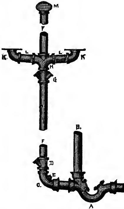
FIG. 188.—Soil Pipe Stack as erected by the Durham House Drainage Company.
