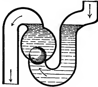
FIG. 143.—Turner's Trap.
