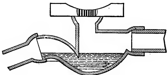
FIG. 59—Molesworth's Trap.
