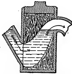
FIG. 118.—Boston Round Trap, with filth accumulation.
