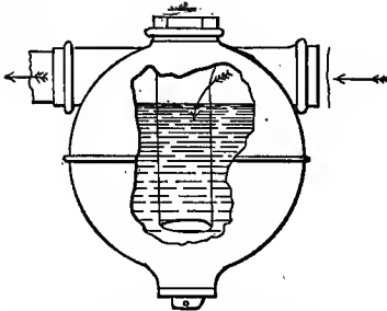
FIG. 126. — Connolly's Patent Globe Trap, of copper, running trap.
