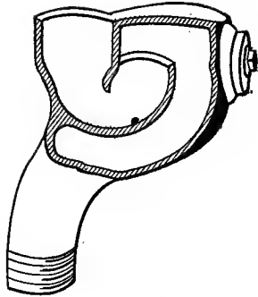
FIG. 105.—J. Tylor's Trap.
