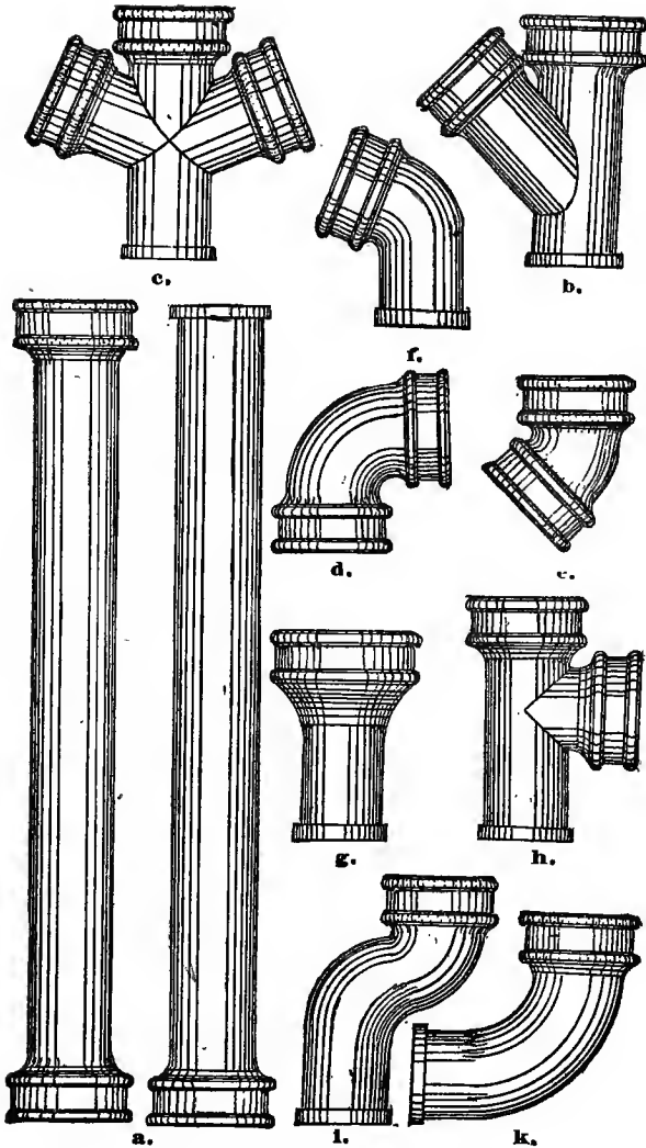
FIG. 20.—Cast Iron Plumbers' Pipe and Fittings.
