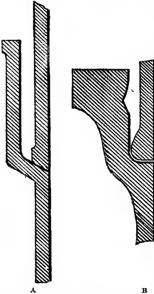
FIG. 21.—Sketch showing comparative strength of hubs of plumbers' pipe and gas pipe.
