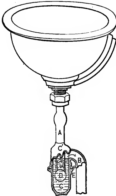
FIG. 132.—Washbowl, trapped by Bower's Trap.
