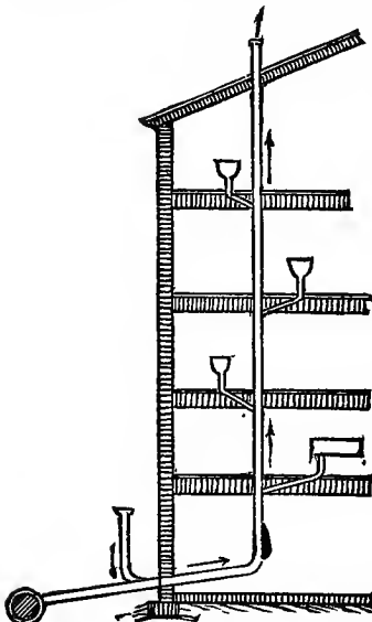
FIG. 28.—Proper method of ventilating a soil pipe.
