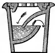
FIG. 100.—Antill's Trap. FIG. 101.—Jennings' Improved Bell-Trap.
