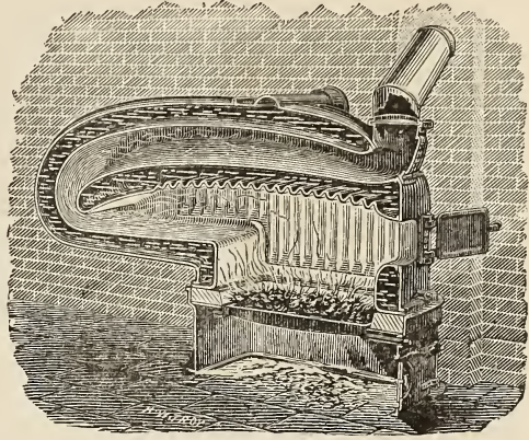
HITCHINGS' CORRUGATED BOILER.
