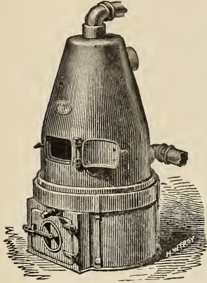
HITCHINGS' CONICAL BOILER.
