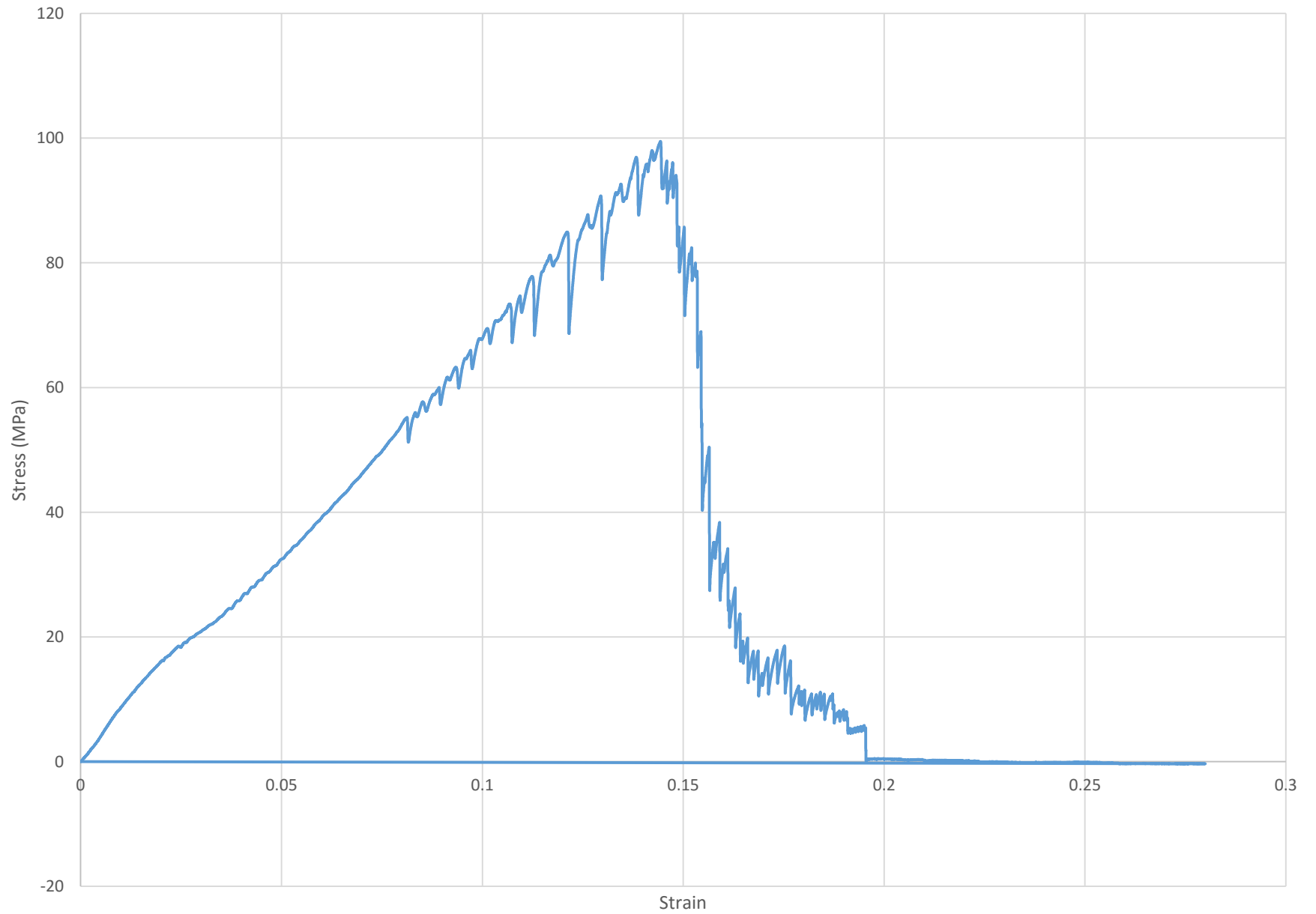
Sisal Twine at 200 mm/min
