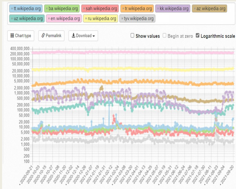
Daily Pageviews: from 2020-09-21 to 2021-09-20 Descending en-ru-tr-kk-az-uz-tt-ba-sah-tyv
