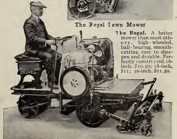
Caldwell Motor Mower
