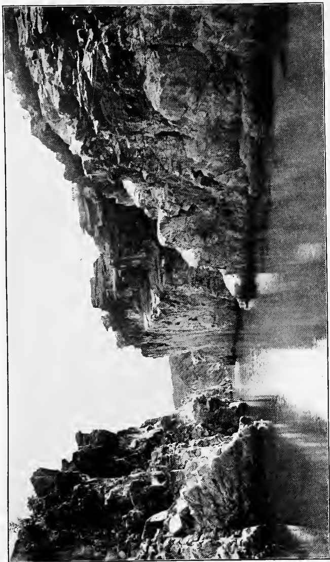
MARBLE ROCKS ON NARBUDDA RIVER, NEAR JABALPUR.
