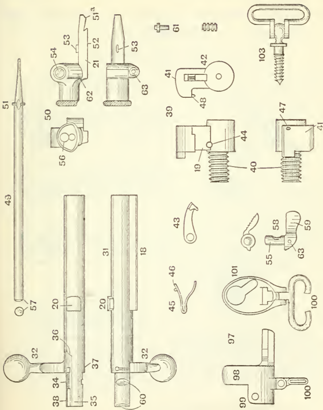
Fig. 63.—CHARGER-LOADING LEE-ENFIELD
