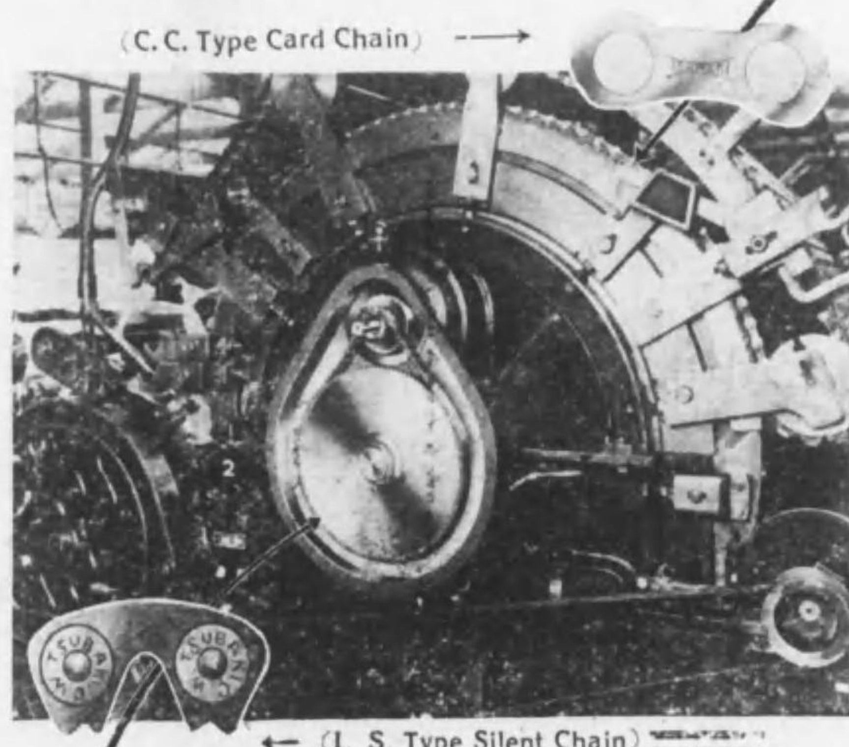
← (L. S. Type Silent Chain)
