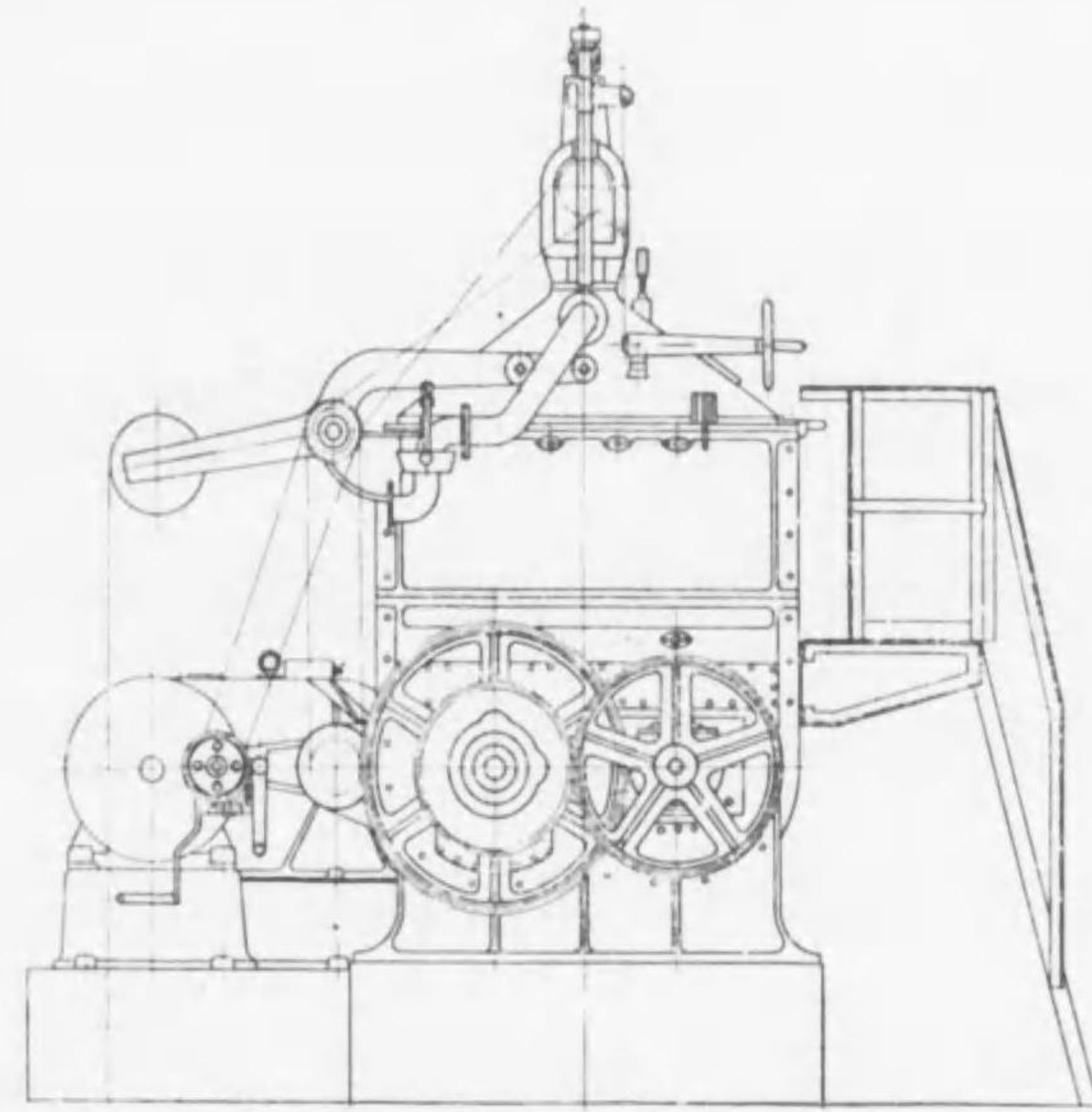
VACUUM XANTHATE KNEADER
