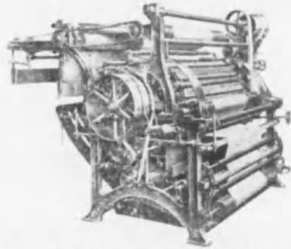
Gessner's Latest wire Card Raising Machine, Pat. Prof. Mundorf.
