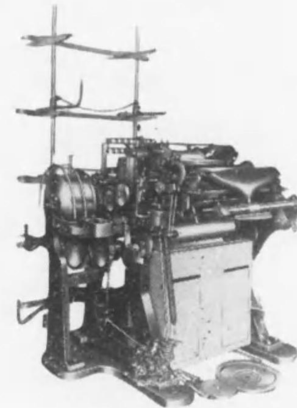
Y. B. Combing machine (Worsted)
