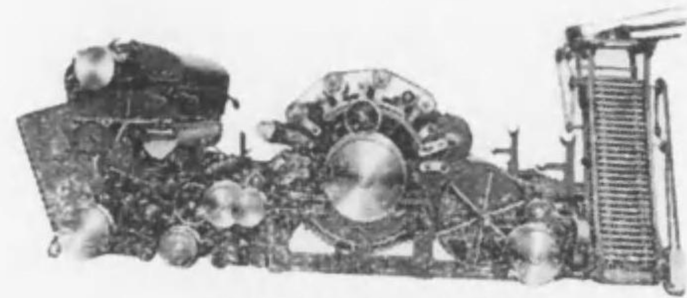
(1) Breaker Card.
