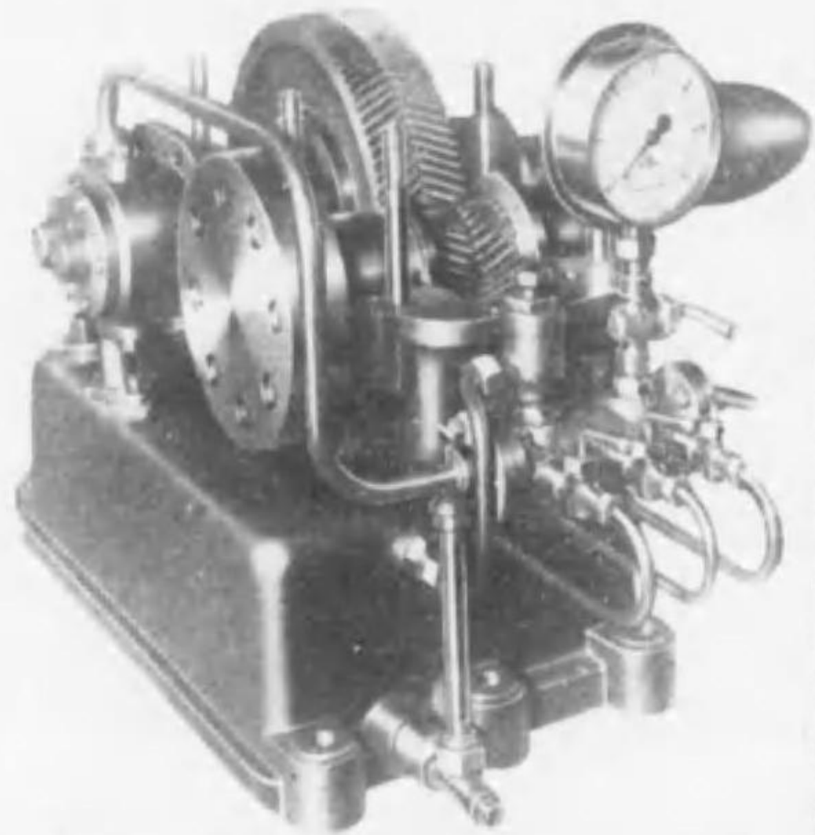
"S.G.W." HERRING BONE GEAR SPEED REDUCER 30B.H.P. 1800 r.p.m.-Motor to 442 r.p.m.
