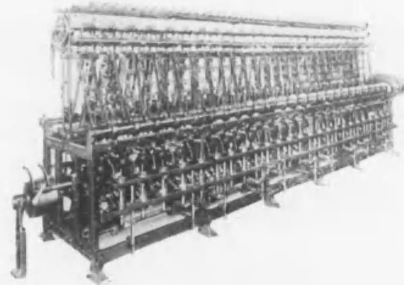
Twister (Rayon)
