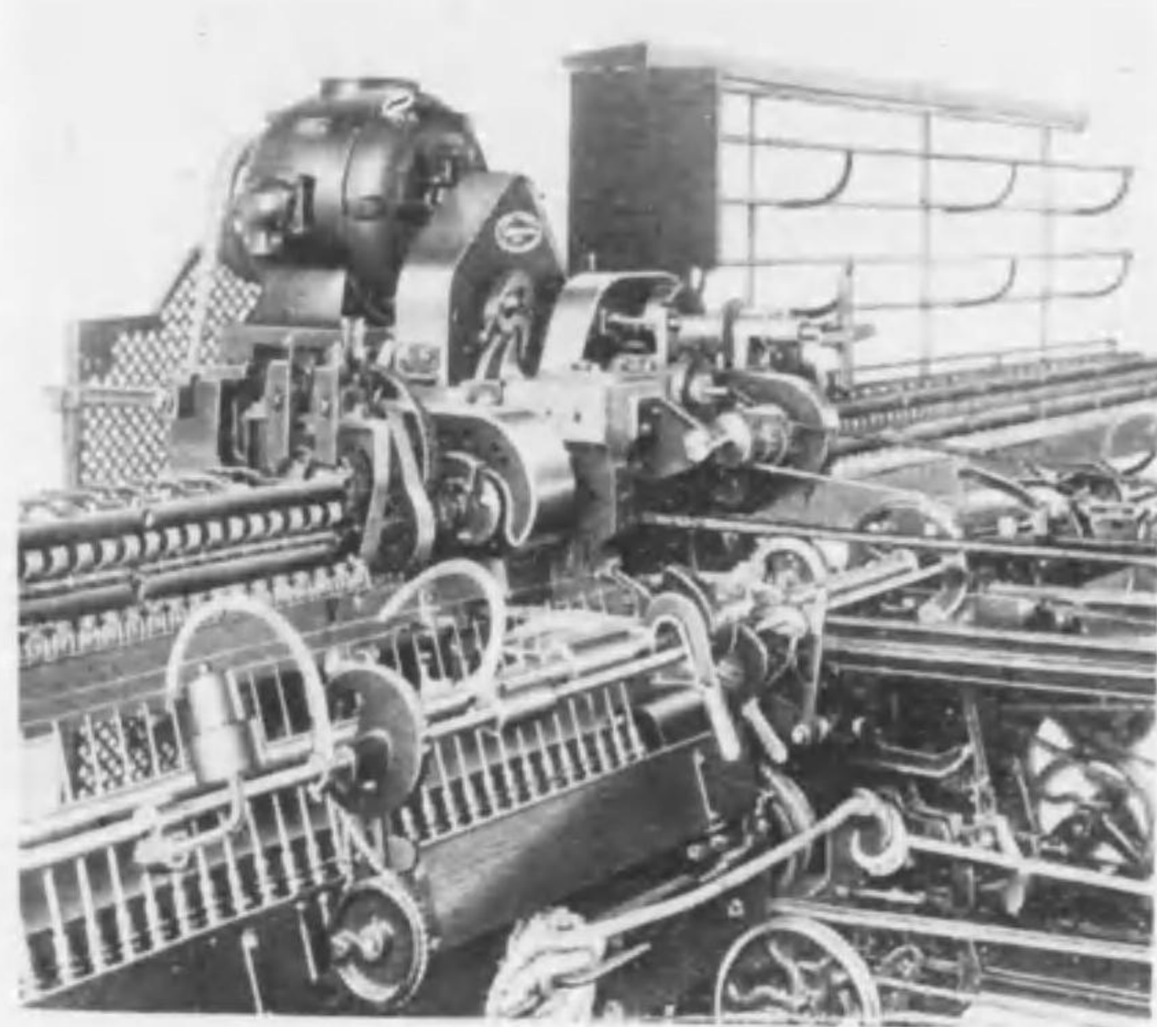
Worsted Mule with differential motion system "Taine",
