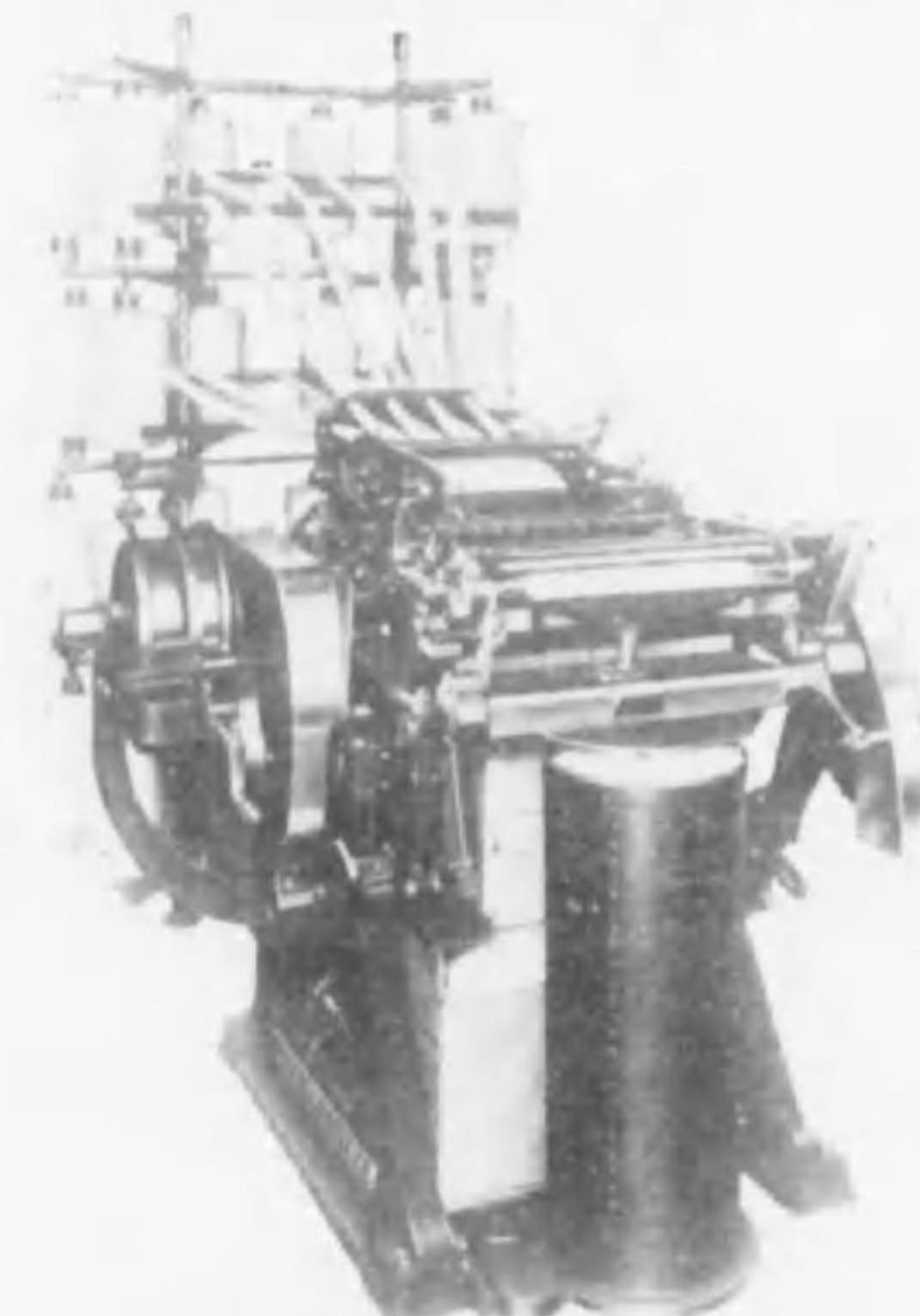
Comber (Worsted)
