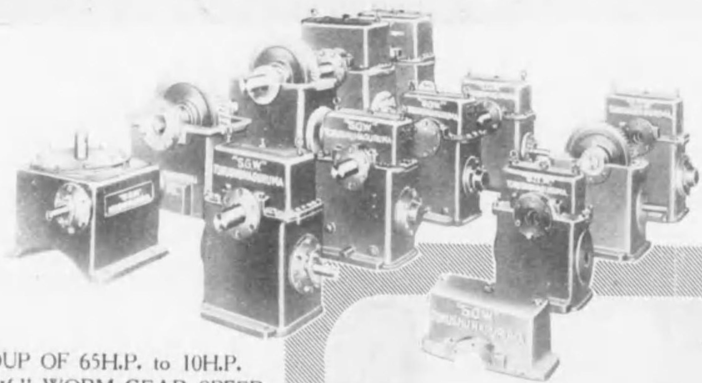
"S.G.W." HERRING BONE. GEAR TWO SPEED REDUCER 100B.H.P. 600 r.p.m. Motor to 30/70 r.p.m.
