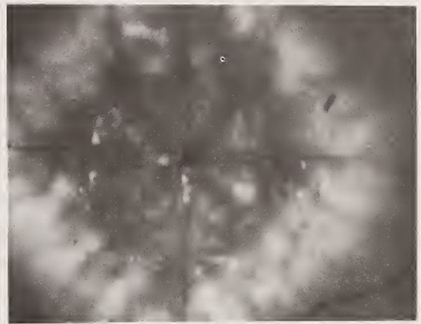
Figure 2. Laser damage at 1.06 μm on an untreated, cleaved NaCl surface.
