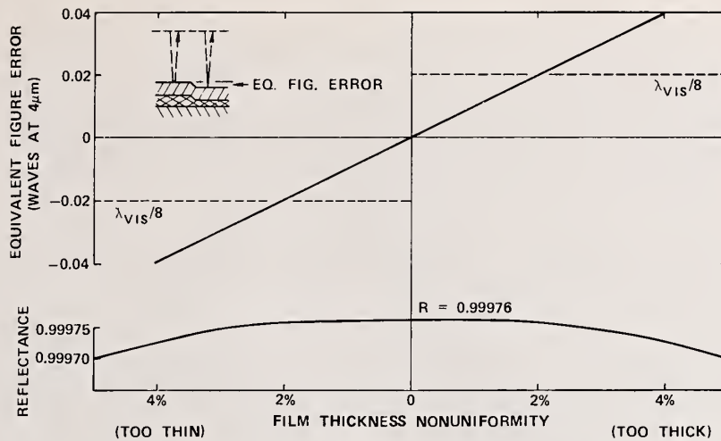
Figure 2. Equivalent figure error in a MLD-coated mirror caused by nonuniform film thickness across the mirror. The multilayer coating design is (ZnS/ThF_4)^4 ZnS^* Ag , and the design wavelength is 3.8 \mu m . The dashed lines give the corresponding figure error in visible wavelengths. They would not be the observed figure errors if measurements were made in the visible, however, because of phase shift.
