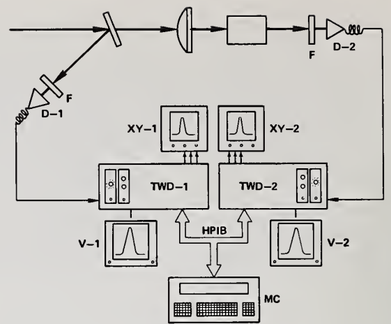
Figure 2. Fast Waveform Analysis Device.
