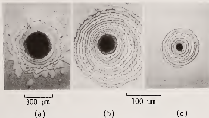
Figure 6. Uniform coating failure observed on a \text{TiO}_2/\text{SiO}_2 stack: (a) axial fluence of 367 \text{ J/cm}^2 ; (b) axial fluence of 63 \text{ J/cm}^2 ; (c) axial fluence of 87 \text{ J/cm}^2 .
