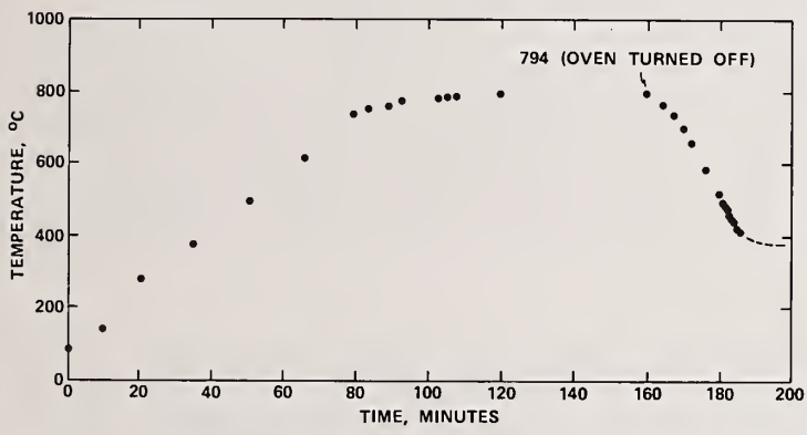
Figure 1. Temperature versus time of single-crystal NaCl. The specimen was heated in a nitrogen atmosphere. It was first brought up to 35°C for 10 min, then taken to 80°C for 187 min, and then heated as shown in the curve above.
