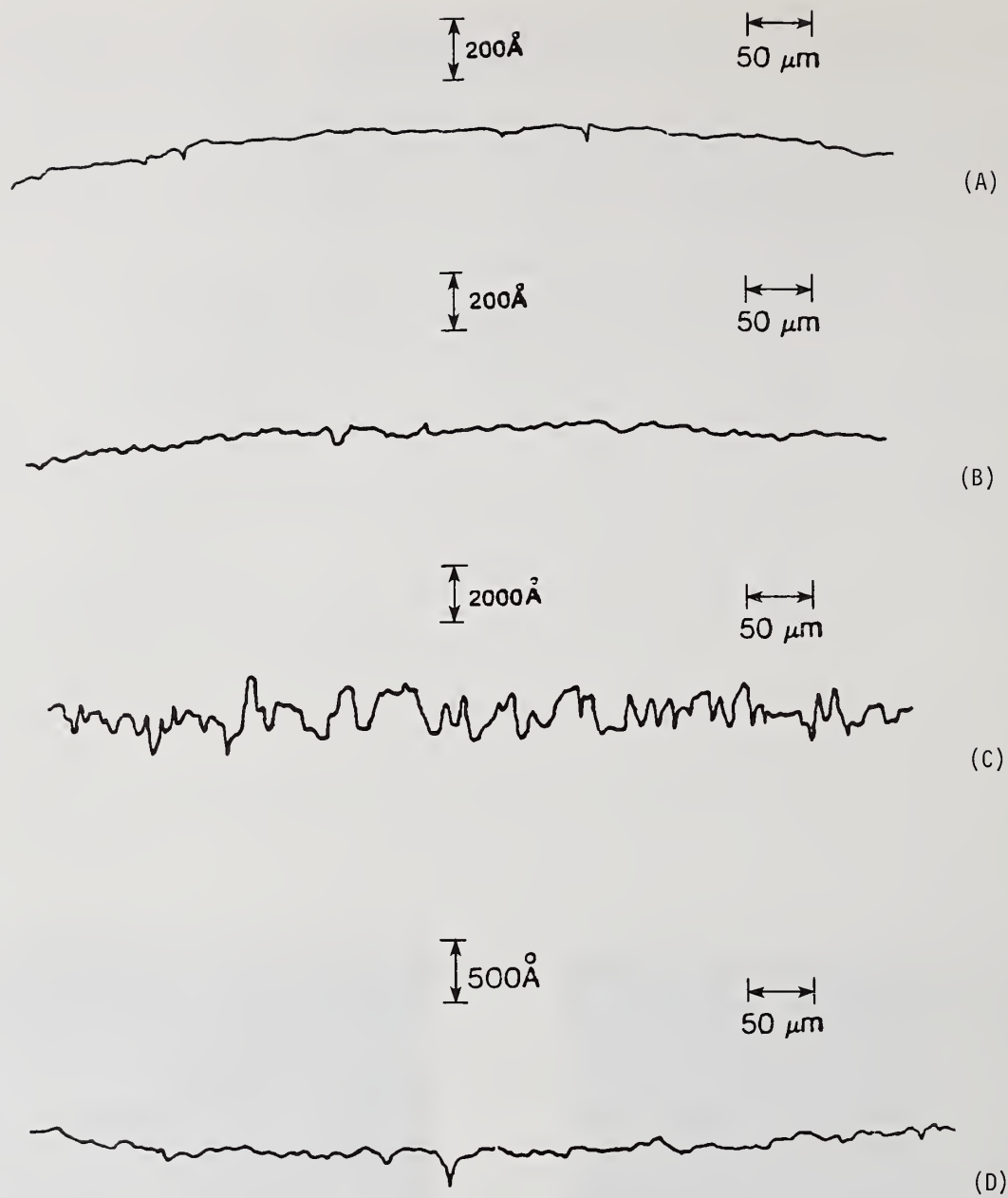
Figure 3. Surface profiles of mechano-chemically polished samples of (A) silicon (B) sapphire (C) tape-cast alumina and (D) hot-pressed Si 3 N 4 .
