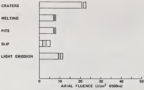
Figure 8. Damage profile of diamond-turned Al alloy at 492 nm.
