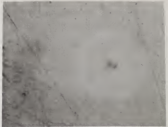
Figure 6. Laser damage at 1.06\ \mu\text{m} on same surface shown in figure 5 with different contrast to show that the extent of damage is approximately the same size as the untreated sample shown in figure 4.
