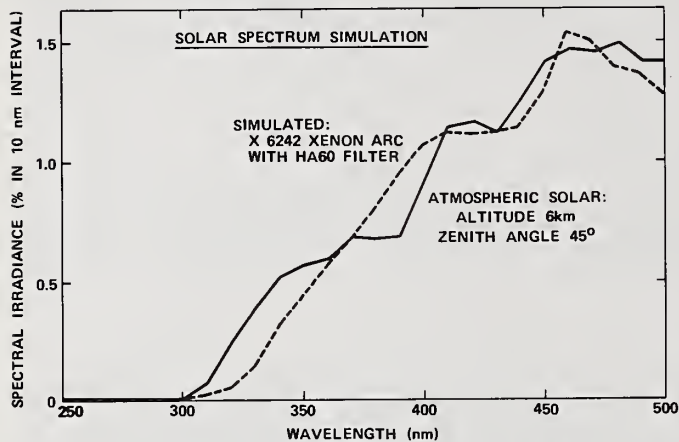
Figure 1. Short-wavelength region of filtered xenon arc spectrum compared with solar spectrum at 6 km, 45-degree zenith angle.
