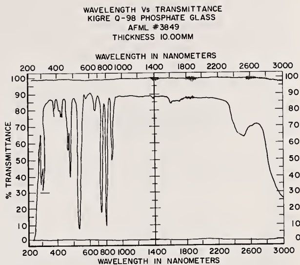
Figure 2. Transmittance versus wavelength for Kigre Q-98 phosphate glass.
