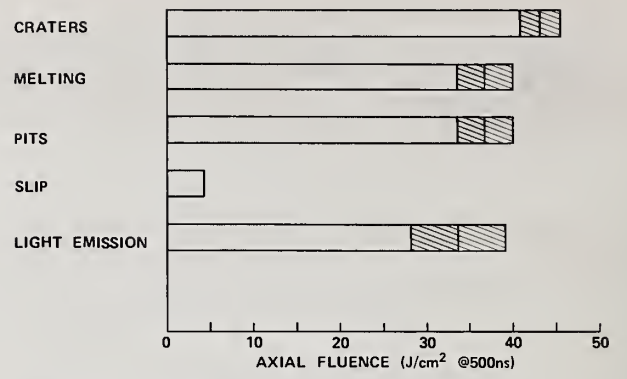
Figure 9. Damage profile of diamond-turned Ag at 492 nm.
