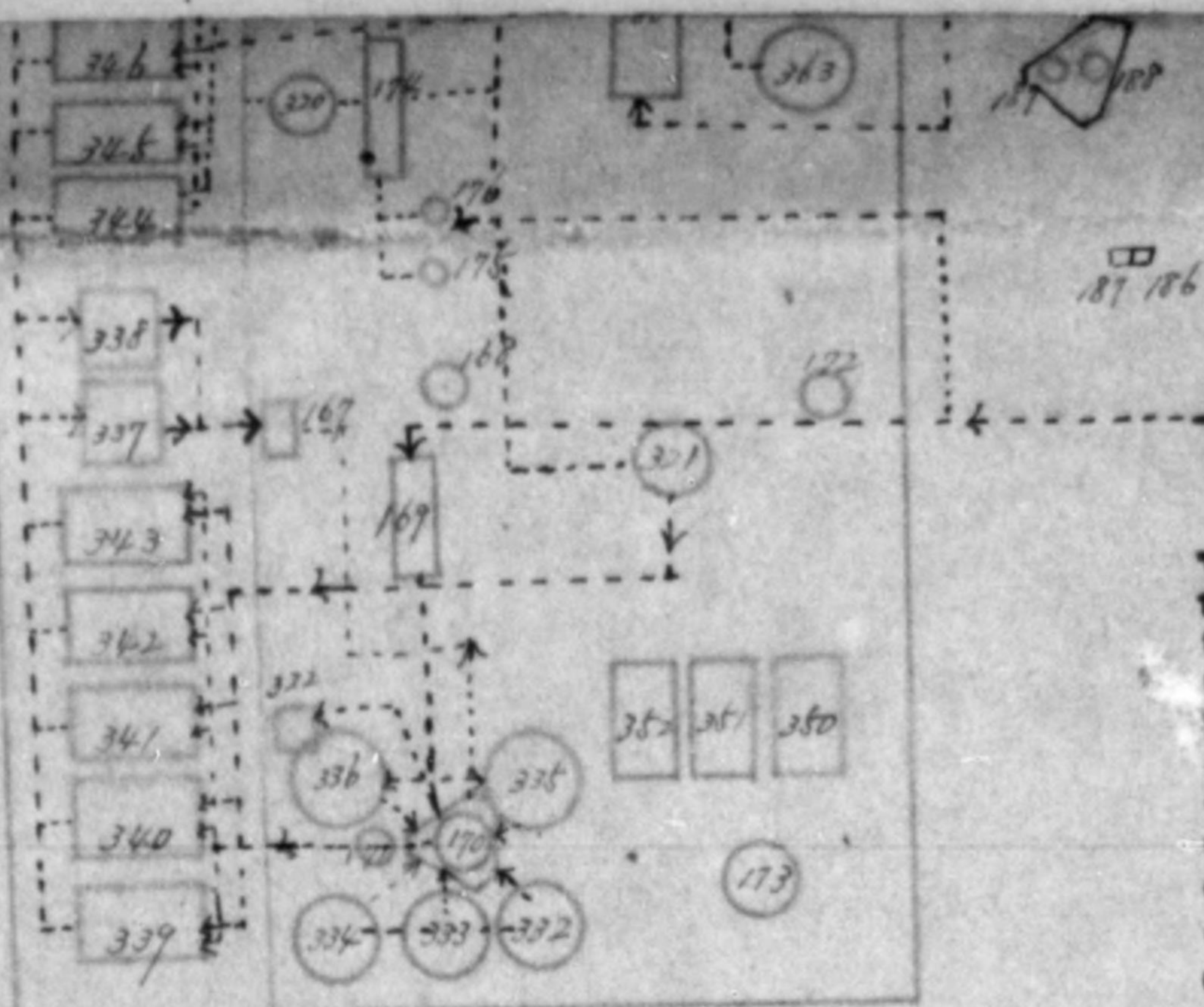
Regenerating plant of catalyst
