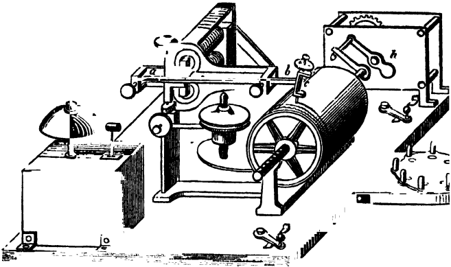
Fig. 7.—Froment's Writing Telegraph.
