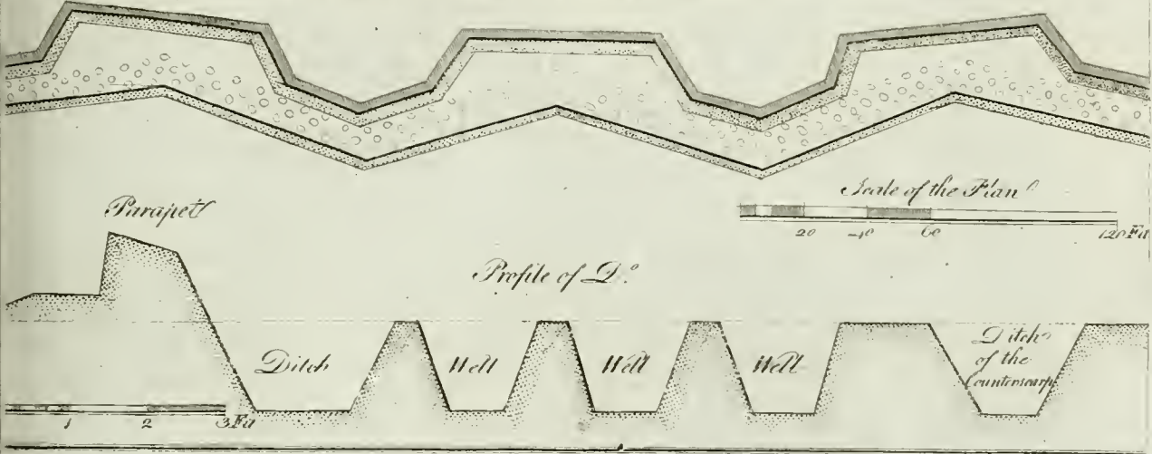
Plan of part of a line of circumvallation of Strass in 1654.
