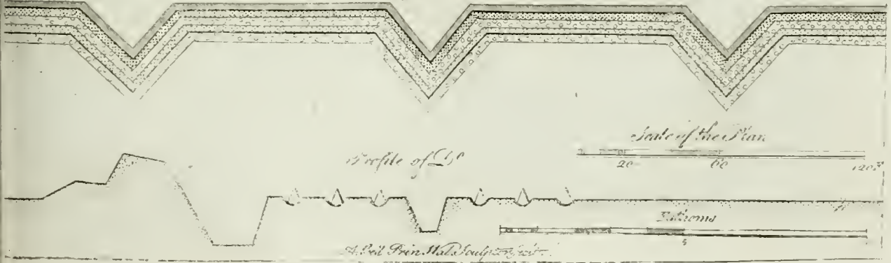
Plan of part of a line of circumvallation of Strass in 1654.
