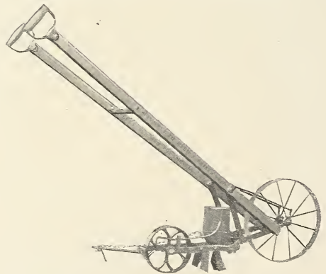
Fig. 2—Garden Raiser Seed Drill (PATENT APPLIED FOR)
