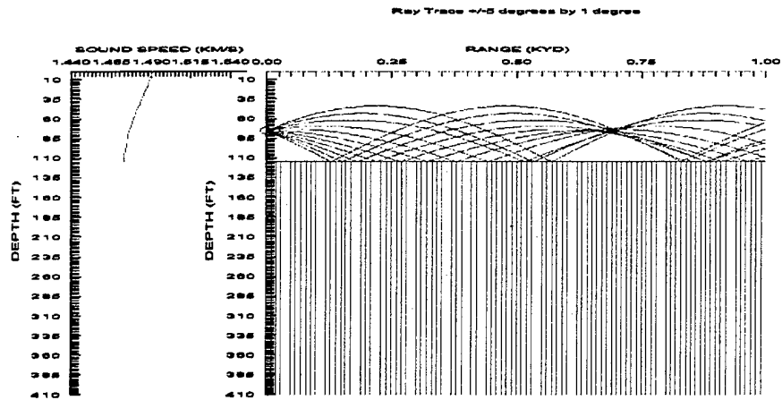
b. Maximum Detection Range (DR) for a Bottom Target Depth = 35 yd, \Delta DR = 655 yd
