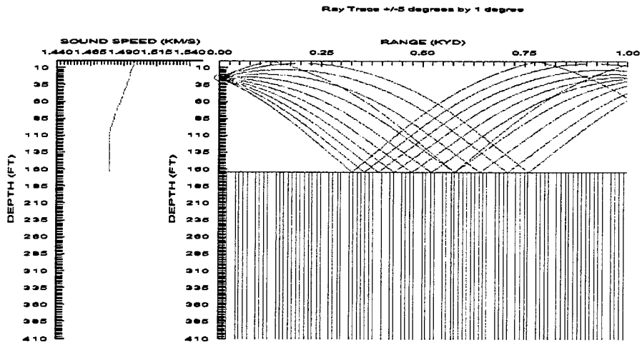
b. Maximum Detection Range (DR) for a 26 ft. Target Depth > 1000 yd, \Delta DR > 860 yd
