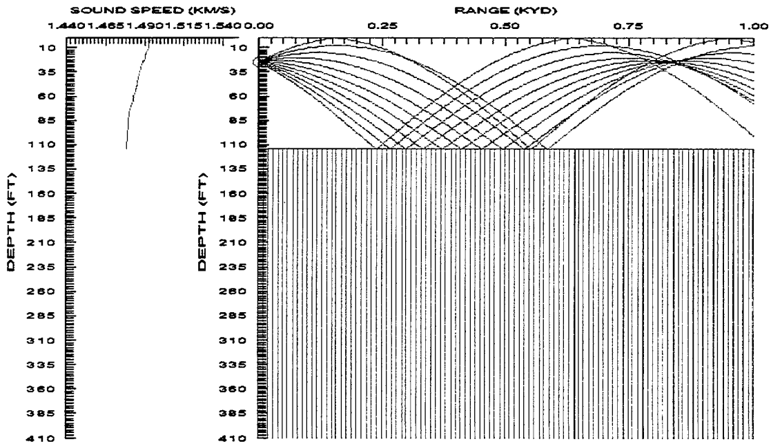
b. Maximum Detection Range (DR) for a 26 ft. Target Depth = 855 yd
