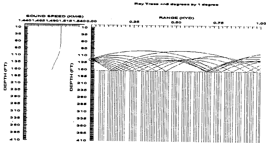
a. Maximum Detection Range (DR) for a 26 ft. Target Depth = 495 yd, \Delta DR = 495 yd
