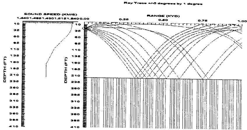
b. Maximum Detection Range (DR) for a 26 ft. Target Depth = 995 yd, \Delta DR = 385 yd
