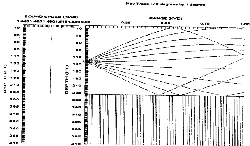
b. Maximum Detection Range (DR) for a Bottom Target > 1000 yd, \Delta DR > 895 yd
