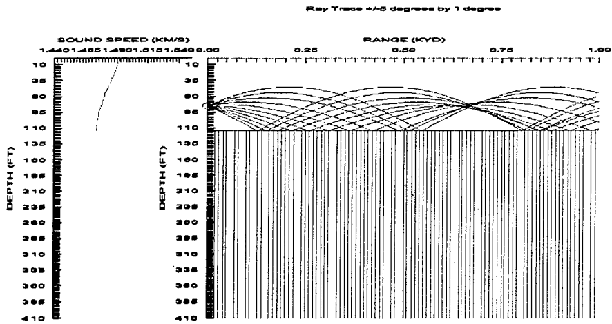
a. Maximum Detection Range (DR) for a Bottom Target Depth = 35 yd, \Delta DR = 655 yd
