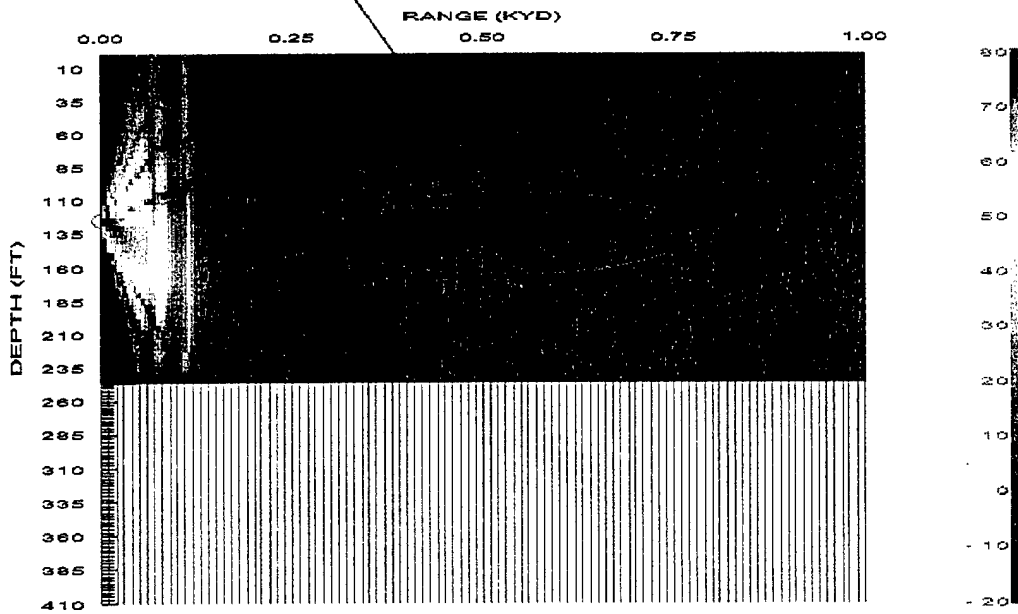
Figure 59. MODAS with +1 m/s Sound Speed error at Source Depth for February 15, 2000, 36.4 N 124.4 E, Mud Bottom, and Source Depth =125 ft. a. Ray Trace, b. Signal Excess Contour Plot (Max Detection Range at Source Depth = 150 yd, \Delta Max Detection Range at Source Depth = 5 yd).
