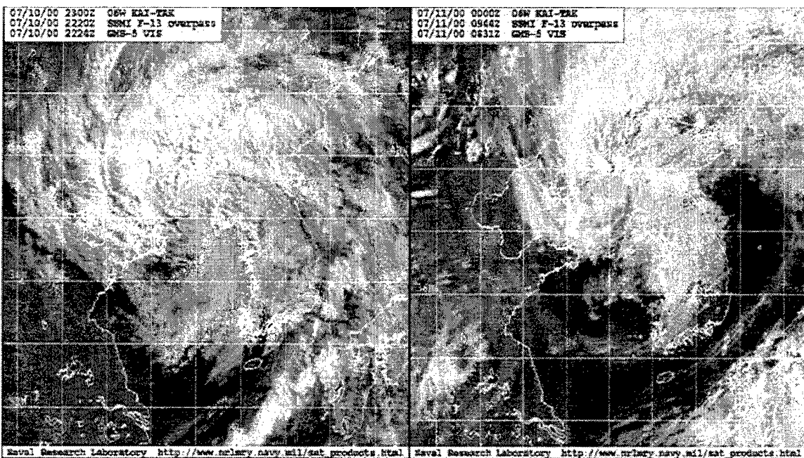
Figure 40. Satellite Images of Tropical Depression Kai-Tak for July 8-11, 2000 respectively (From Naval Research Laboratory 2000).
