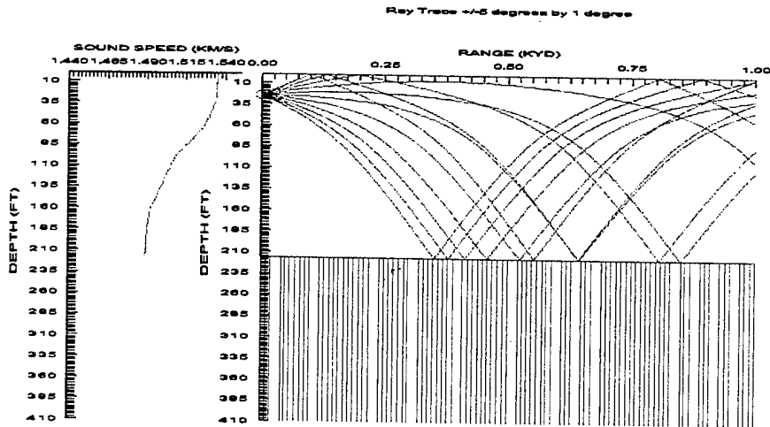
c. Maximum Detection Range (DR) for a 26 ft. Target Depth = 610 yd
