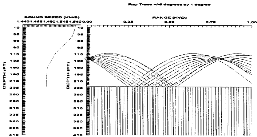
b. Maximum Detection Range (DR) for a 26 ft. Target Depth = 90 yd, \Delta DR = 545 yd
