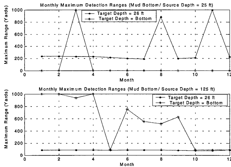
Figure 33. Monthly maximum detection ranges for a Mud Bottom at two source depths and target depths.
