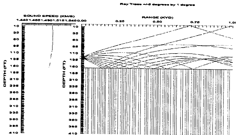
c. Maximum Detection Range (DR) for a 26 ft. Target Depth = 0 yd
