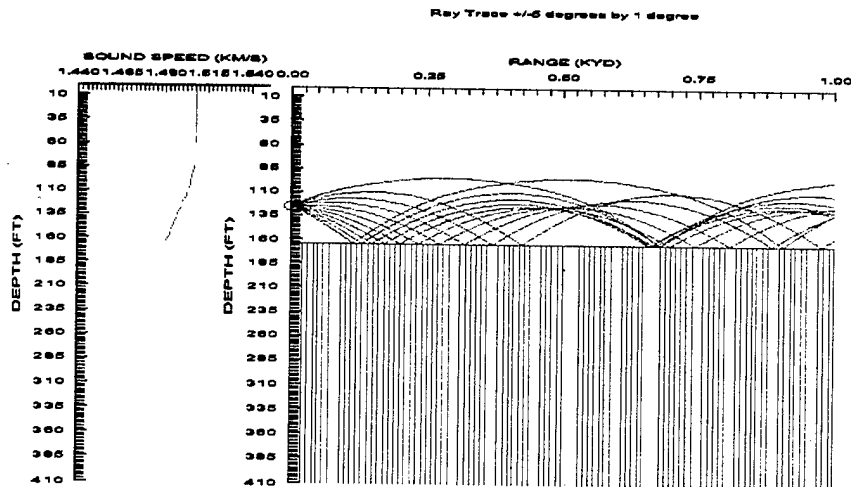
b. Maximum Detection Range (DR) for a 26 ft. Target Depth = 510 yd, \Delta DR = 510 yd
