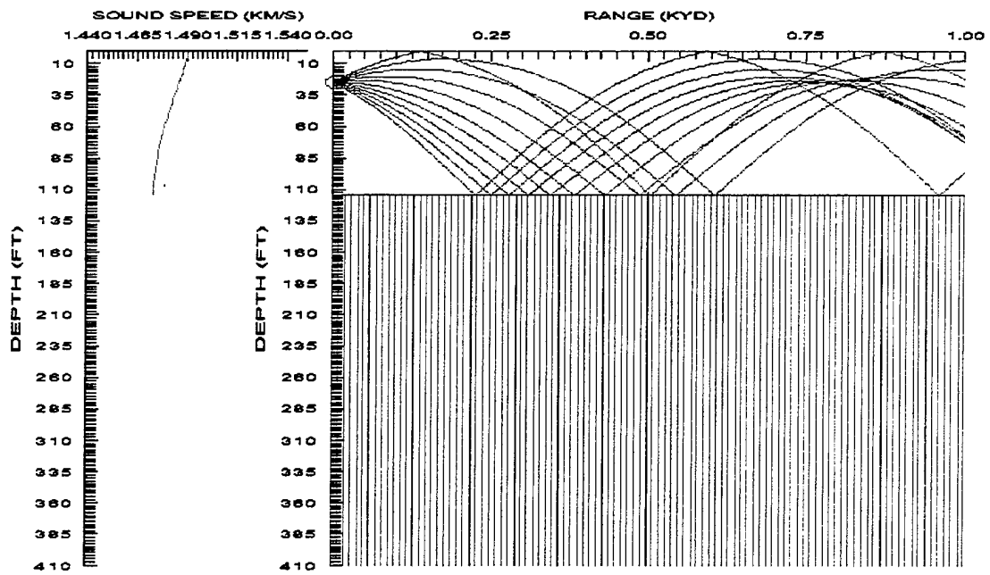
a. Maximum Detection Range (DR) for a 26 ft. Target Depth = 80 yd, \Delta DR = 775 yd
