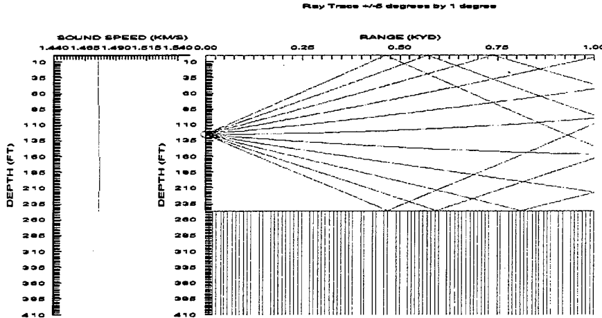
b. Maximum Detection Range (DR) for a Bottom Target Depth = 0 yd, \Delta DR > 1000 yd
