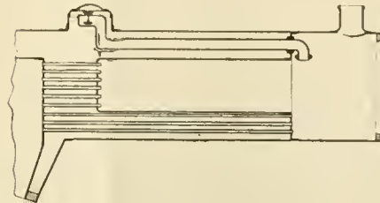
LOCOMOTIVE SUPERHEATER.
