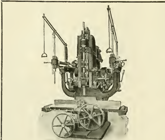
No. 214, Vertical Hollow Chisel Mortiser.
