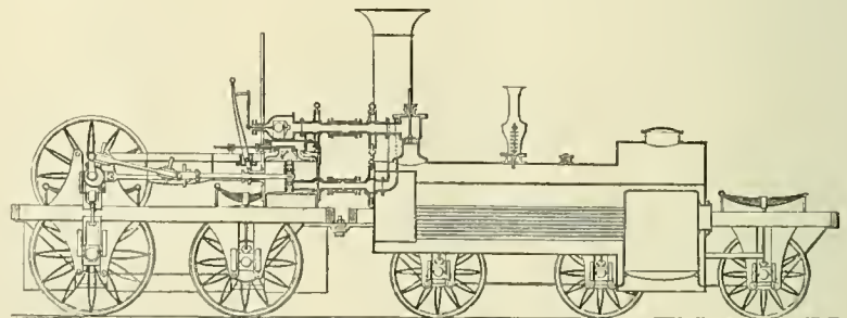
FIG. 10. HARRISON'S "THUNDERER."
