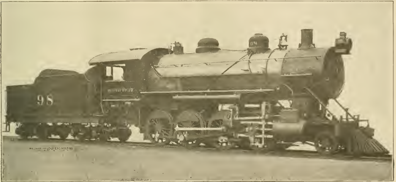
CONSOLIDATION TYPE ENGINE FOR THE MISSOURI PACIFIC.
