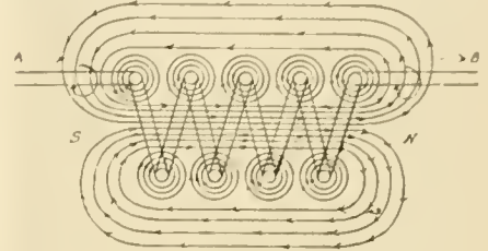
FIG. 1. FLOW OF CURRENT THROUGH SIMPLE COIL.
