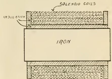
FIG. 3. WINDING OF A SOLENOID.
