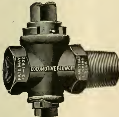
Iron Body, Brass Plug, 1 1/2 in.
