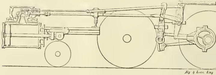
FIG. 3. CLARK'S INDEPENDENT CUT-OFF MOTION.
