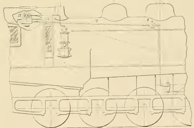
FIG. 1. THE GENERAL ARRANGEMENT.
