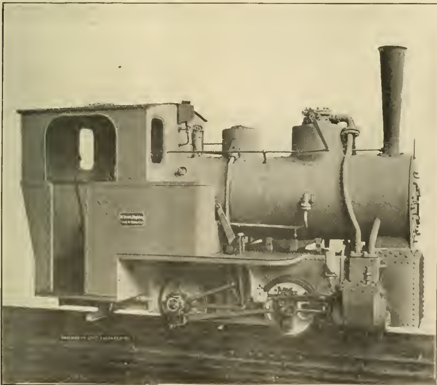
FIG. 1. NARROW GAUGE TANK ENGINE FOR INDUSTRIAL SERVICE.
