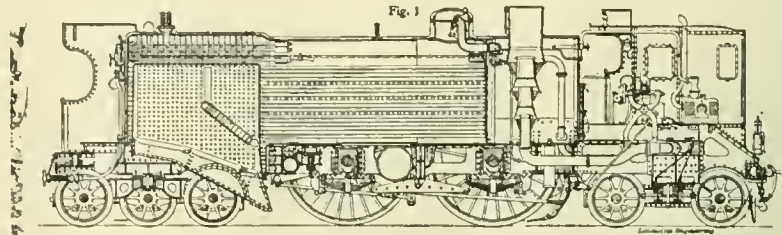
FIG. 22. THUILE LOCOMOTIVE.
