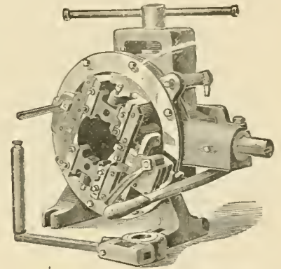
FIG. 2. SMALL PIPE MACHINE.
