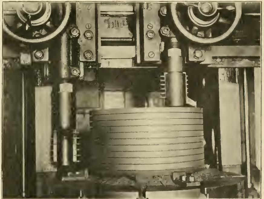
CYLINDER PACKING QUICKLY MADE ON A BORING MILL.
