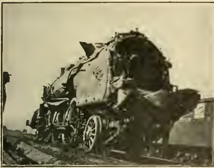
RESULT OF DEFECTIVE TRACK.
