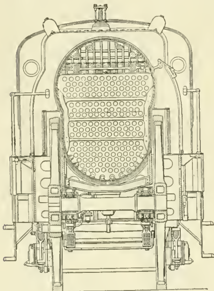
FIG. 23. SECTION OF BOILER OF THE THUILE LOCOMOTIVE.
