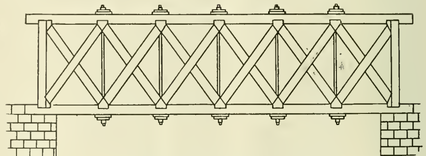
SKELETON OF THE HOWE TRUSS BRIDGE.
