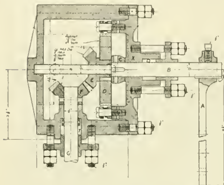
FIG. 2. SECTION OF TRANSFORMER.
