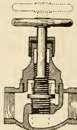
VALVE WITH SCREW SEAT.
