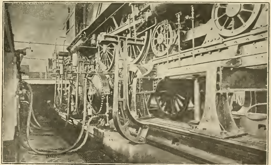
ENGINE IN POSITION FOR TEST AT THE ALTOONA PLANT.
