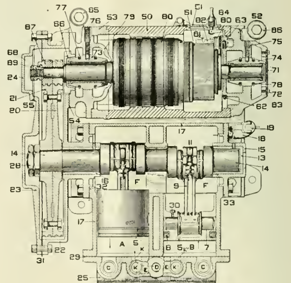
FIG. 2. PLAN OF ELECTRIC AIR PUMP.
