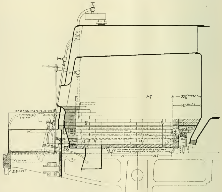
FIREBOX OF MEXICAN CENTRAL OIL BURNER.
