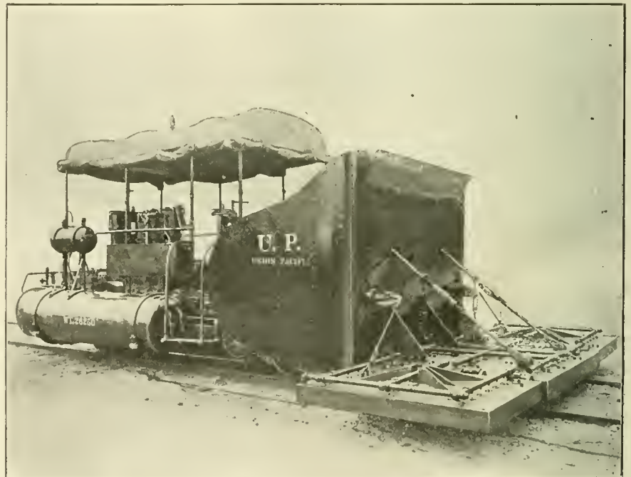
UNION PACIFIC GASOLINE WEED BURNER.
