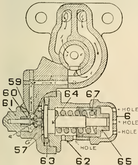
ALTERED SLIDE VALVE FEED VALVE.
