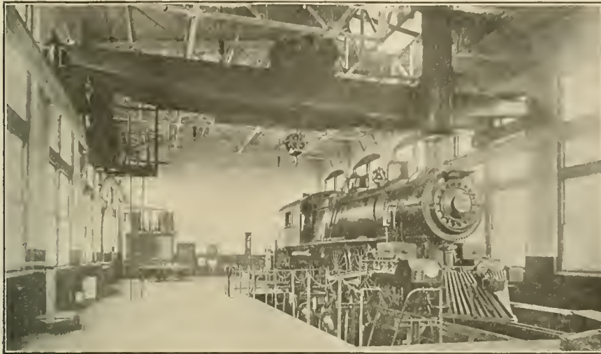
GENERAL VIEW OF PENNSYLVANIA RAILROAD TESTING PLANT.
