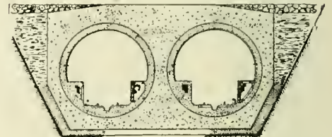
SECTION OF TUNNEL SHOWING TRENCH, FILLING, CONCRETE AND TUBES.
