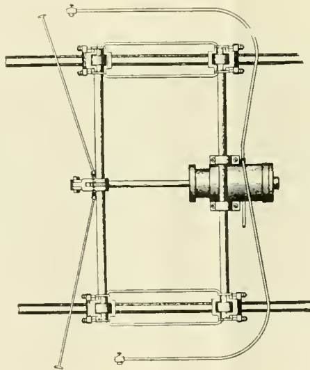
MACHINE FOR VALVE SETTING.
