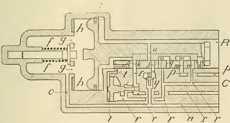
FIG. 7. GRADUATED-RELEASE LAP POSITION.
