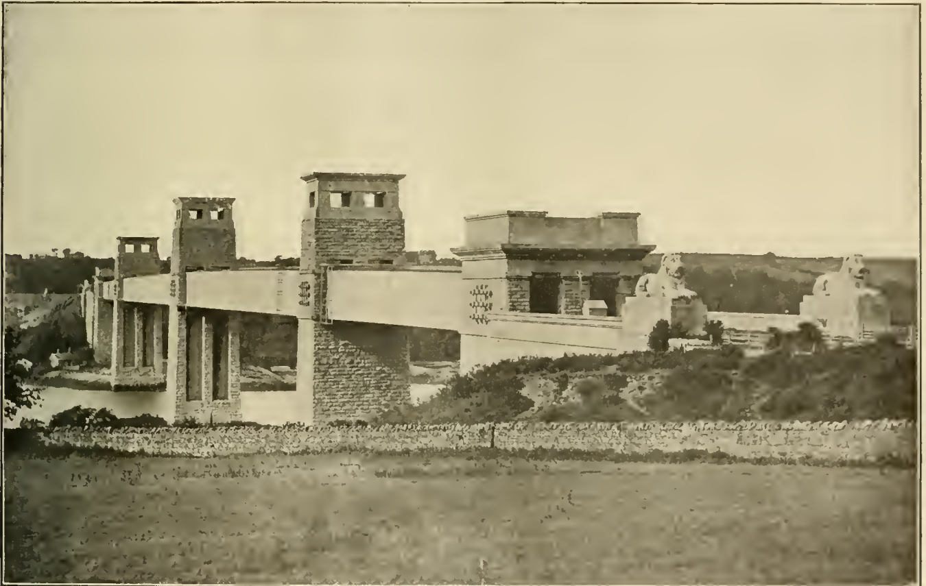
THE BRITANNIA TUBULAR BRIDGE OVER THE MENAI STRAIT.
