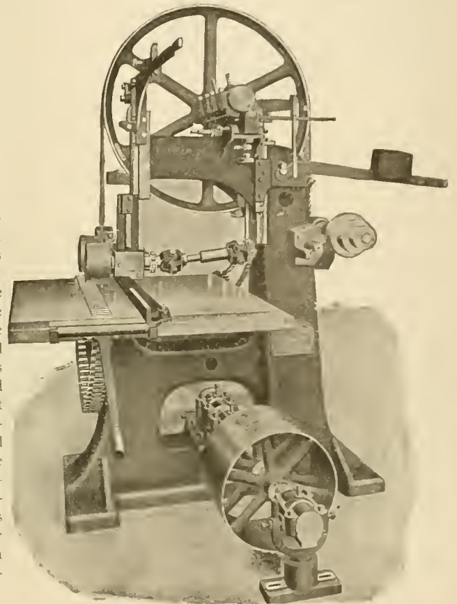
BAND RIP AND EDGING SAW.
