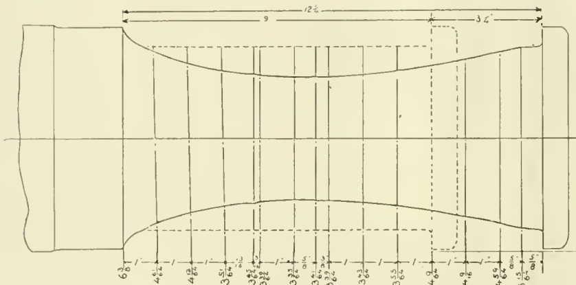
JOURNAL ELONGATED IN SERVICE.
