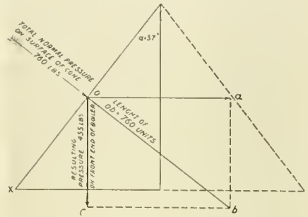
FIG. 1.—GRAPHIC PRESSURE DIAGRAM.
