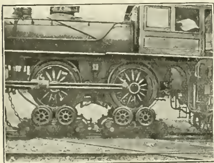
FIG. 12. HOLMAN LOCOMOTIVE.
