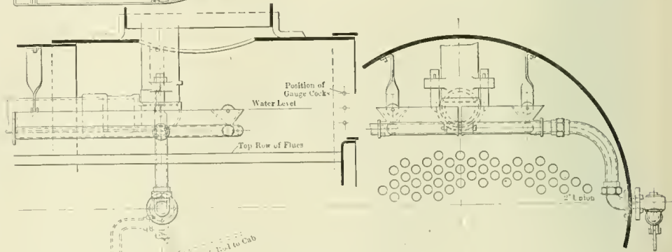
SECTION, PLAN AND END VIEW OF BARNES' BOILER SKIMMER AND BLOW-OFF VALVE.
