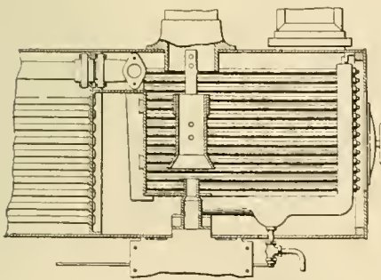
LOCOMOTIVE SUPERHEATER.
