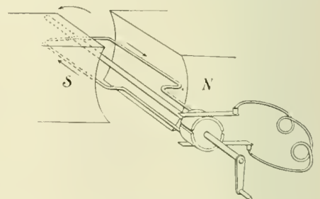
FIG. 3. SKELETON OF GENERATOR WITH COMMUTATOR.
