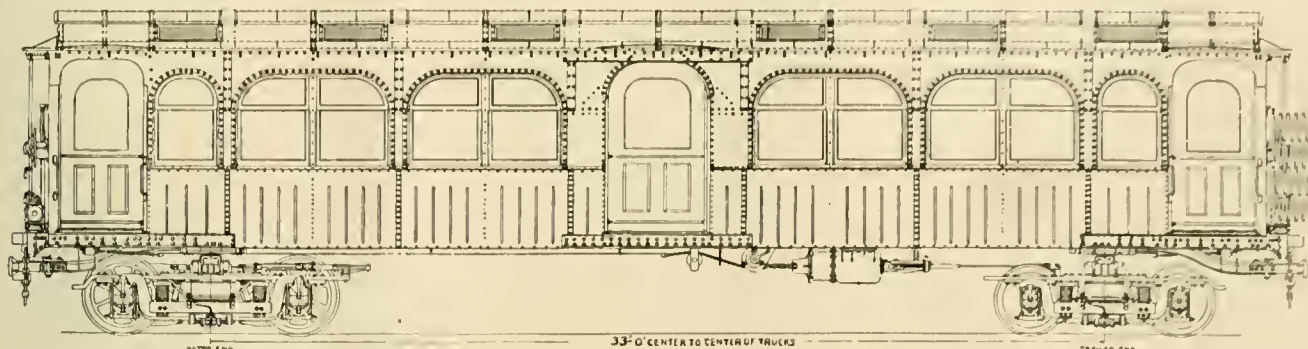
SIDE ELEVATION OF MOTOR COACH FOR THE HUDSON COMPANIES.
