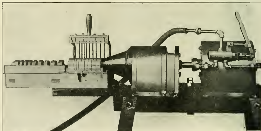
GREASE MOULDING MACHINE.
