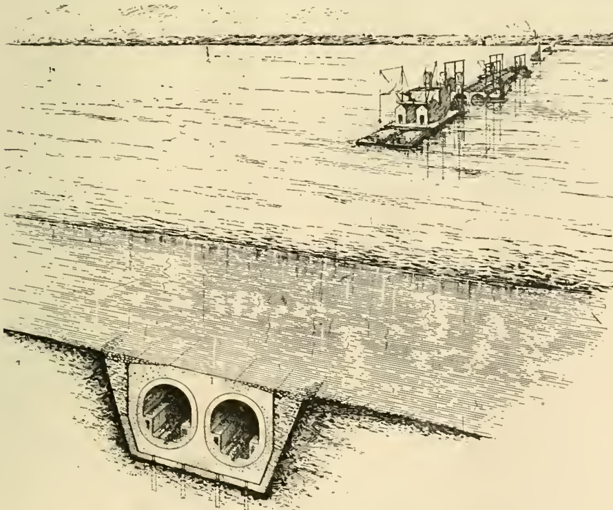
DETROIT RIVER TUNNEL, LOOKING TOWARD CANADA.
