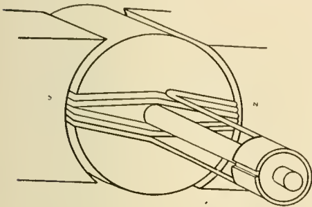
FIG. 4. SINGLE COIL DRUM ARMATURE.
