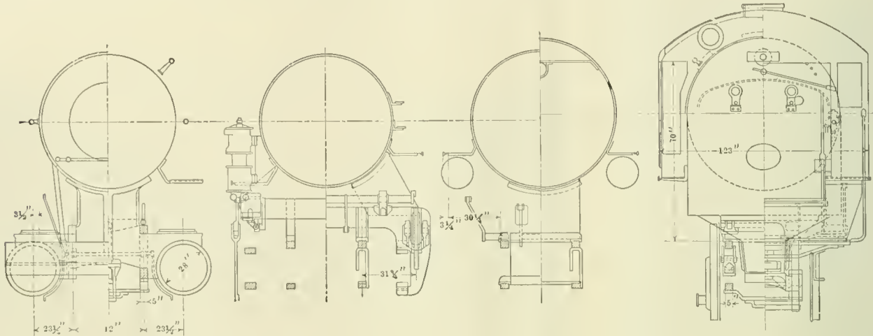
CROSS SECTIONS OF PITTSBURG, SHAWMUT & NORTHERN RAILROAD ENGINE.
