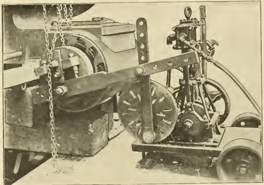
LABOR-SAVING METHOD OF GRINDING CYLINDER COVERS.
