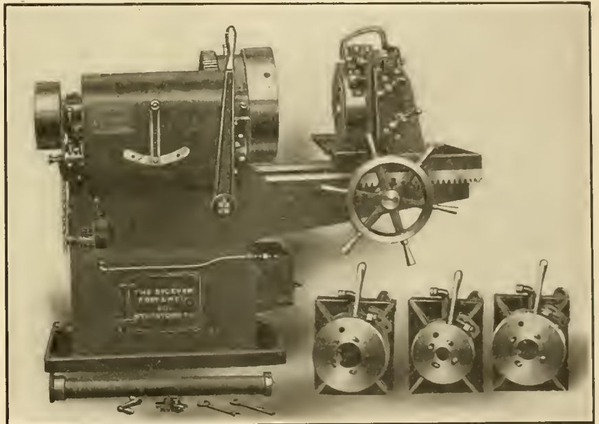
LEVER TYPE OF PIPE THREADING MACHINE.
