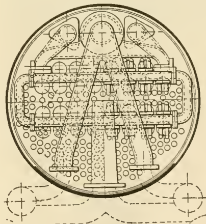
TOLTZ SUPERHEATER.
