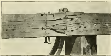
RAIL DRIVEN THROUGH PILOT BEAM.
