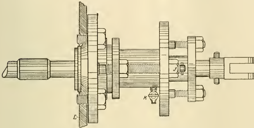
FIG. 1. STUFFINGBOX WHILE IN SERVICE.
