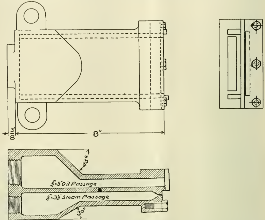
CONSTRUCTION OF THE BURNER, SHOWING OIL AND STEAM JET OPENING.
