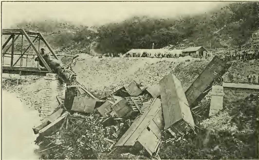
WRECKED BY ACCIDENTAL DISCHARGE OF DYNAMITE WHERE TUNNEL WAS BEING DRIVEN. (Courtesy of the Engineering Record.)
