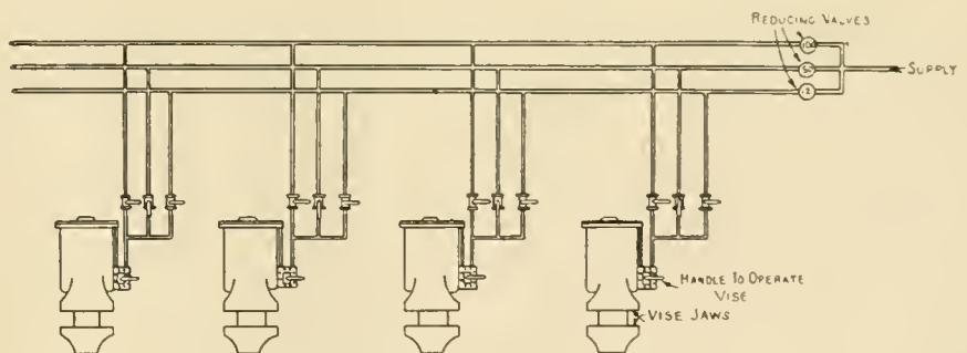
PIPING ARRANGEMENT FOR AIR OPERATED VISES.
