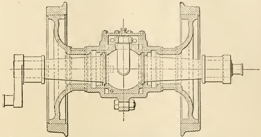
WHEELS WITH HOLLOW SLEEVE CONTAINING SOLID AXLE WITH CENTRAL BALL JOINTS FOR DRIVING; MATHERAN RAILWAY.
