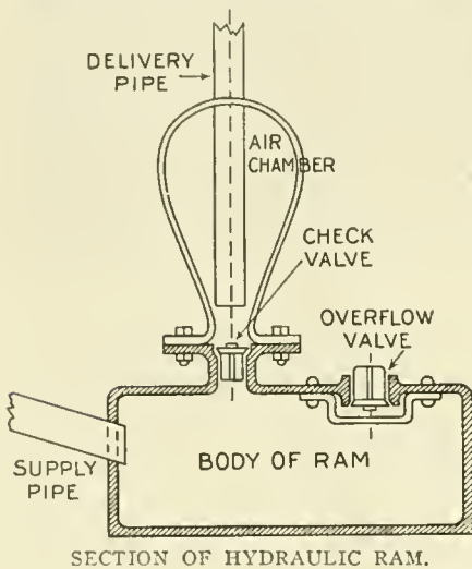
SECTION OF HYDRAULIC RAM.
