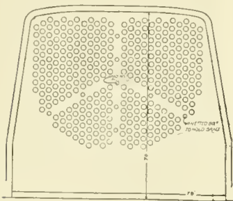
METHOD OF BRACING FLUE SHEET. BIG FOUR.
