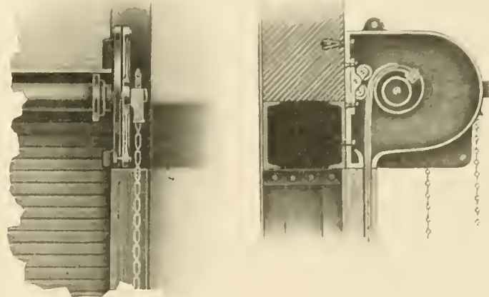
OPERATING MECHANISM AND CASE FOR ROLLED DOOR.
