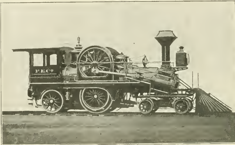
FIG. 11. FONTAINE LOCOMOTIVE.
