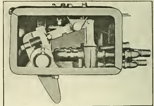
FIG. 4. ENGINE EQUIPMENT, PHILLIPS SYSTEM.
