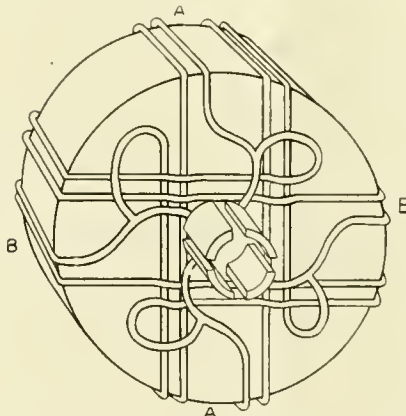
FIG. 9. FOUR COIL DRUM ARMATURE.
