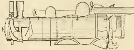
DRAFT REGULATING DEVICE.
