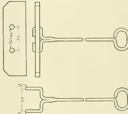
TOOT'S "STAY-TIGHT" FIRE HOE.
