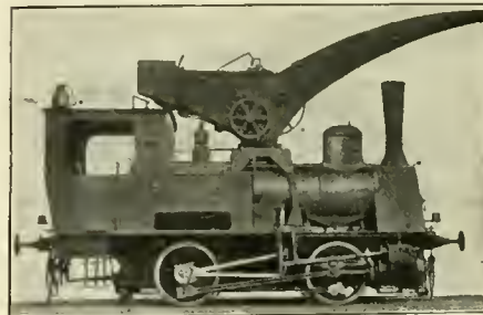
A KRUPP CRANE TANK ENGINE.
