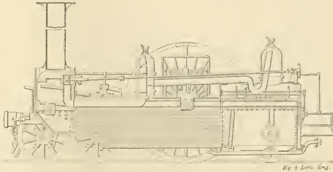
TREVITHICK'S ENGINE "CORNWALL," 1847. DRIVING AXLE CARRIED OVER BOILER TO GIVE LOW CENTRE OF GRAVITY.
