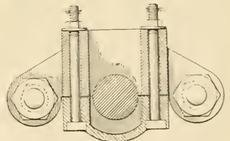
VALVE ROD CLAMP AND OILER.
