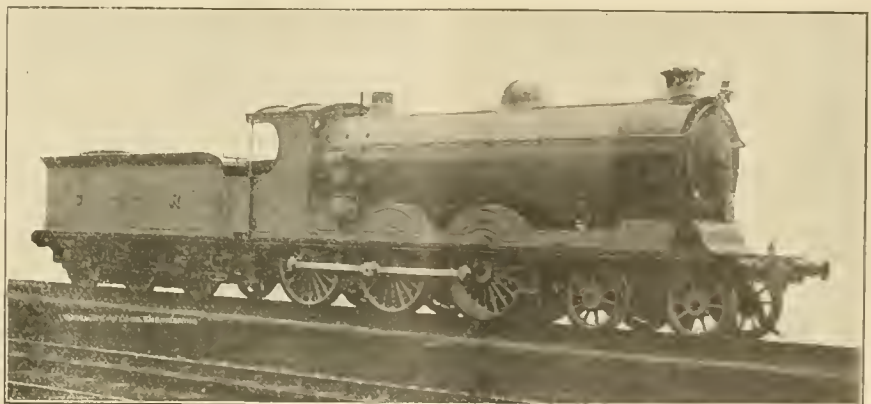
CALEDONIAN 4-6-0, ONE OF THE 908 CLASS.
