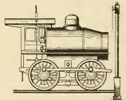
LOCOMOTIVE AUTOMATIC CONTROLLER.
