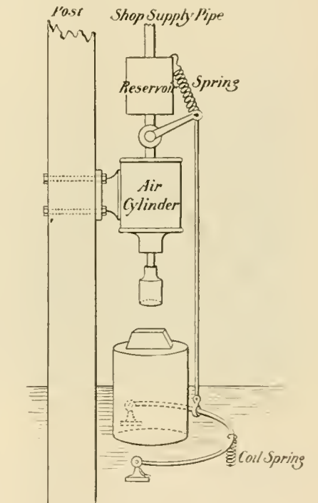
SHOP AIR HAMMER.
