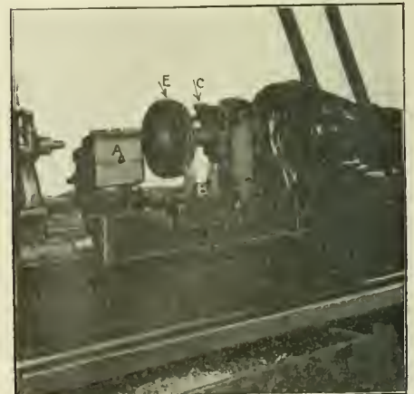
FIG. 3. GANG TOOL FOR PISTON HEADS.
