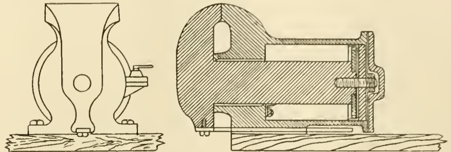
AIR OPERATED VISE FOR RAILWAY SHOPS.
