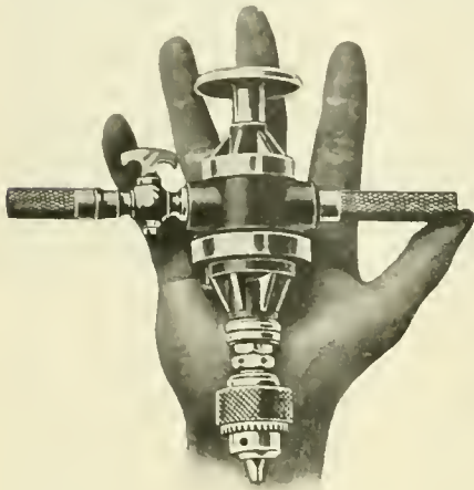
MIDGET DRILL.
