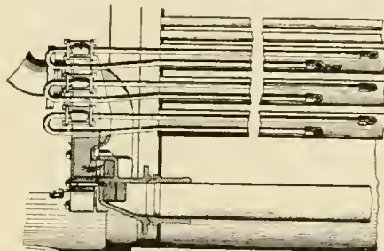
COLE SUPERHEATER.
