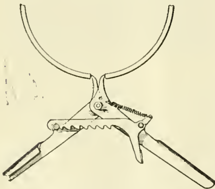
EXPANDER FOR PISTON RINGS.
