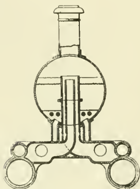
ANNULAR EXHAUST.
