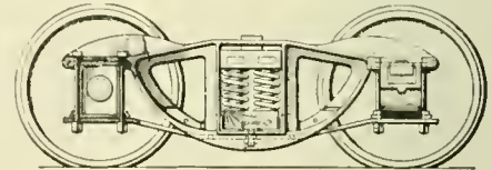
CAR TRUCK FRAMING.
