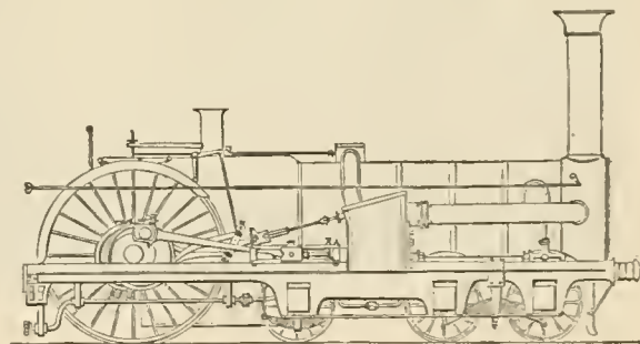
FIG. 17. CRAMPTON'S "LIVERPOOL."
