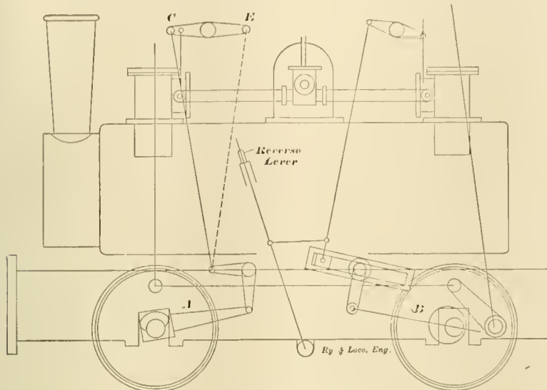
FIG. 28. ORIGINAL VALVE MOTION.
