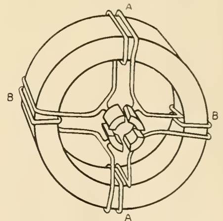
FIG. 7. FOUR COIL RING ARMATURE.
