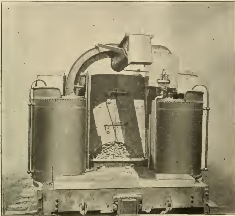
TENDER EQUIPMENT, HAYDEN STOKER.
