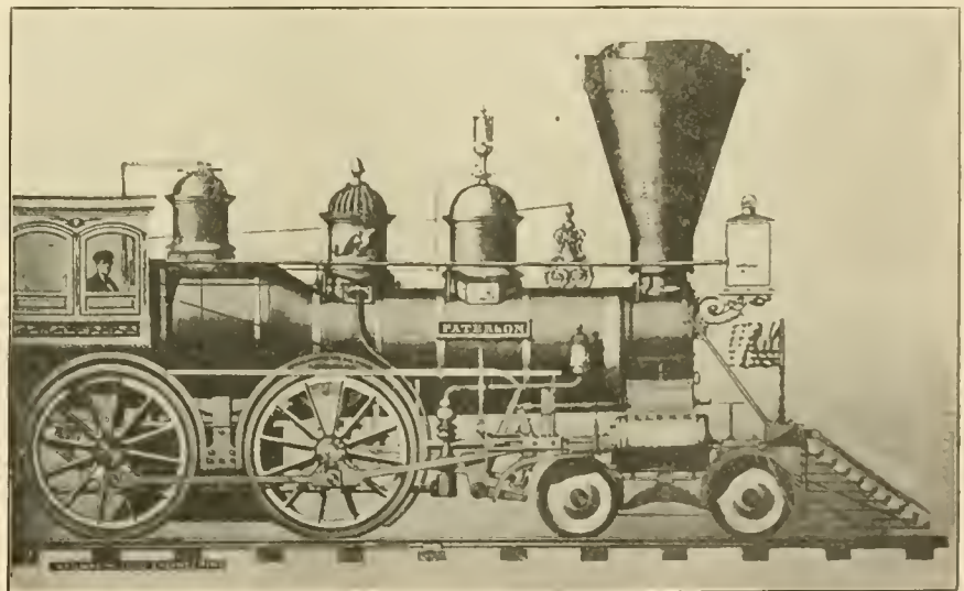
OLD ROGERS ENGINE, NEW YORK AND ERIE RAILROAD, 1855.
