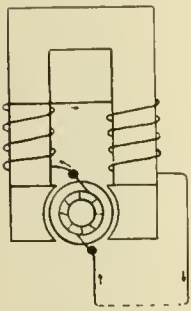
FIG. 10. SERIES WOUND.
