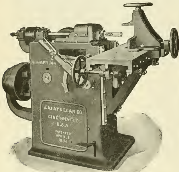
HOLLOW CHISEL MORTISING MACHINE.
