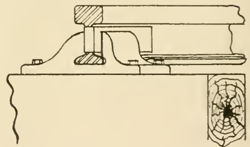
FIG. 2. PERSPECTIVE VIEW OF RAIL AND CHAIR.
