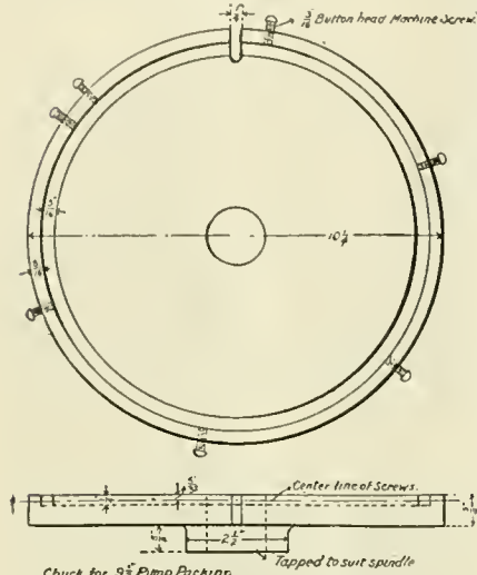
PUMP PACKING-RING CHUCK.
