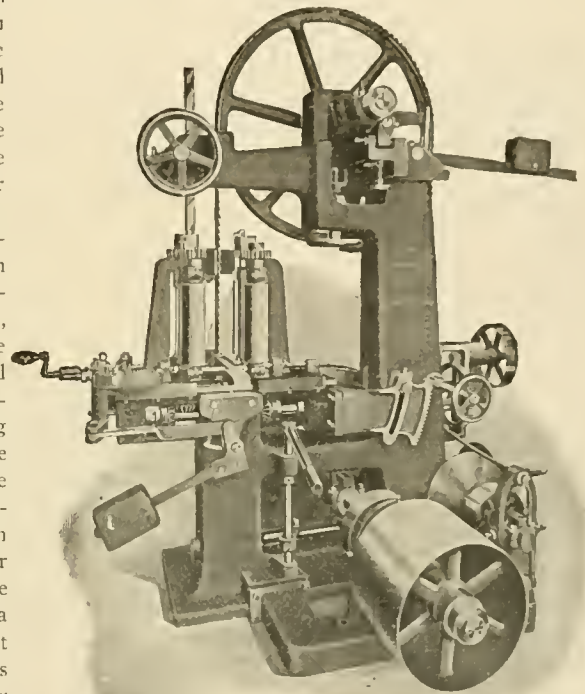
NEW BAND RESAW.
