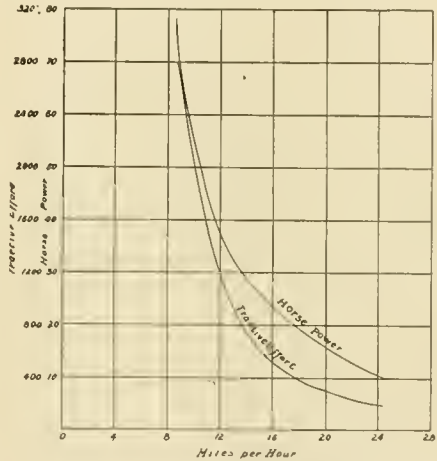
FIG. 2. TRACTIVE EFFORT AND HORSE POWER.
