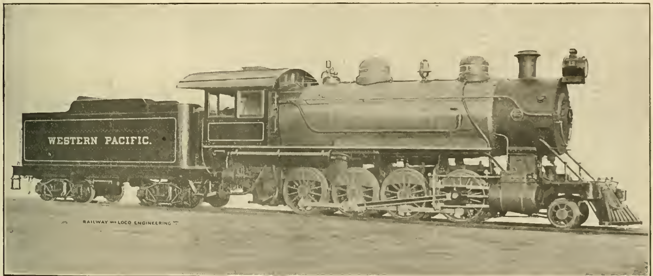
CONSOLIDATION ENGINE FOR THE WESTERN PACIFIC.
