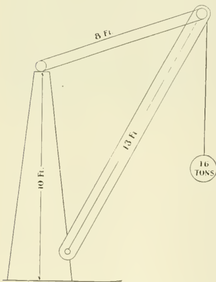
FIG. 3. WRECKING TYPE OF CRANE.
