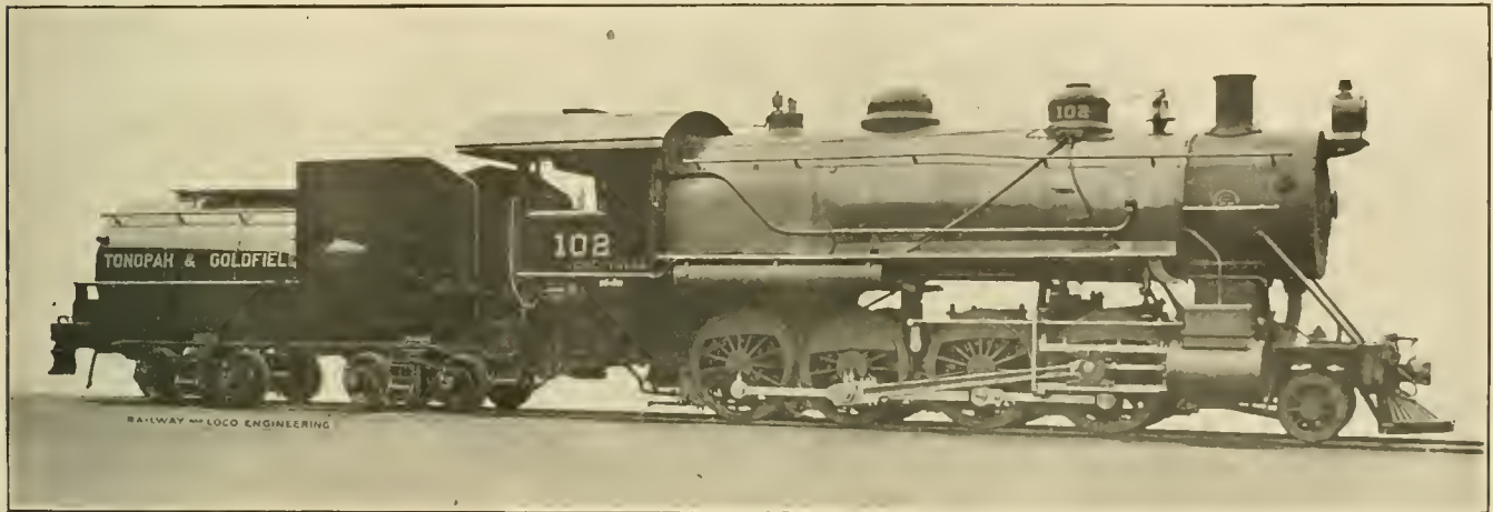
HEAVY 2-8-0 ENGINE FOR THE TONOPAH & GOLDFIELD.
