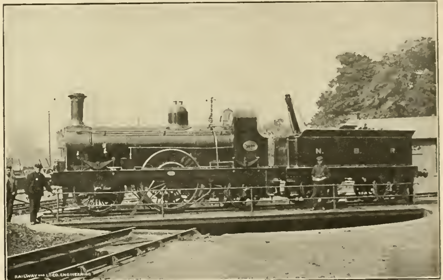
NORTH BRITISH "SINGLE," READY FOR THE ROAD.
