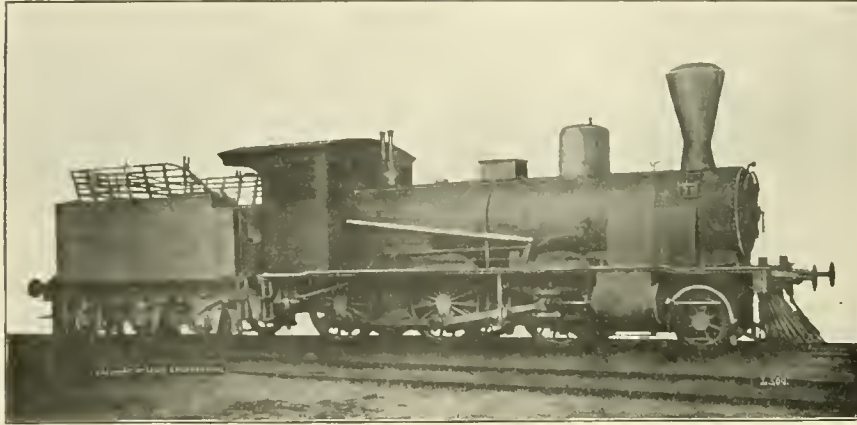
FIG. 1.—WOOD-BURNING FREIGHT ENGINE, SIAMESE STATE RAILWAY.
