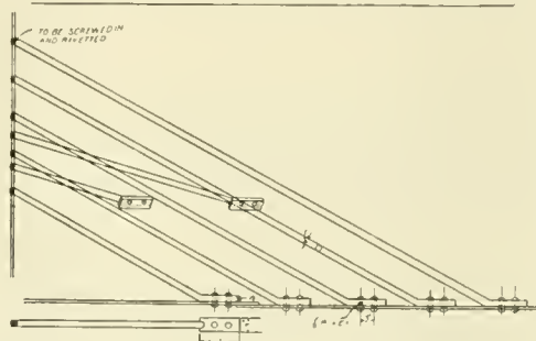
METHOD OF BRACING FLUE SHEET. BIG FOUR.
