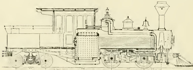
FIG. 8. MASON'S DOUBLE TRUCK LOCOMOTIVE.
