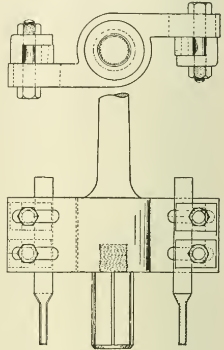
TOOL FOR CUTTING HOLES IN SIDE RODS.
