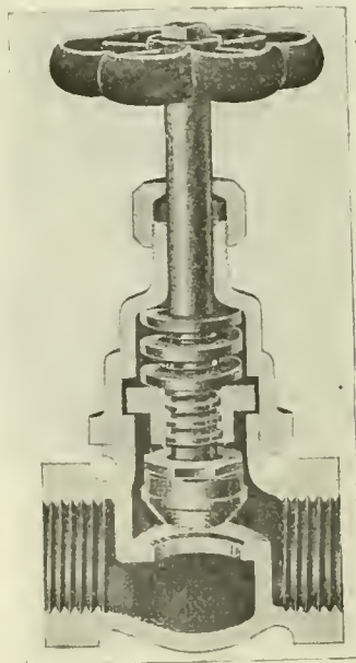
SELF-GRINDING VALVE.
