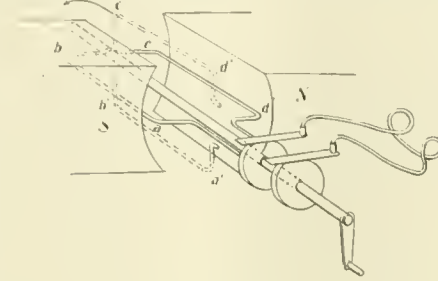
FIG. 2. GENERATOR WITH SIMPLE CONTACT RINGS.
