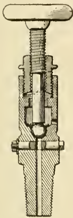
IMPROVED GAUGE-COCK.
