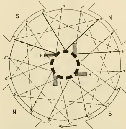
FIG. 17. MULTIPLE WOUND ARMATURE.
