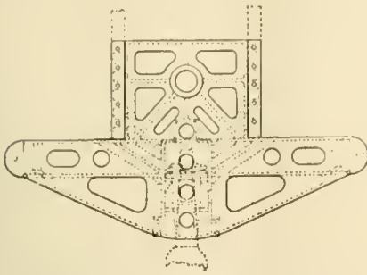
ARRANGEMENT OF BUFFER BEAM.
