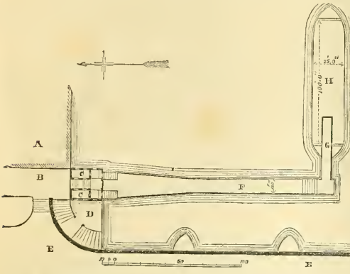
A, Houses.—B, Chatham Place.—C, Waiting Rooms.—D, Quay.—E, Blackfriars' Bridge.—F, Pier.—G, Slope.—H, Dumbly.
