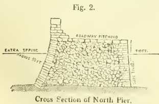
Cross Section of North Pier.
