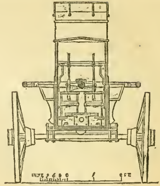
Fig. 9.—Transverse section.
