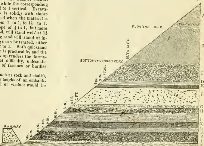
Fig. 1.—Geological section of a part of the New Cross Cutting, London and Croydon Railway.
