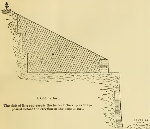
Section of the Slope in the Bilsforth Cutting, London and Birmingham Railway.
