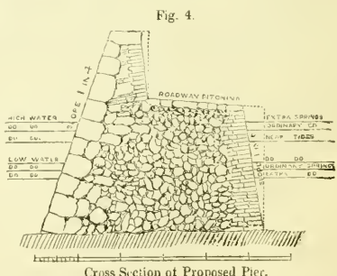
Cross Section of Proposed Pier.
