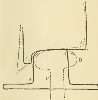
A B, Great Western rail. C D, Eastern Counties' rail. a b, flange suited for Great Western rail. c d, flange used for Eastern Counties.
