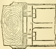
Fig. 3.—Horizontal section of the mitre-post.
