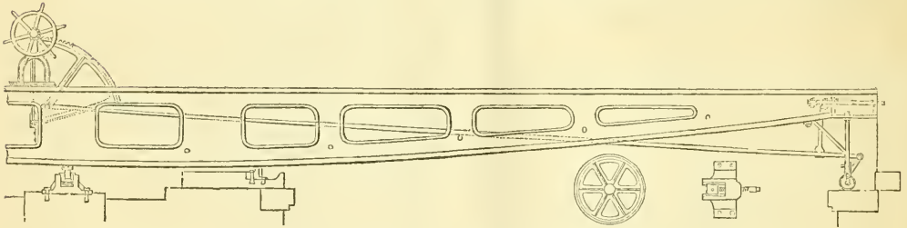
Fig. 7.—Elevation of half of the swing bridge, showing its machinery.
