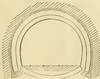
Fig. 12.—Mose Tunnel.—Transverse section.
