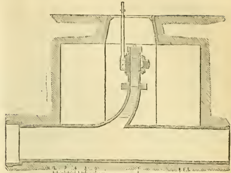
Fig. 5.—Single Fire-cock.
