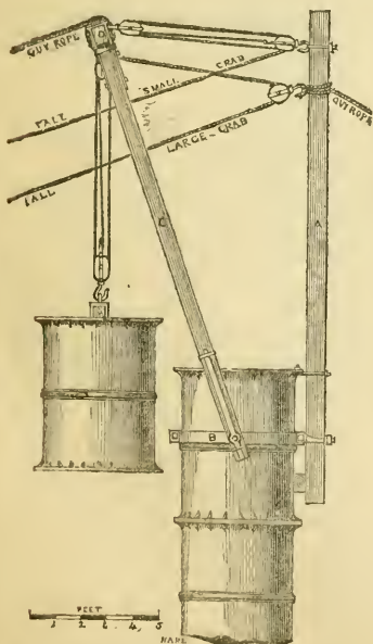
Fig. 6.—Tackle used in elevating the pipes of the 'Stand-pipe' at the East London Water-works.
