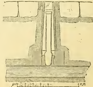
Fig. 2.—Common Fire-plug.
