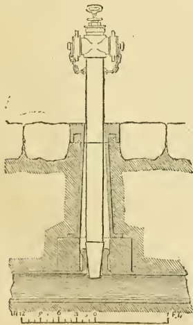
Fig. 4.—Plug, with Standcock.
