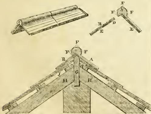
A. Ridge side with roller. B. Ditto loose, to fit under ditto. C. Pin hole in the end of the roller. D. Screw hole to fasten the under piece to the ridge. E. E. Rabbeted joints. FF. The dotted part shows the form of the square, top
