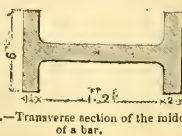
Fig. 5.—Transverse section of the middle of a bar.
