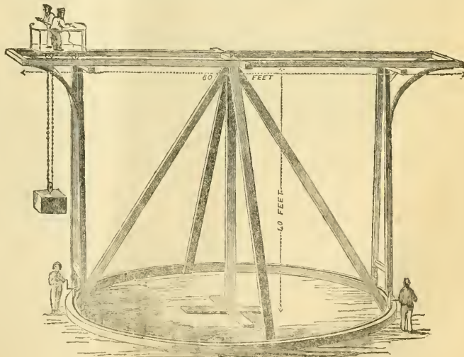
Fig. 7.—Revolving Scaffolding used at the new Houses of Parliament.
