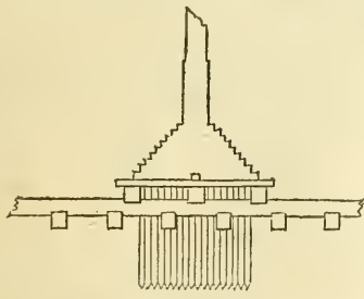
Fig. 4.—Section of the foundation for the walls of the Leyden station.
