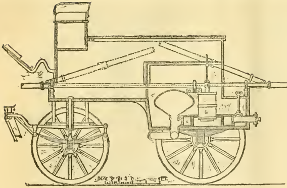
Fig. 8.—Fire Engine, used by the London Fire Brigade. Longitudinal section,—with the Levers turned up for travelling.
