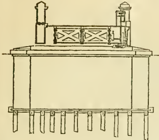
Fig. 9.—Section of the swing bridge at the centre pier.
