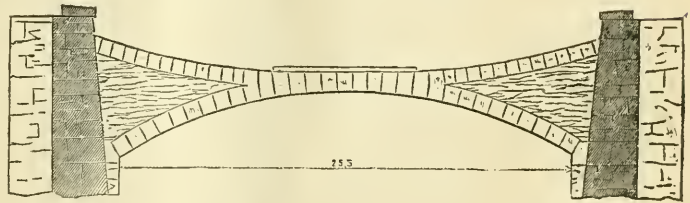
Fig. 11.—Stone Strut, Chorley Cutting. Scale.—1 inch to 8 feet.
