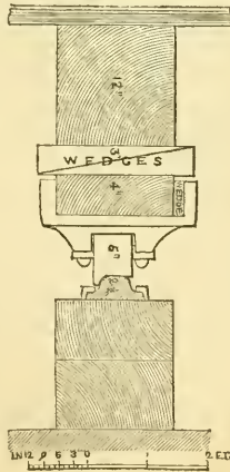
Fig. 7.—Section.
