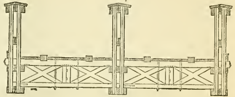
Fig. 13.—Transverse section.
