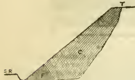
Section of Gravel counterfort, and footing, introduced into a Slip.
