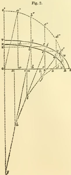
Fig. 2. Elliptical arch on the square divided into circular arcs. B S = 1.25, second arc = 1.13, third = 1.05, fourth &c. = 1.0.
