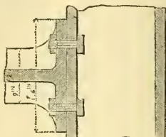
Fig. 2.—Vertical section of heel-post and bar.
