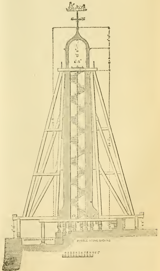
Fig. 4. Section of the Light-house, showing the Rail-balks, &c.
