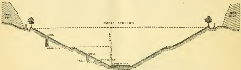
Transverse Section.—Brentwood Hill Cutting.
