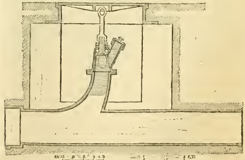
Fig. 7.—Double Fire-cock, used at the British Museum.
