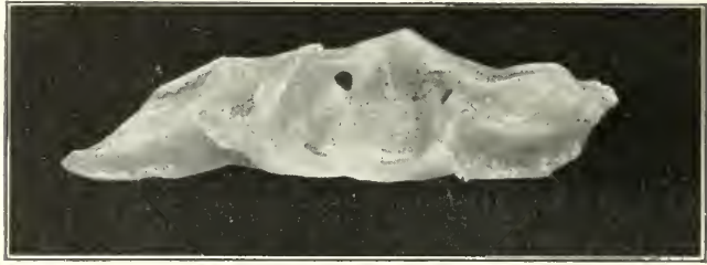
FIG. 80.—Cranium of Dogfish, cartilaginous, generalized in structure.
