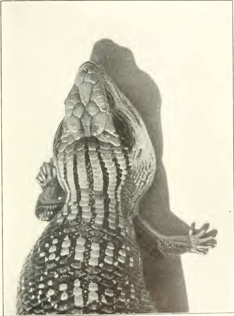
FIG. 368.—Pineal eye in Lizard
