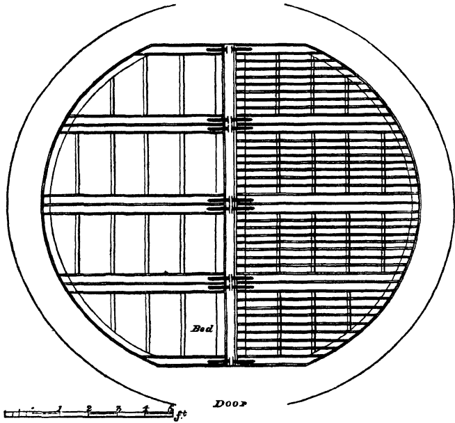
PLAN OF THE STABLES AT TEDWORTH.
