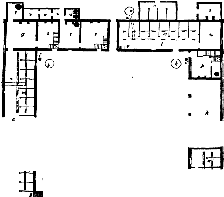
PLAN OF THE STABLES AT TEDWORTH.
