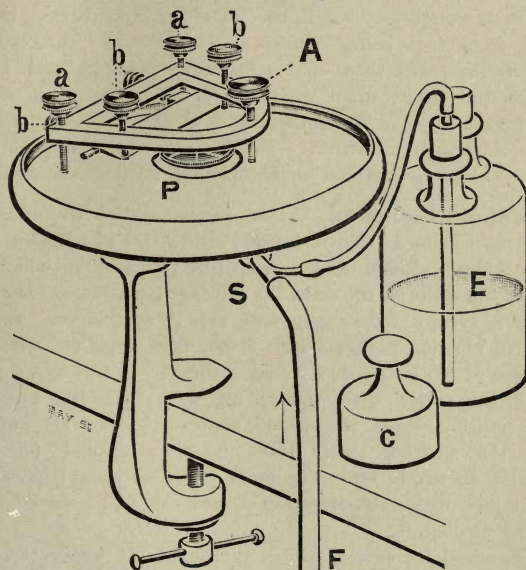
FIG. 10. Williams' Ether Freezing Microtome. (Made by Swift).
