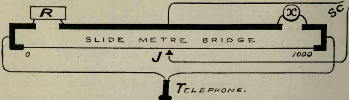
FIG. 60. Kohlrausche's Method.
