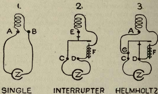
FIG. 28. Connections of the primary circuit (after Waller).
