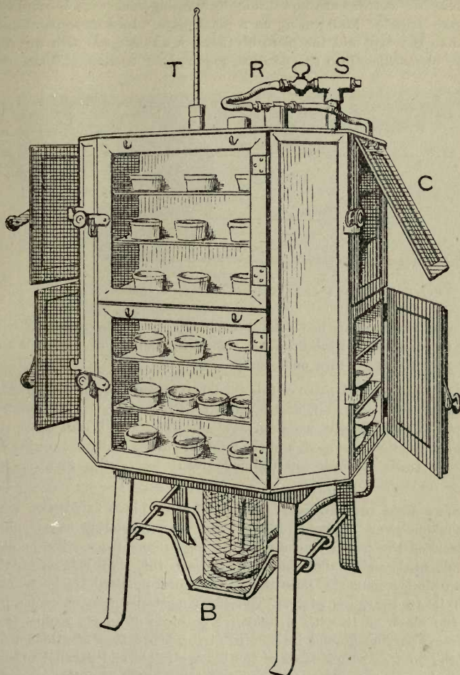
FIG. 6. Embedding Bath for the use of students in class, Yorkshire College. Around a central water cistern are six shallow closets with shelves. Each closet has a glass-panelled door, over which a non-conducting flap C hangs, removed from the front closets for clearness. R gas from S supply to regulator and thence to B, a Fletcher's safety burner; all metal piping. T thermometer. (Made to the author's directions by Messrs. Braithwaite & Co., Swinegate, Leeds.)
