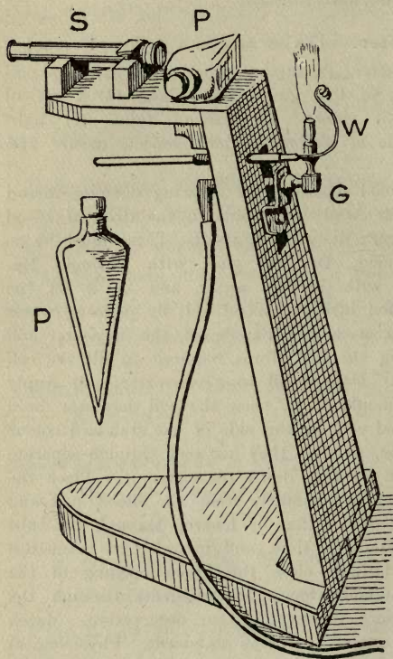
FIG. 16. Direct vision spectroscope S on a wooden stand. P wedge-shaped bottle for blood solutions. G gas. W platinum wire with a borax bead for the sodium line.
