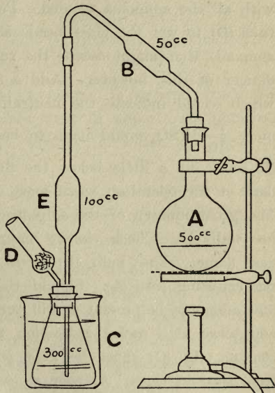
FIG. 18. Apparatus for Kjeldahl's Process. 1
