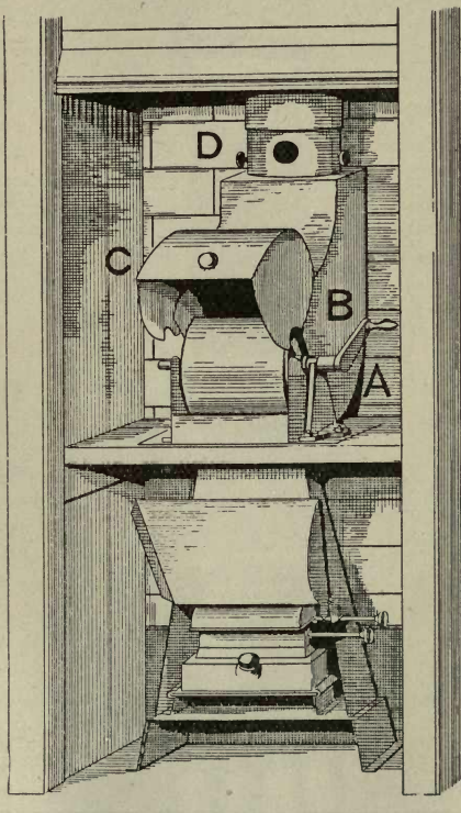
FIG. 36. Smoking chamber.
