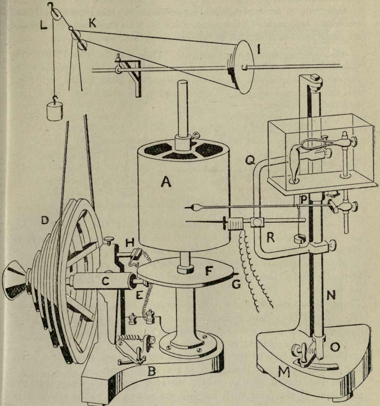
FIG. 34. Cylinder, general stand and driving cord.
