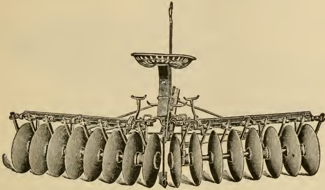
FIG. 79. Disk harrow.
