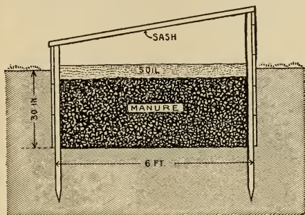
FIG. 124. A hot-bed.
