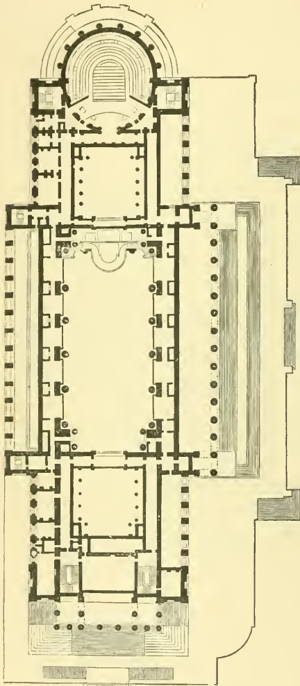
202. Plan of St. George's Hall, Liverpool. Scale 100 feet to 1 inch.
