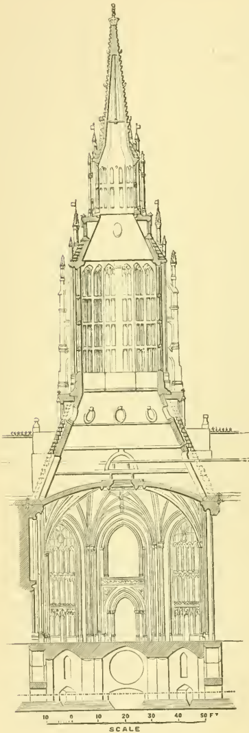
218. Section of Central Octagon, Parliament Houses. Scale 50 feet to 1 inch.
