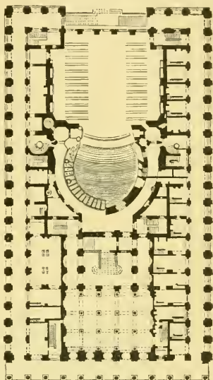
307. Plan of the Theatre at Bordeaux. Scale 100 feet to 1 inch.
