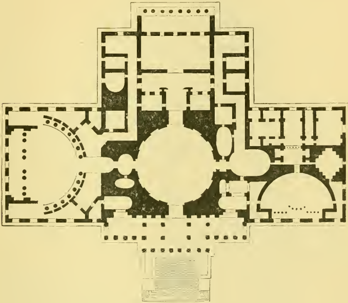
Plan of the Original Capitol at Washington. Scale 100 feet to 1 inch.
