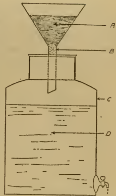
FIG. 26. — Apparatus for studying the relative rate of air movement through soils. (A) soil in funnel, (B) cotton support, (C) aspirating bottle, (D) water.
