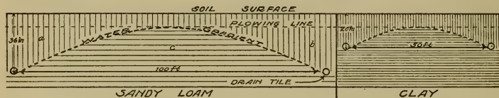
FIG. 16. — Cross sections of two soils, a sandy loam and a clay, both of which have drain tiles laid at right angles to the sections. Owing to the more rapid movement of water through the sandy loam, the tiles are laid twice as far apart as they are in the clay. They are also deeper in the former soil. The water gradient is steeper in the clay. The tiles should be sufficiently close together to keep the water table below the plowing line.
