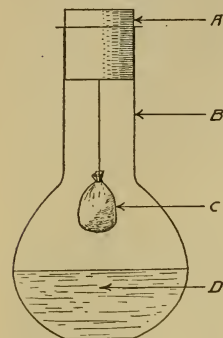
FIG. 28. — Production of carbon dioxide by germs in soil. (A) tight stopper, (B) flask containing limewater, (C) small bag containing moist soil suspended from stopper, (D) limewater.
