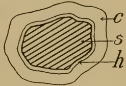
FIG. 13. — Diagrammatic drawing of soil particle and surrounding films of hygroscopic and capillary water. ( s ) soil particle, ( h ) hygroscopic film, ( c ) capillary film.
