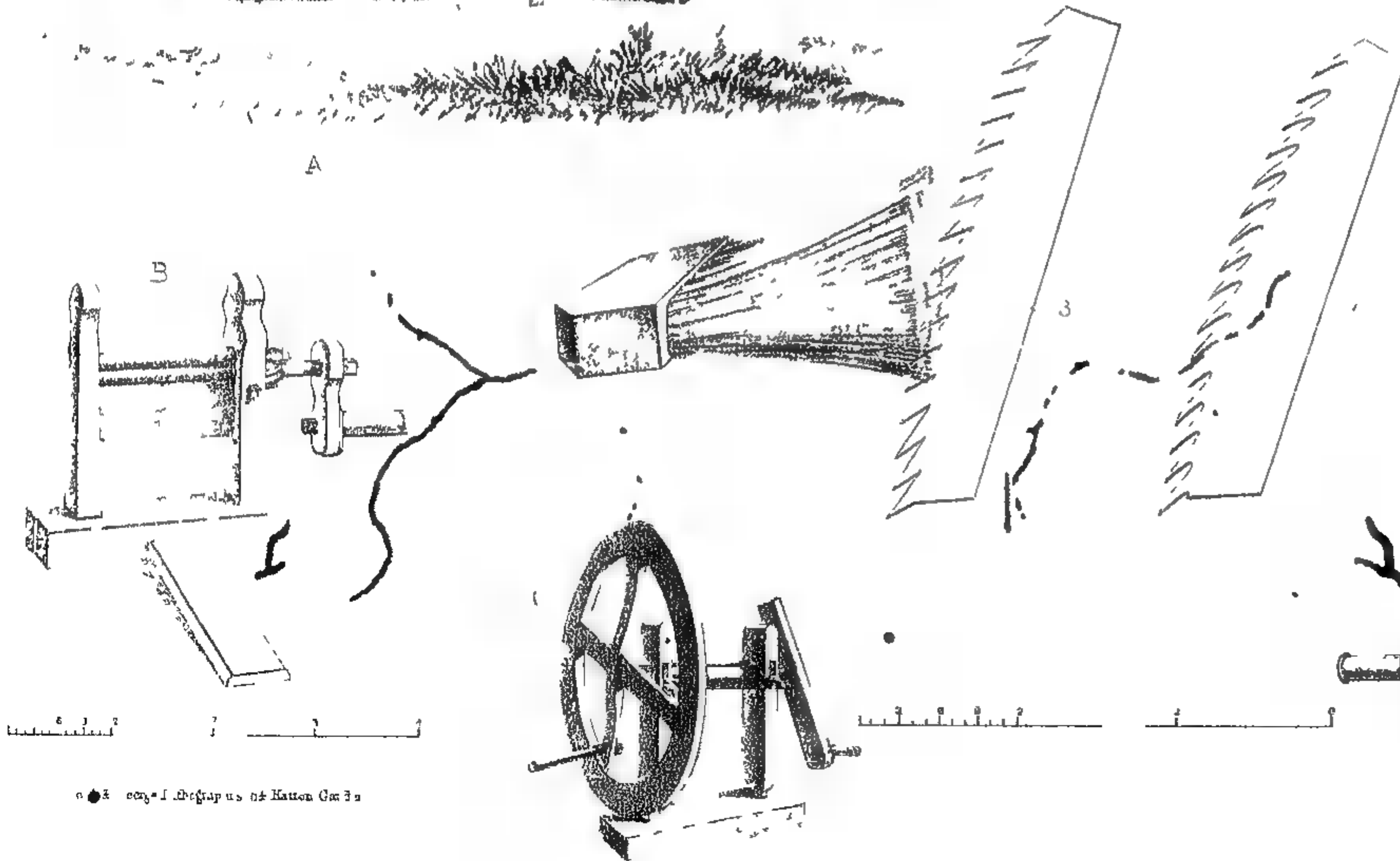
A TOOL FOR THE COMMON CHURKA C BROACH CHURKA D COMPOUND SAW AND BRUSH
