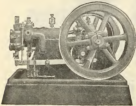
ALAMO STANDARD GASOLINE ENGINE. Type of 5-7-9 Horse Power.
