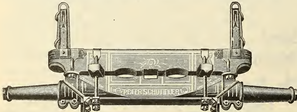
SHOWING PATENTED OSCILLATING KING BOLT AND SAND GUARDS.
