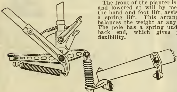
Spring Lift and Connection to Front Frame.
