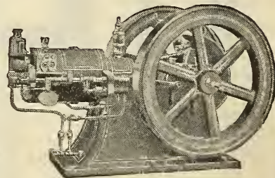
"NEW MODEL" ENGINE 2 and 3½ H. P.
