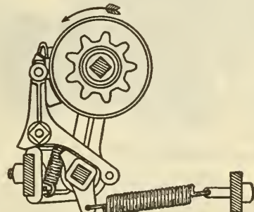
Clutch in Gear.
